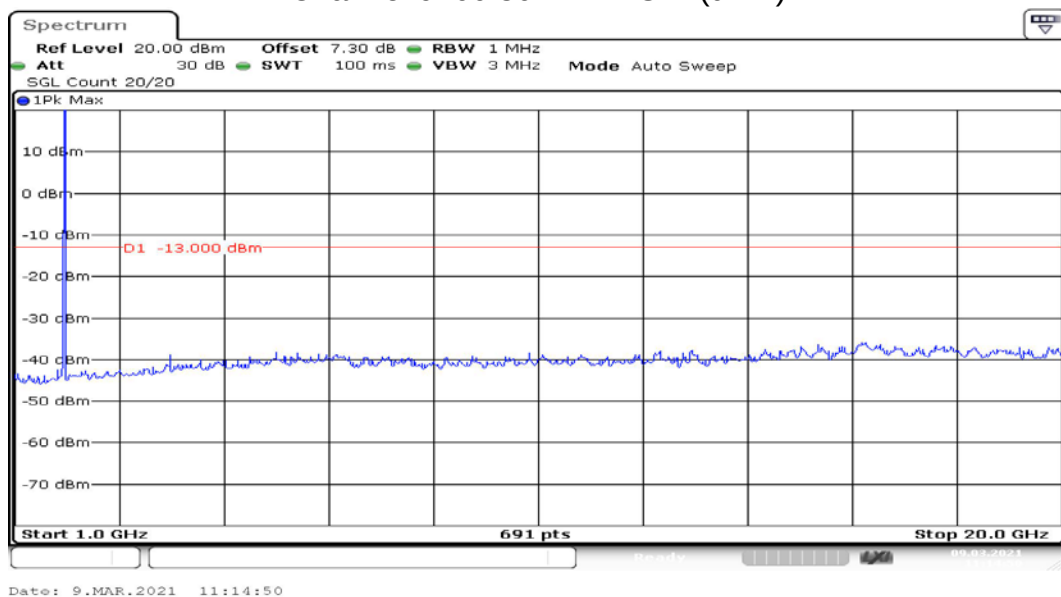
Channel 9400 1GHz~20GHz (dBm)
