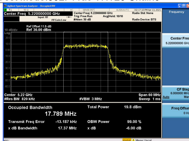
Test Mode:802. 11ac VHT20 Chain1
