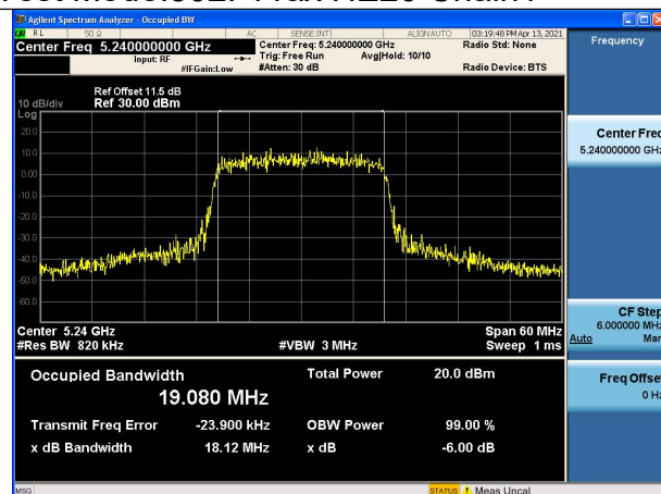
Test Mode:802. 11ax HE20 Chain1
