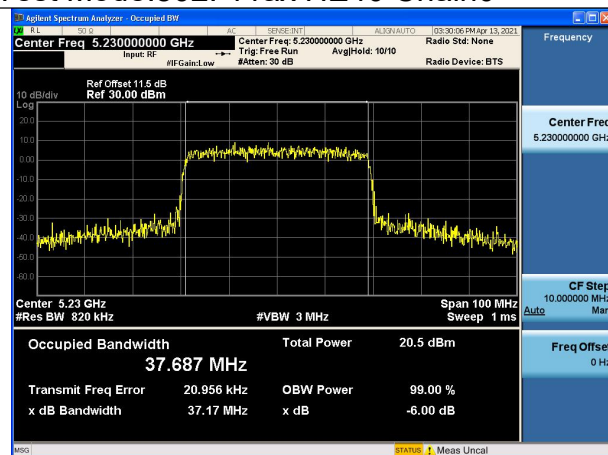
Test Mode:802. 11ax HE40 Chain0
