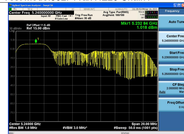
Test Mode:802. 11ax HE20 Chain1
