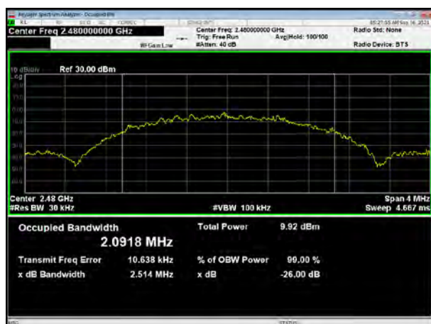
Bluetooth LE (2M) Carrier frequency (MHz): 2480
