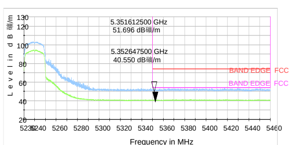
802.11ac VHT20 -Channel 48: Peak + Average
