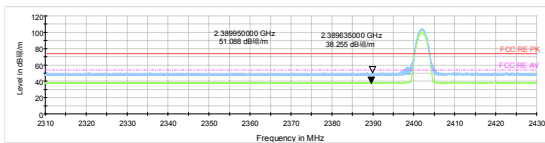
3DH5-Channel 0: Peak + Average
