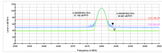
DH5-Channel 78: Peak + Average
