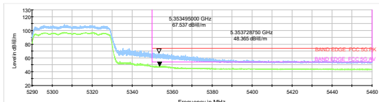
802.11ax HE40-Channel 62: Peak+Average
