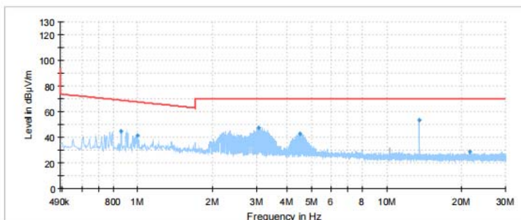
Radiates Emission from 490kHz to 30MHz
