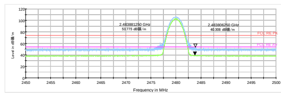
3DH5-Channel 78: Peak + Average
