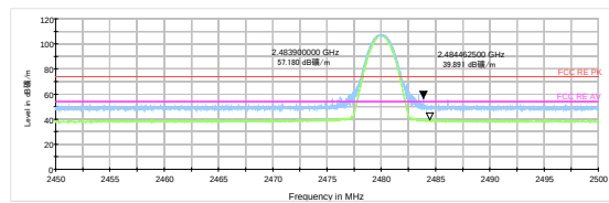
DH5-Channel 78: Peak + Average
