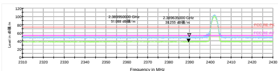
3DH5-Channel 0: Peak + Average
