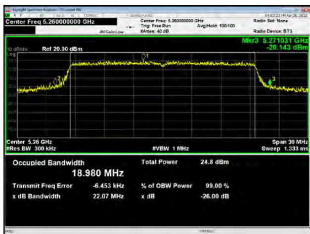
U-NII-2A, 802.11ax HE20 Carrier frequency (MHz): 5260
