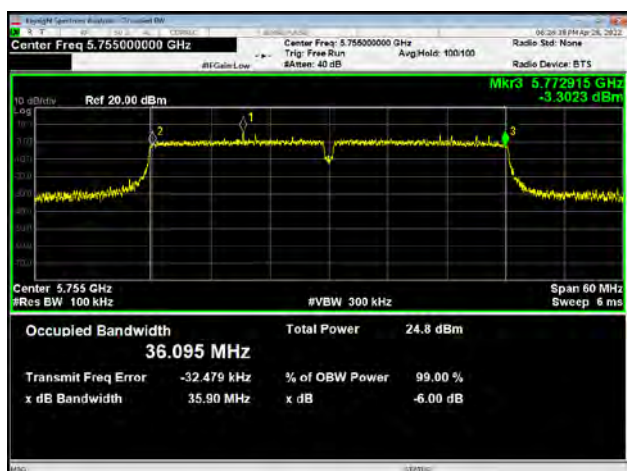
U-NII-3, 802.11ac VHT40 Carrier frequency (MHz): 5755
