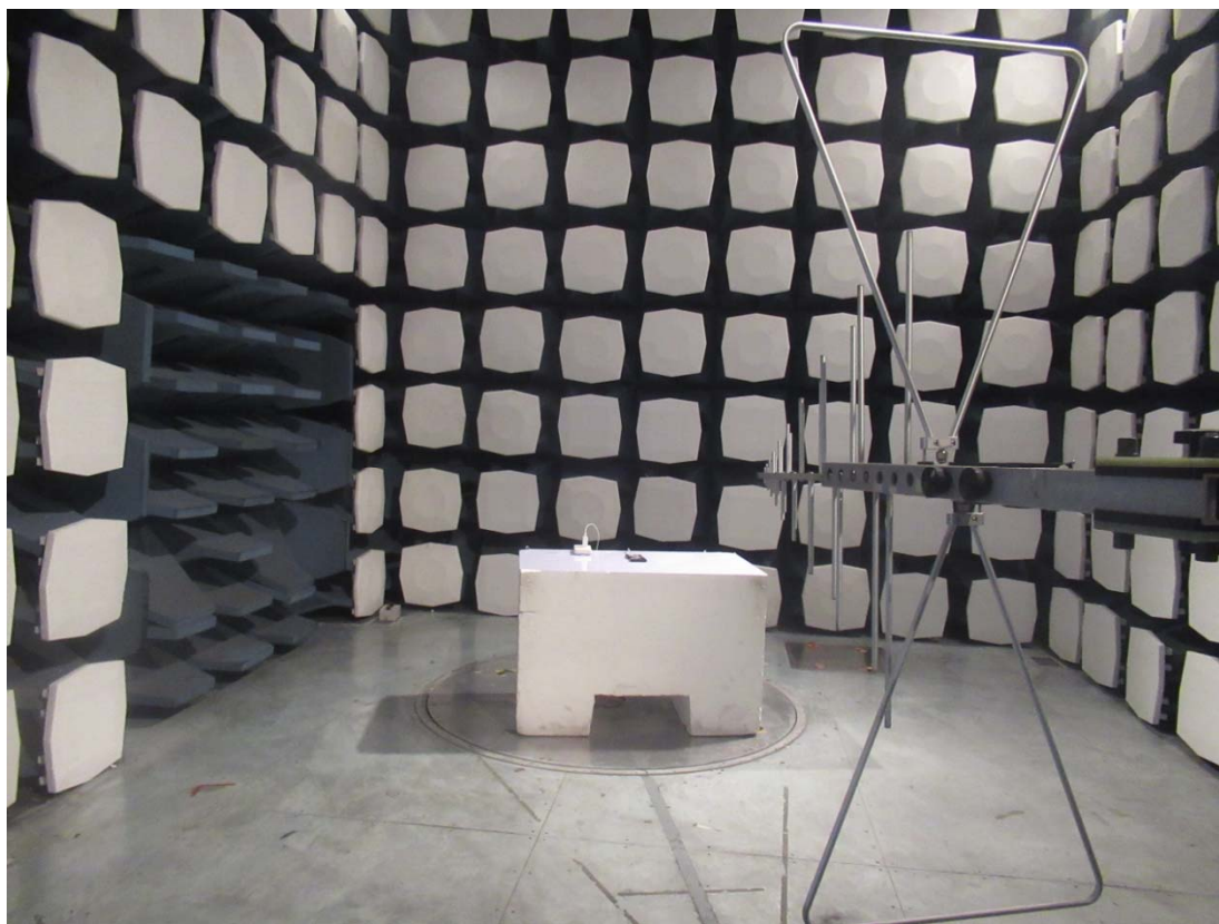
30MHz-1GHz
