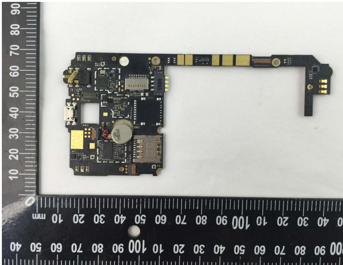
MAIN BOARD 1 FRONT VIEW
