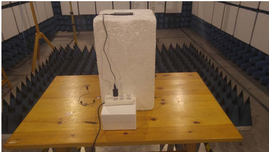
Above 1GHz-2
