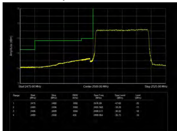
LTE Band 7 64QAM 20MHz CH-Low, 100%RB
