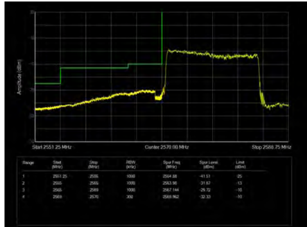
LTE Band 38 64QAM 20MHz CH-Low, 1 RB
