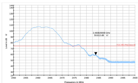
802.11b-Channel 11 Peak
