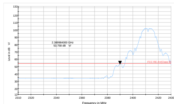
802.11b-Channel 1 Average
