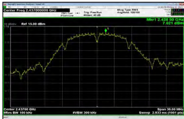
802.11b, Channel No.: 6
