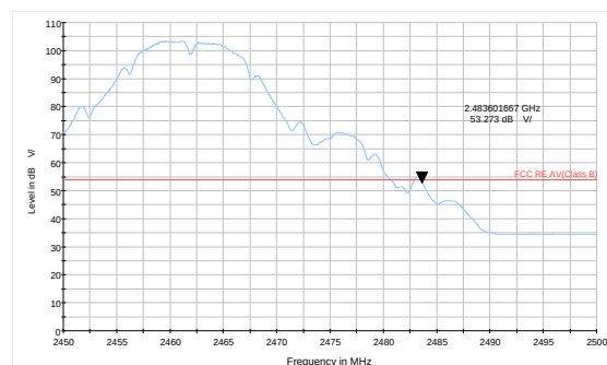
802.11b-Channel 11 Average
