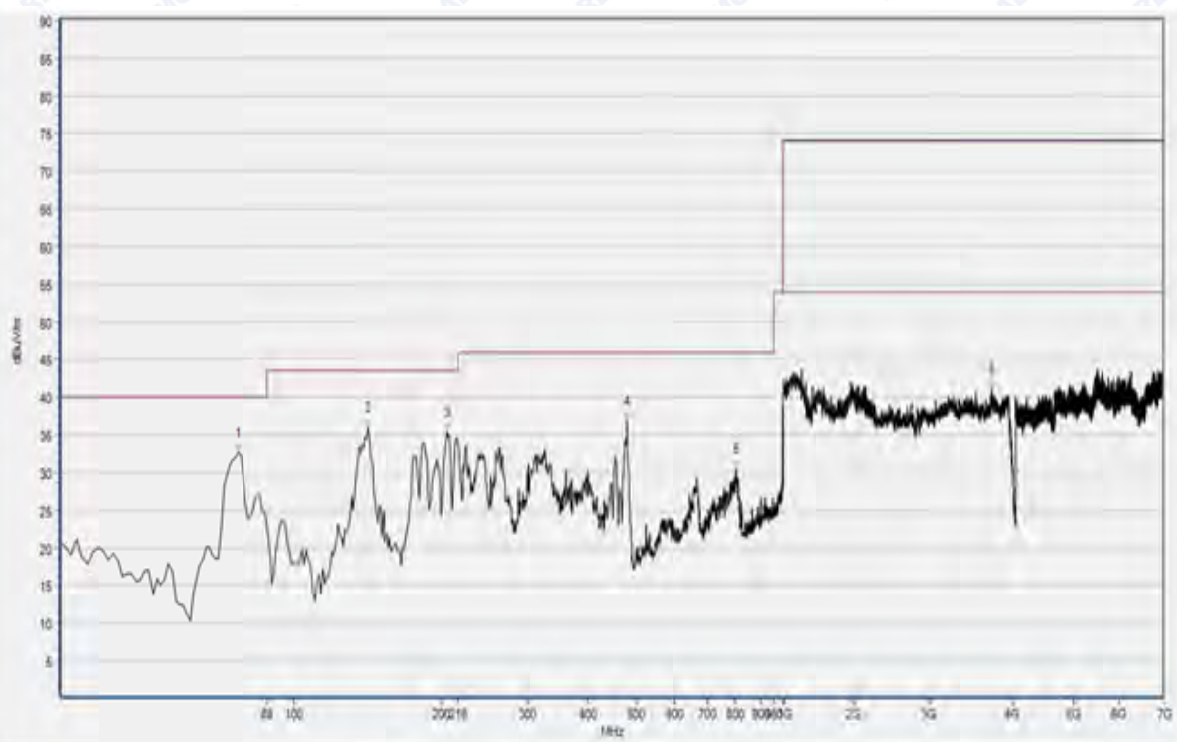
(Plot B: 30MHz – 7GHz, Test Antenna Horizontal)
