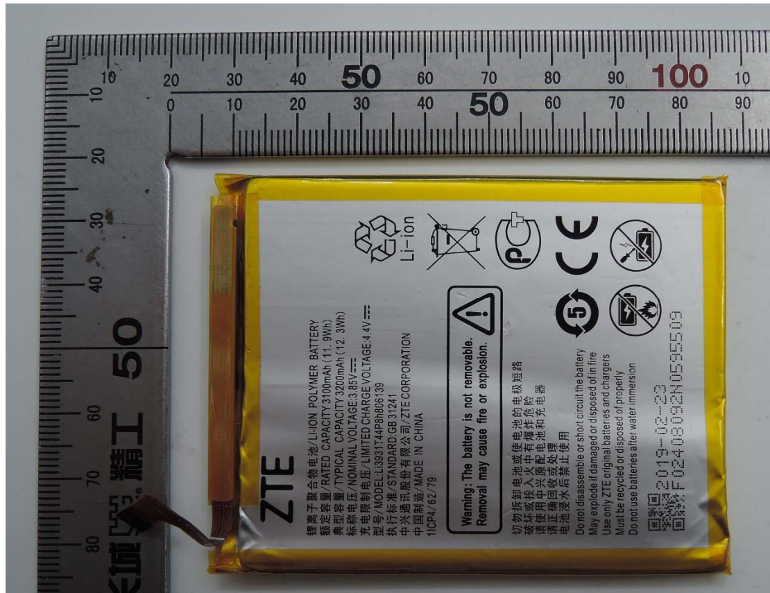
The battery view(Zhongshan Tianmao Battery Co., Ltd.)
