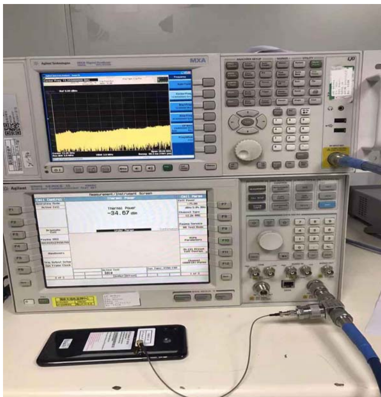
'RF Conducted Test setup (GSM/WCDMA)
