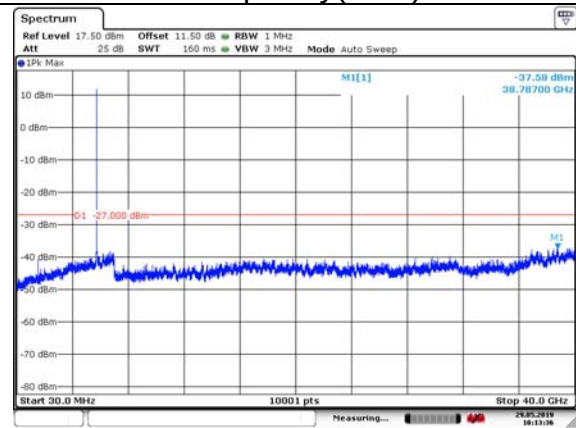
802.11a (SISO Ant2) Carrier frequency(MHz):5745
