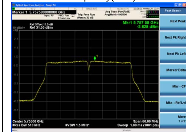
802.11n HT40 Carrier frequency(MHz):5755
