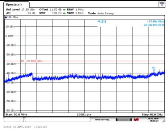
802.11n HT20 (MIMO Ant2) Carrier frequency(MHz):5745
