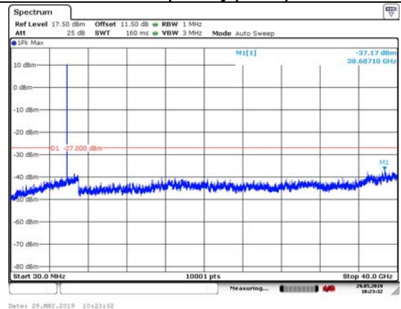
802.11n HT20 (MIMO Ant2) Carrier frequency(MHz):5825
