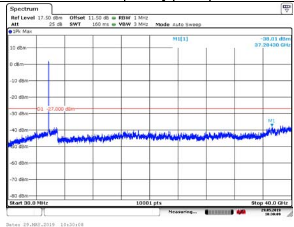
802.11ac HT80 (MIMO Ant2) Carrier frequency(MHz):5775
