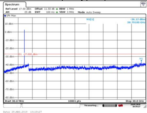
802.11ac HT80 (SISO Ant2) Carrier frequency(MHz):5775
