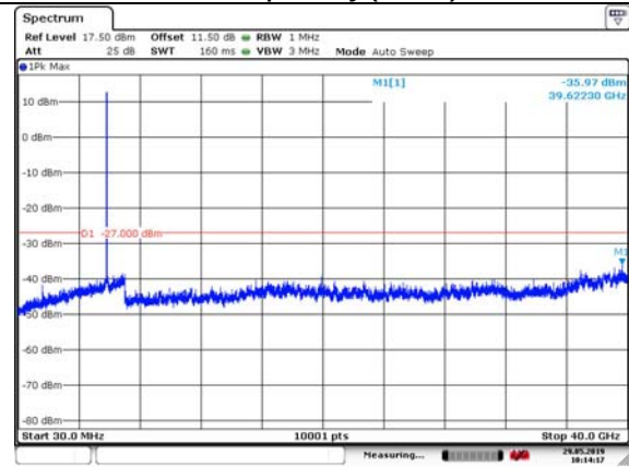
802.11a (SISO Ant2) Carrier frequency(MHz):5825
