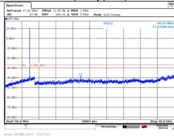
802.11n HT20 (SISO Ant2) Carrier frequency(MHz):5825
