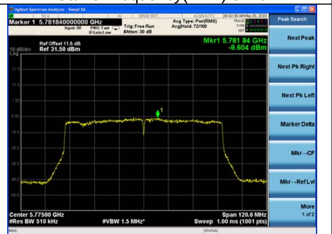
802.11ac HT80 (MIMO Ant2) Carrier frequency(MHz):5775
