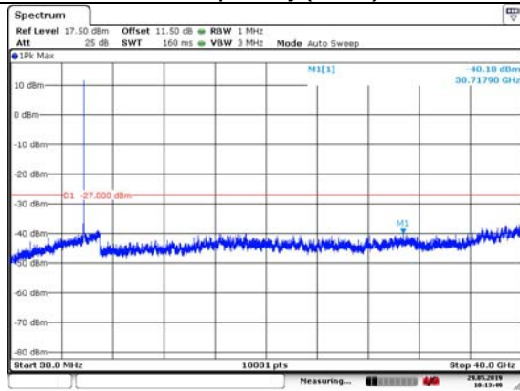
802.11a (SISO Ant2) Carrier frequency(MHz):5785
