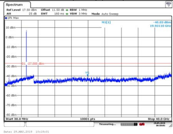
802.11n HT40 (SISO Ant2) Carrier frequency(MHz):5795
