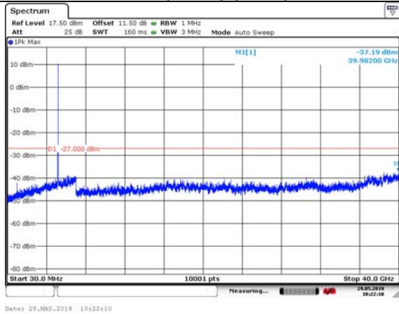
802.11n HT20 (MIMO Ant2) Carrier frequency(MHz):5240
