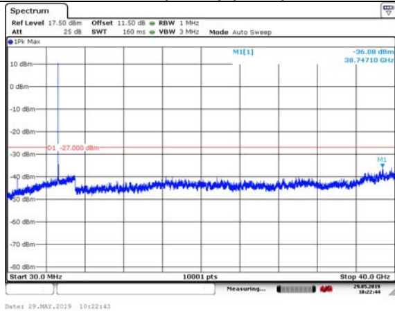
802.11n HT20 (MIMO Ant2) Carrier frequency(MHz):5785
