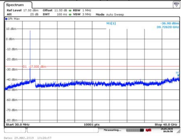
802.11n HT40 (MIMO Ant2) Carrier frequency(MHz):5230
