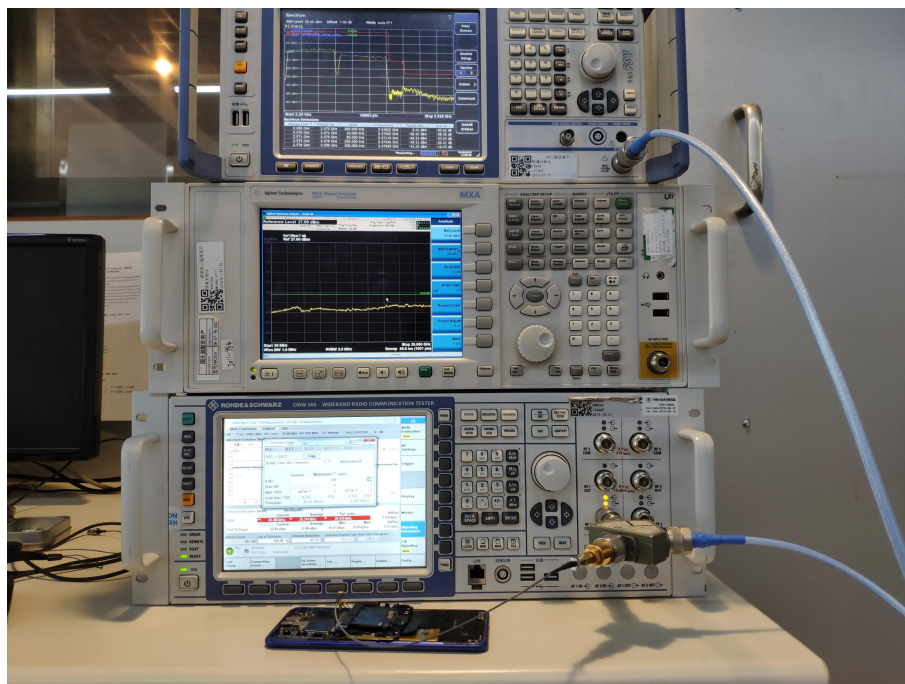
RF Conducted Test setup (LTE CA)
