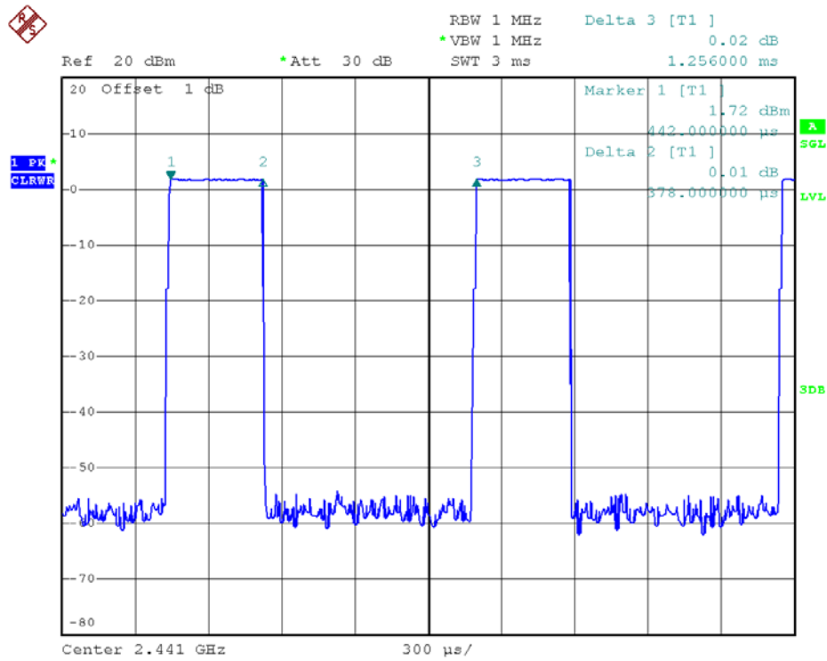
39 Channel @ DH1
