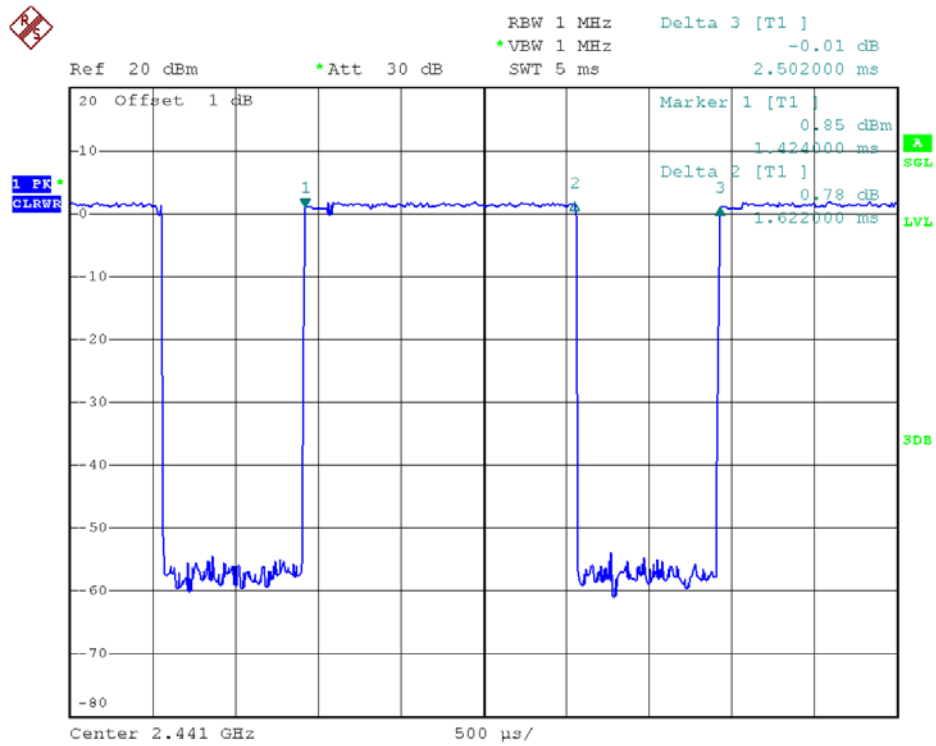
39 Channel @ 2DH3
