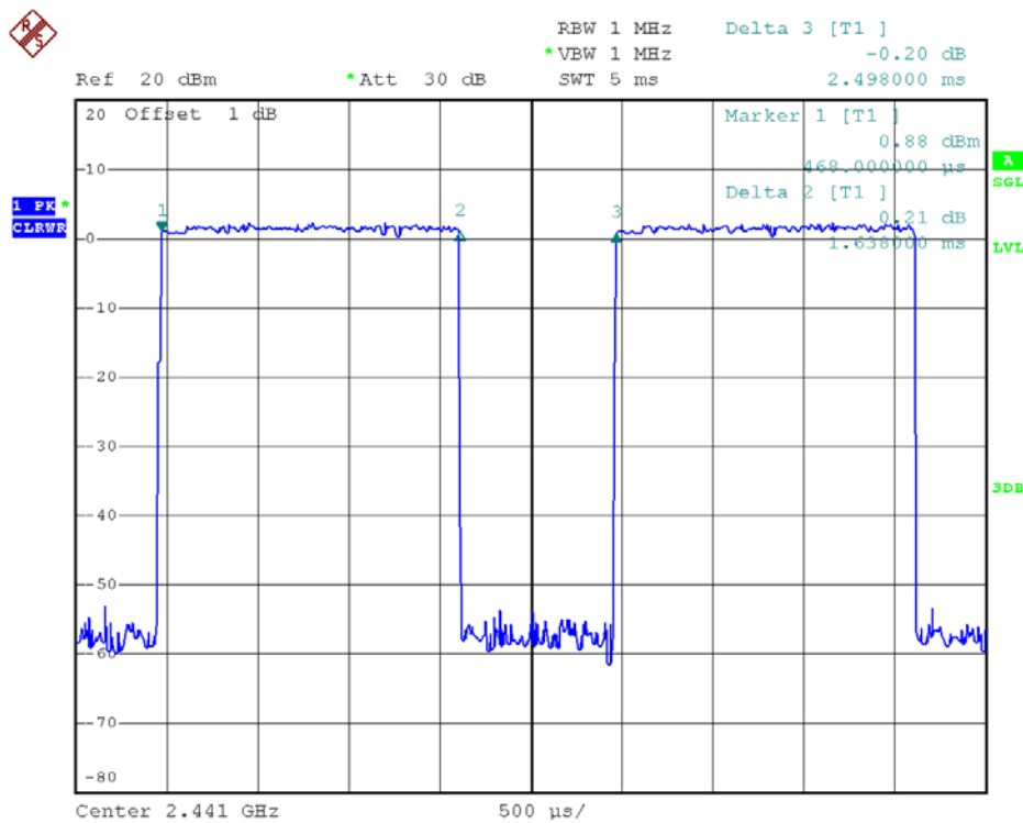
39 Channel @ 3DH3
