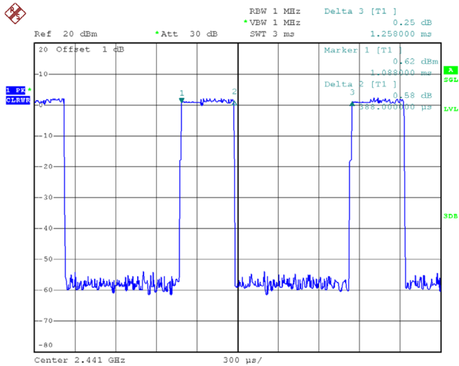
39 Channel @ 3DH1
