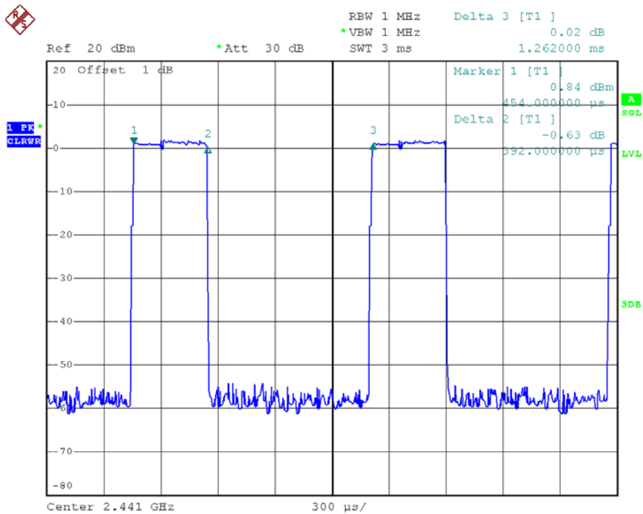
39 Channel @ 2DH1
