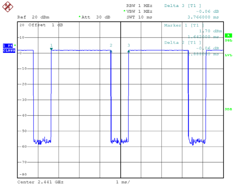
39 Channel @ DH5
