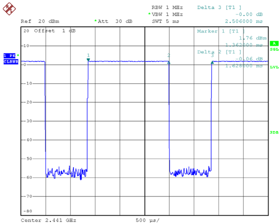
39 Channel @ DH3
