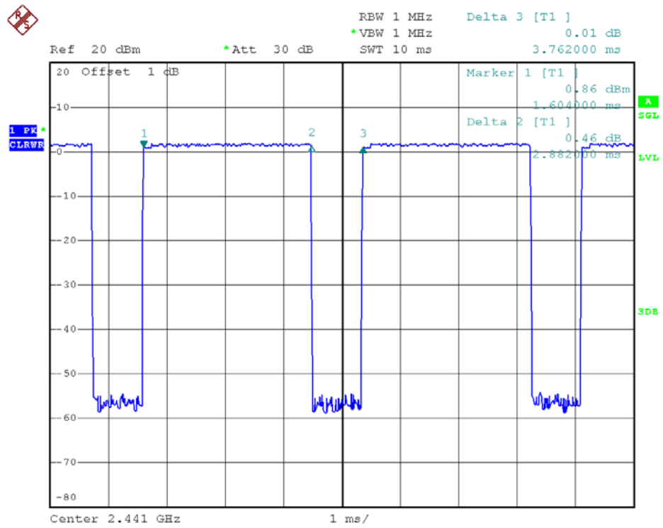
39 Channel @ 2DH5
