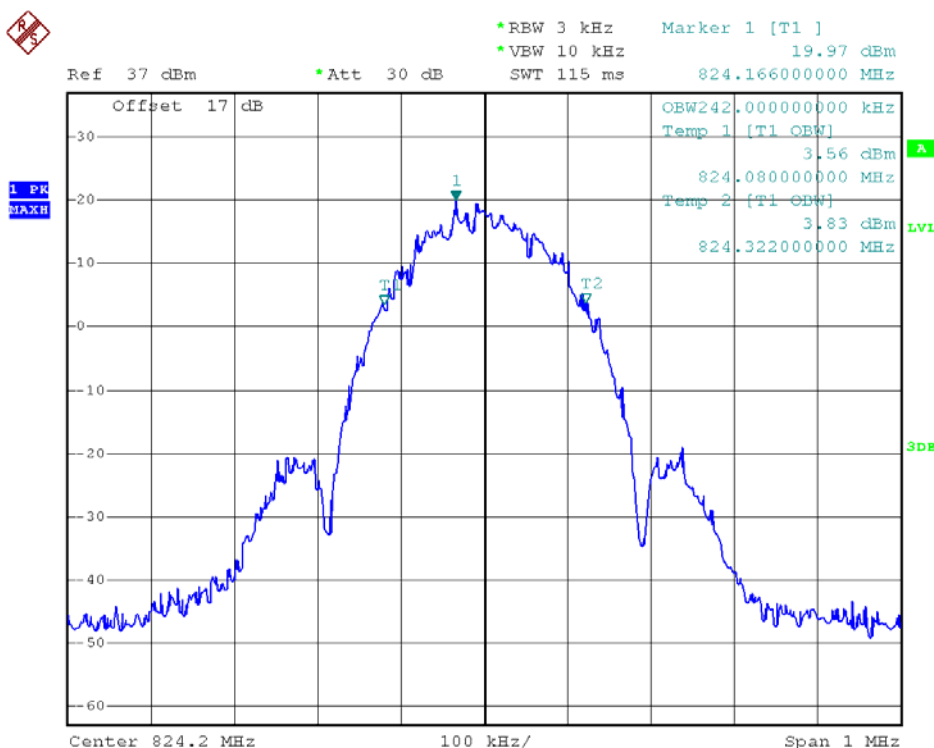
(Plot C2: EDGE 850MHz Channel = 128 99% Occupied Bandwidth)
