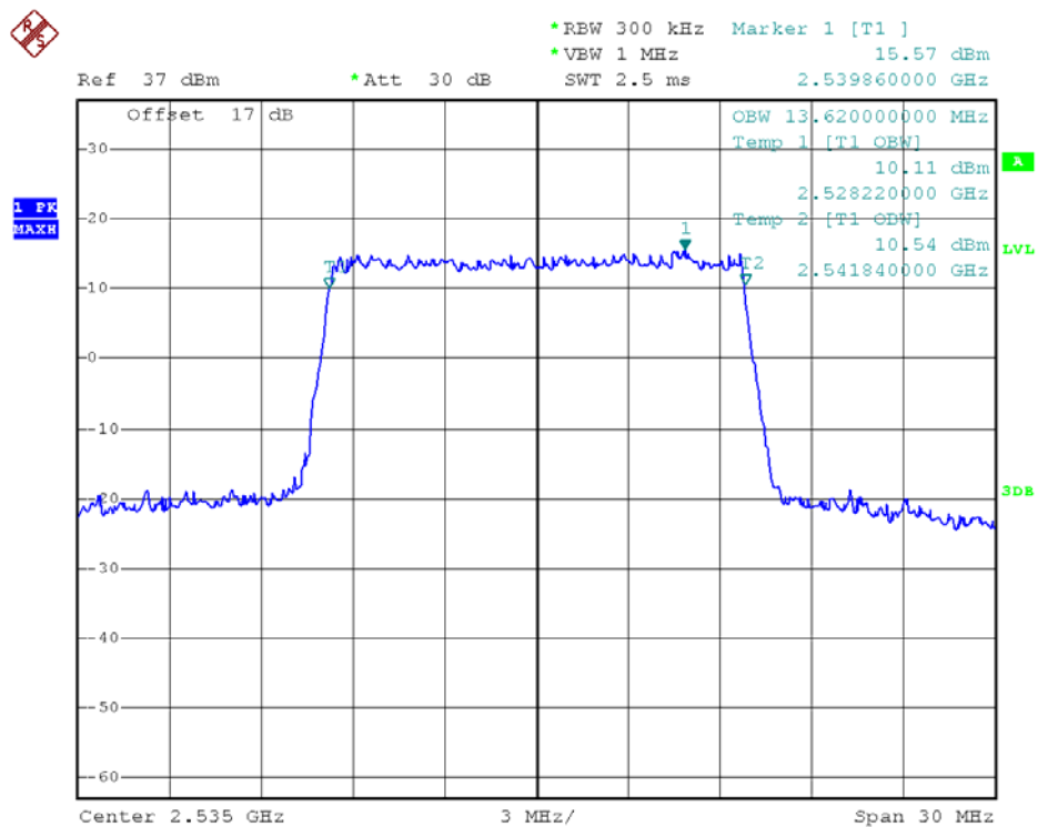
99% Occupied Bandwidth LTE Band 7/15MHz/16QAM
