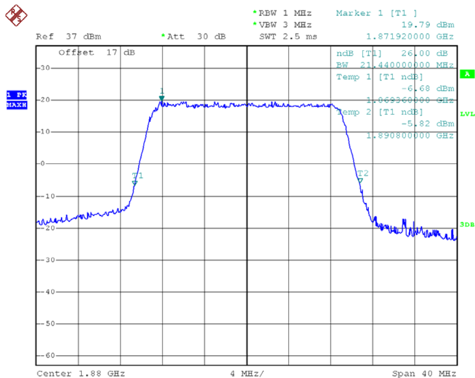
26dB Bandwidth LTE Band 2/20MHz/QPSK
