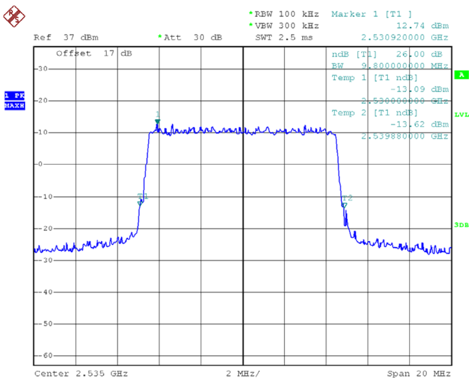
26dB Bandwidth LTE Band 7/10MHz/QPSK
