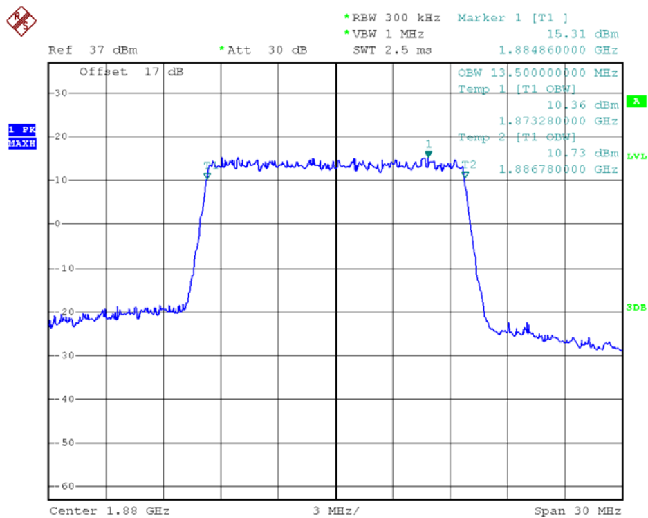
99% Occupied Bandwidth LTE Band 2/15MHz/16QAM
