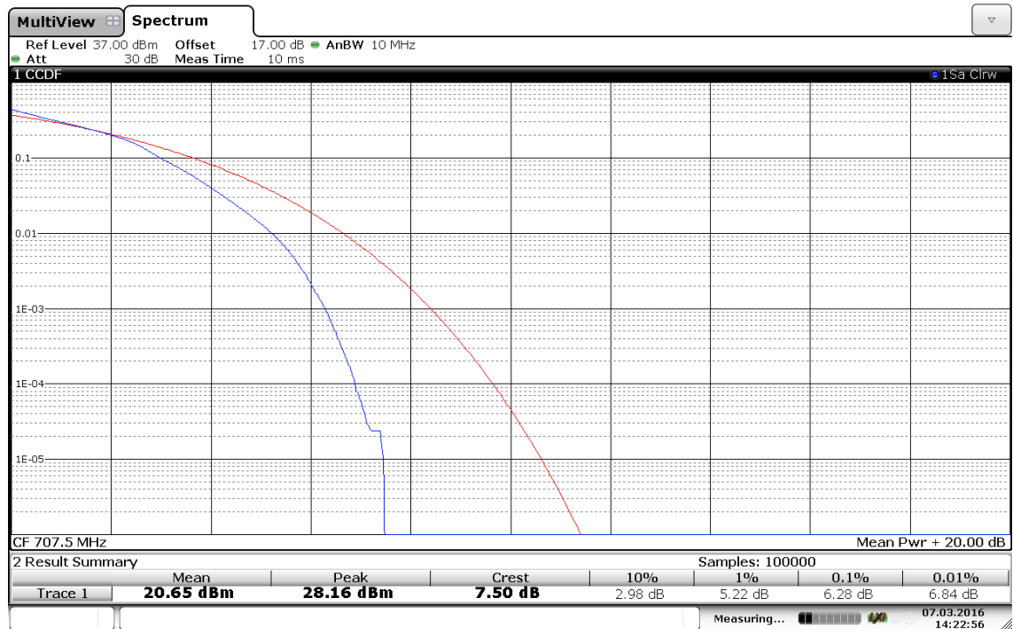
(Plot E3: Band 12/10MHz/16QAM in M Ch 1RB Size)
