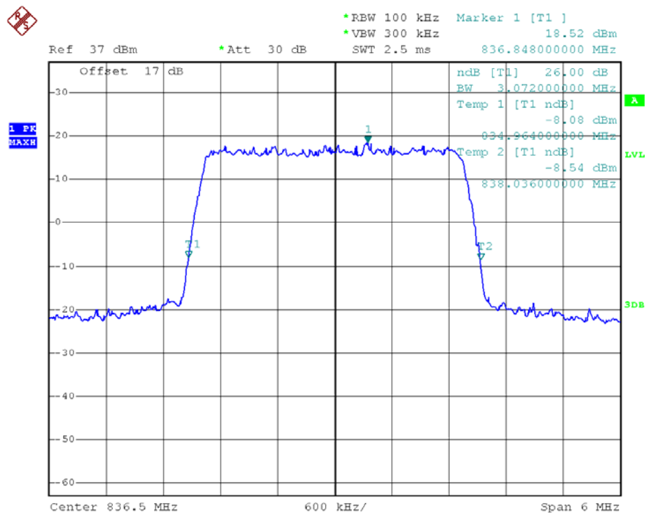
26dB Bandwidth LTE Band 5/3MHz/QPSK
