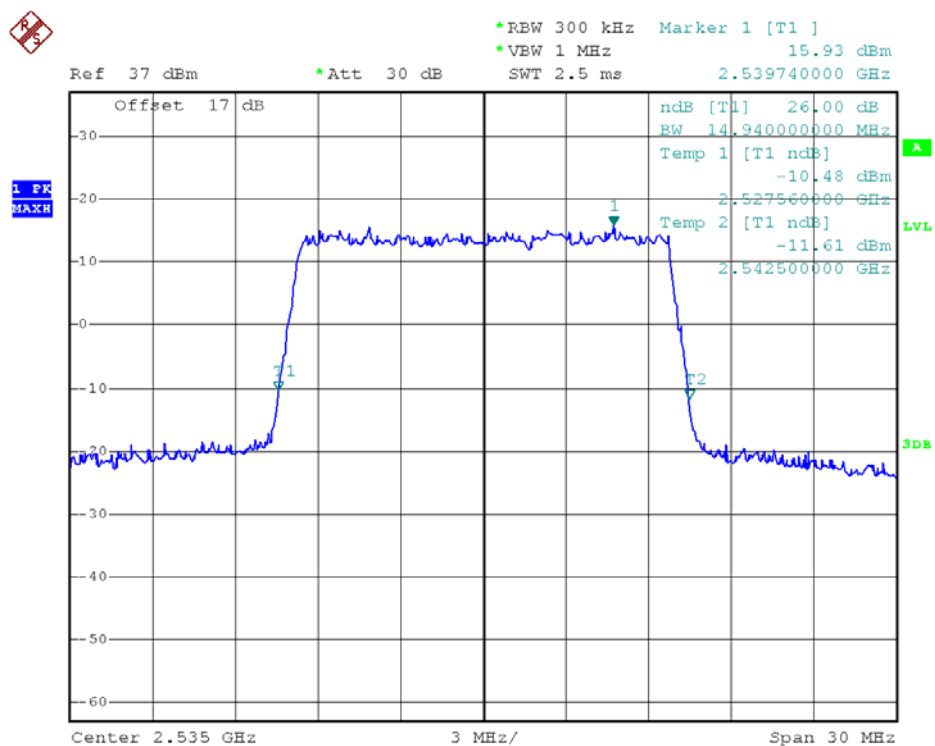
26dB Bandwidth LTE Band 7/15MHz/16QAM
