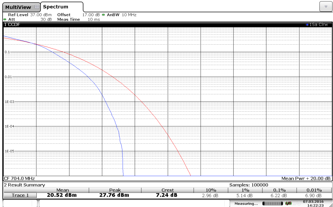
(Plot E1: Band 12/10MHz/16QAM in L Ch 1RB Size )
