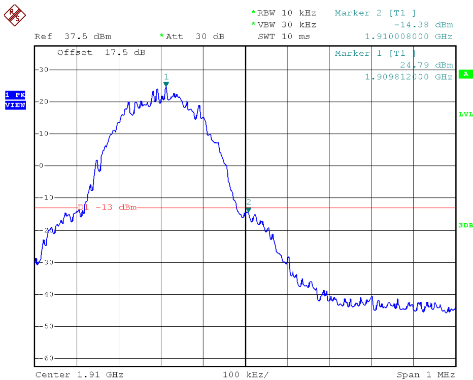
(Plot D: GSM 1900 Channel = 810)
