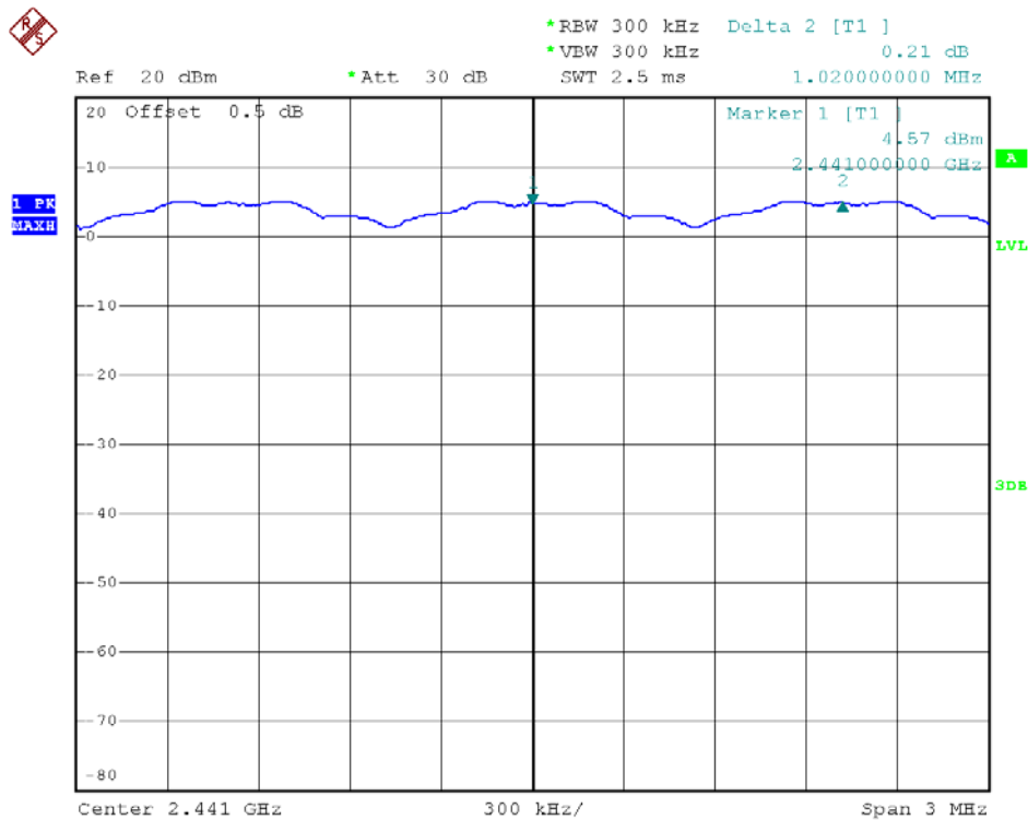
8-DPSK Mode
