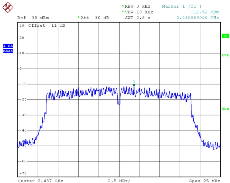
802.11n20 - Channel 6
