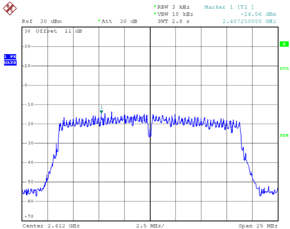
802.11n20 - Channel 1
