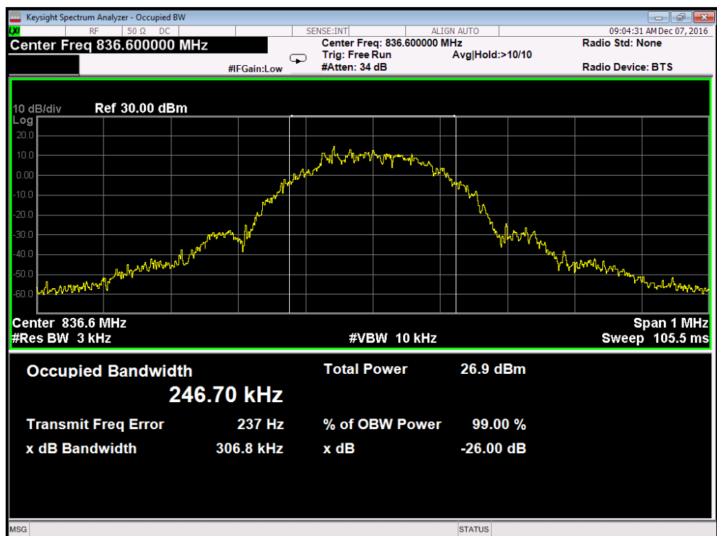
(Plot C2: EDGE 850MHz Channel = 190 Occupied bandwidth)
