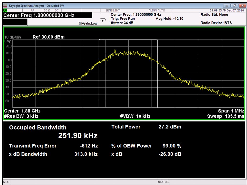
(Plot D2: EDGE 1900MHz Channel = 661 Occupied bandwidth)
