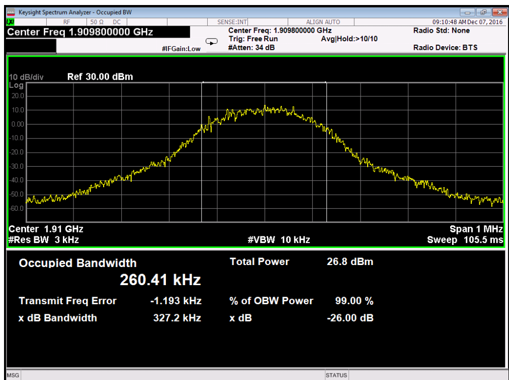
(Plot D3: EDGE 1900MHz Channel = 810 Occupied bandwidth)
