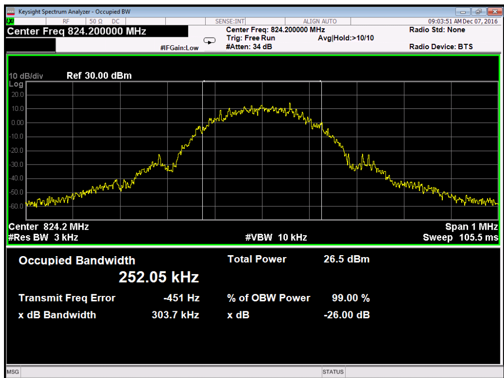
(Plot C1: EDGE 850MHz Channel = 128 Occupied bandwidth)
