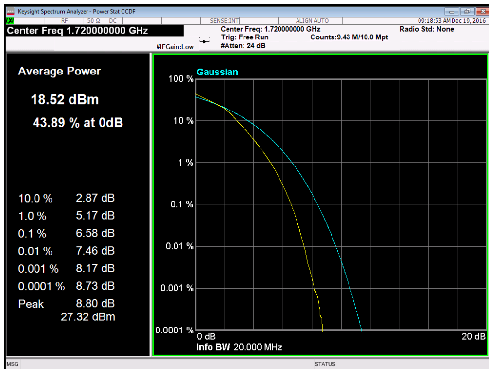
(Plot B2: Band 4/20MHz/16QAM in L Ch 100RB Size)
