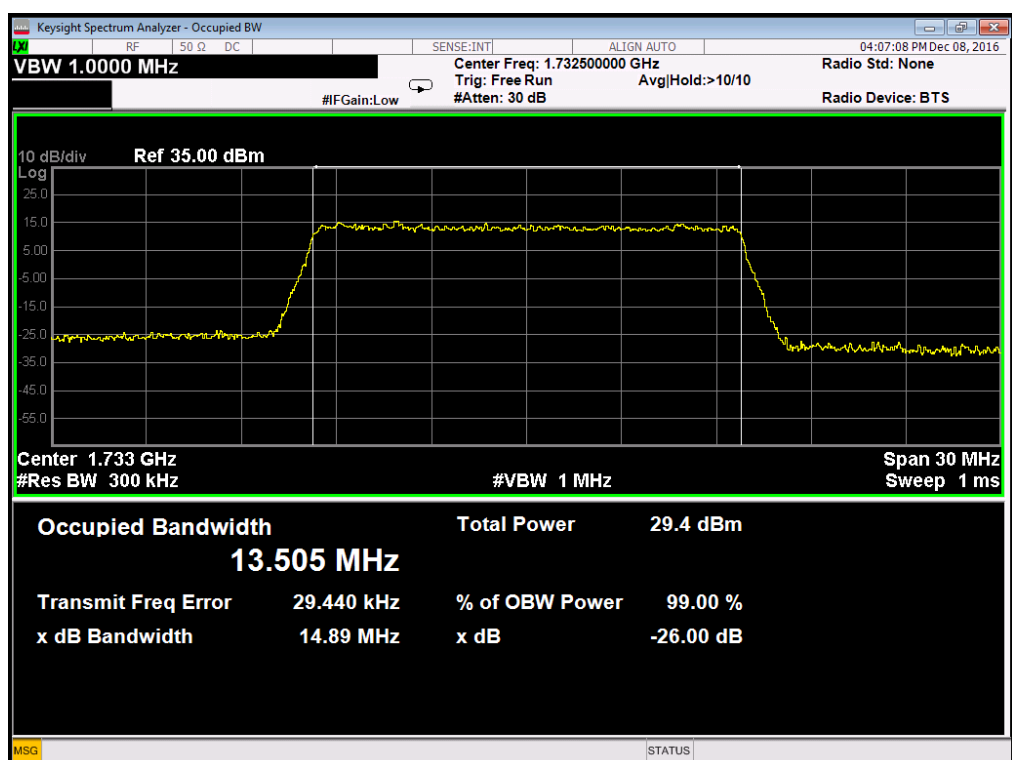
Occupied Bandwidth LTE Band 4/15MHz/16QAM
