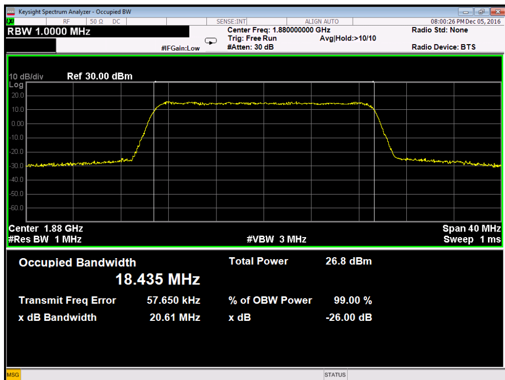
Occupied Bandwidth LTE Band 2/20MHz/QPSK
