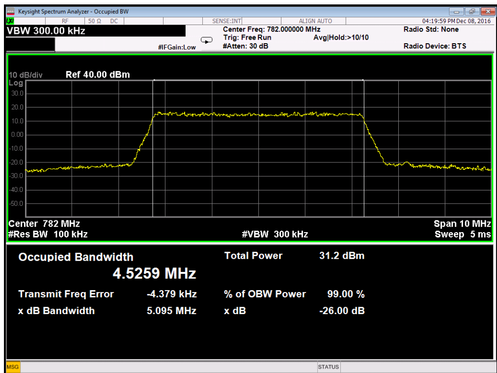
Occupied Bandwidth LTE Band 13/5MHz/QPSK
