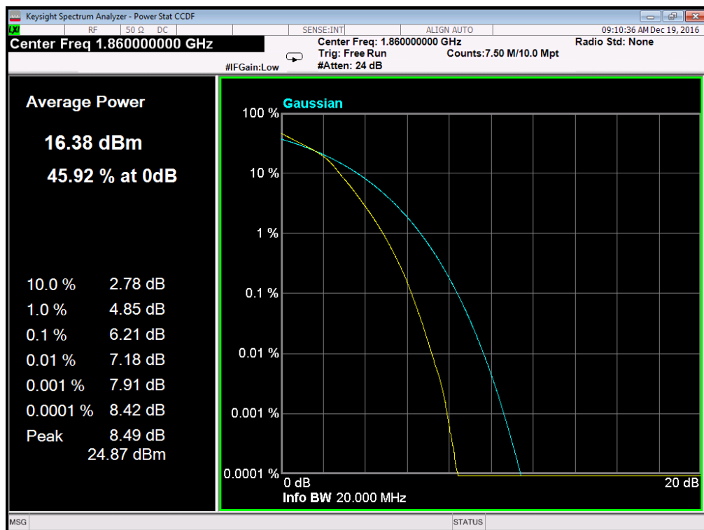
(Plot A2: Band 2/20MHz/16QAM in L Ch 100RB Size)
