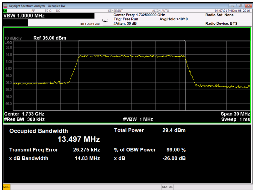
Occupied Bandwidth LTE Band 4/15MHz/QPSK
