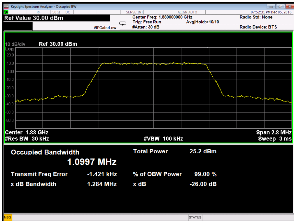
Occupied Bandwidth LTE Band 2 1.4MHz/16QAM
