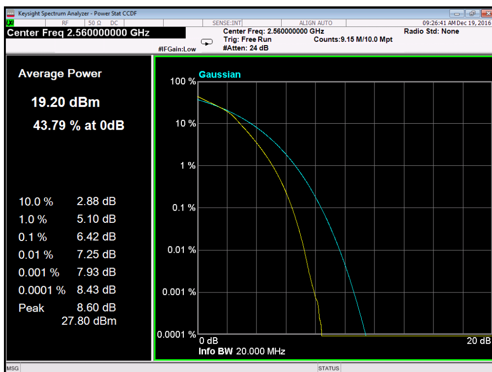
(Plot C6: Band 7/20MHz/16QAM in H Ch 100RB Size)
