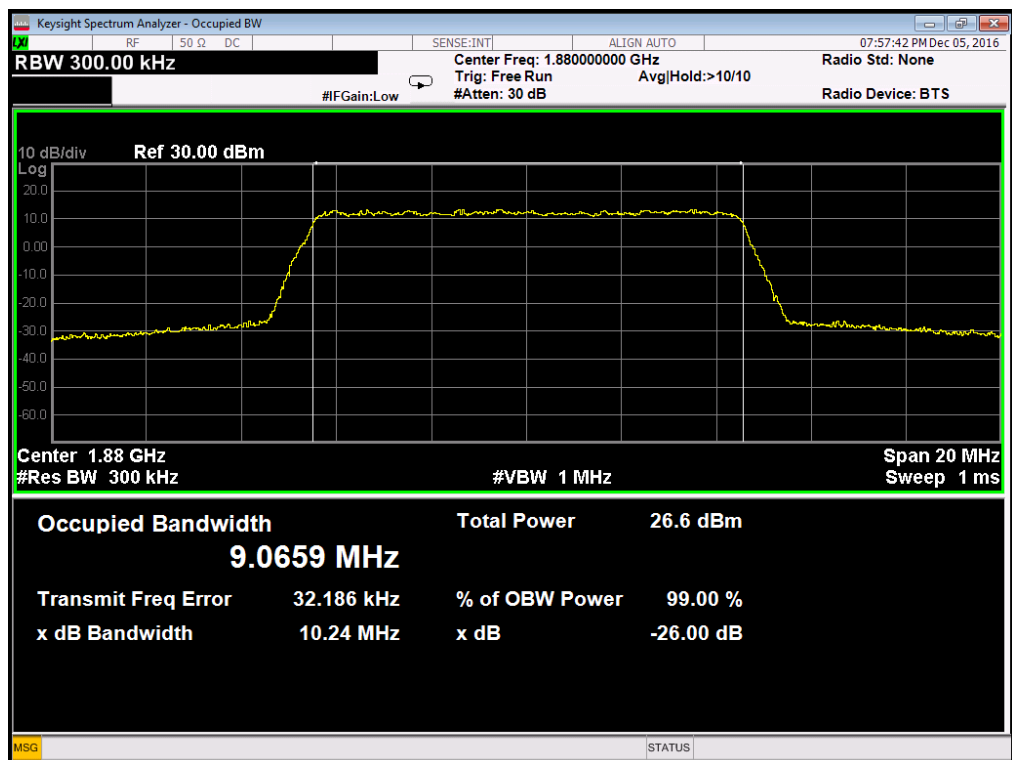
Occupied Bandwidth LTE Band 2/10MHz/QPSK
