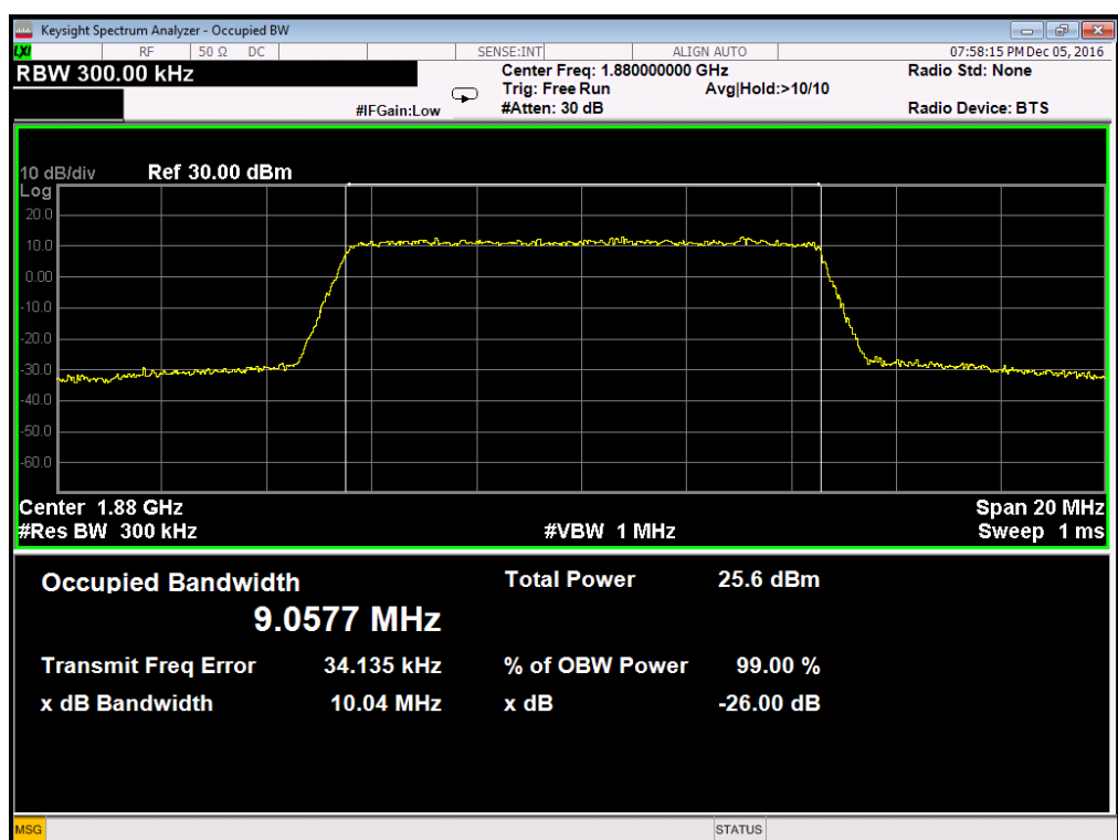
Occupied Bandwidth LTE Band 2/10MHz/16QAM
