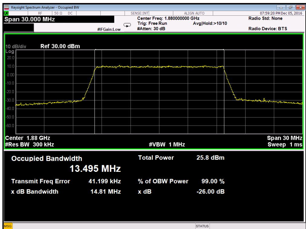
Occupied Bandwidth LTE Band 2/15MHz/16QAM
