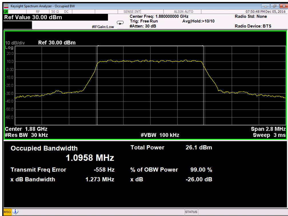
Occupied Bandwidth LTE Band 2 1.4MHz/QPSK
