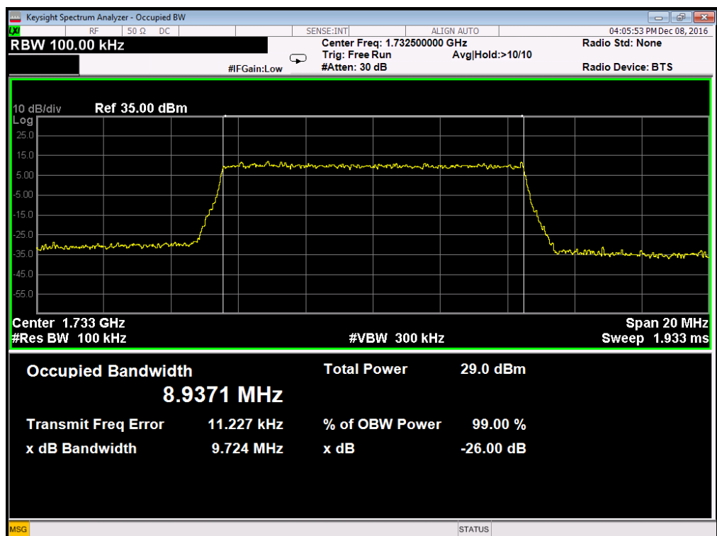
Occupied Bandwidth LTE Band 4/10MHz/16QAM
