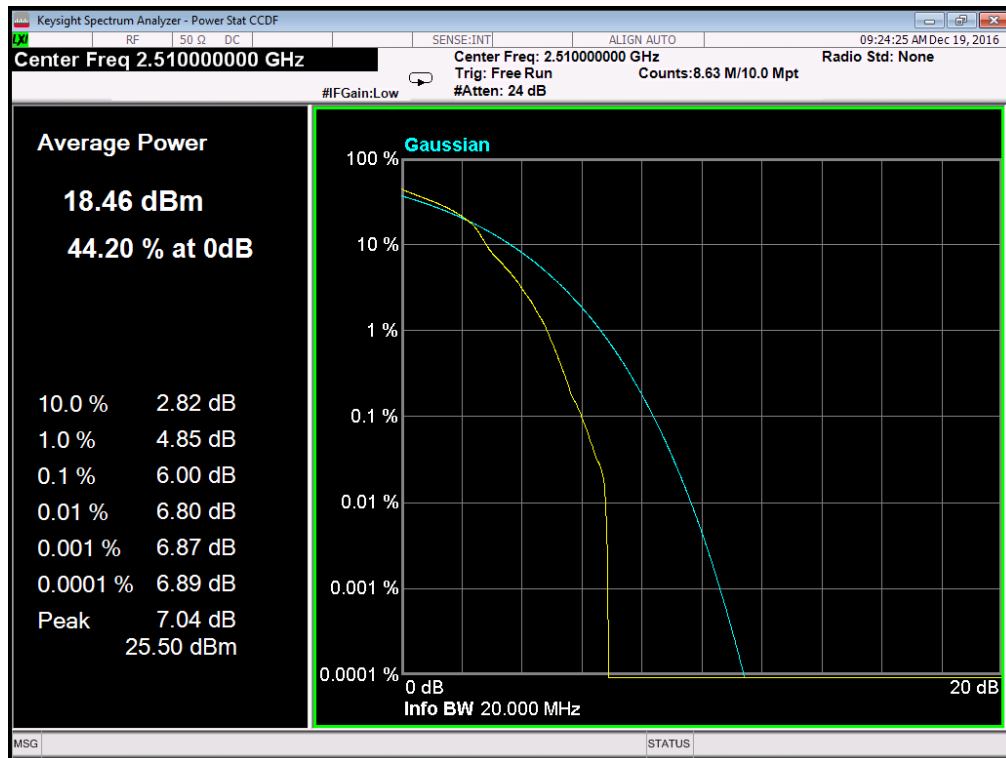
(Plot C1: Band 7/20MHz/16QAM in L Ch 1RB Size )
