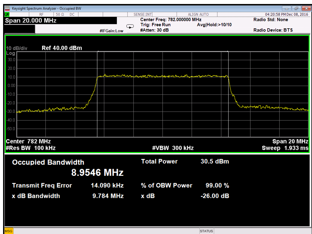
Occupied Bandwidth LTE Band 13/10MHz/16QAM
