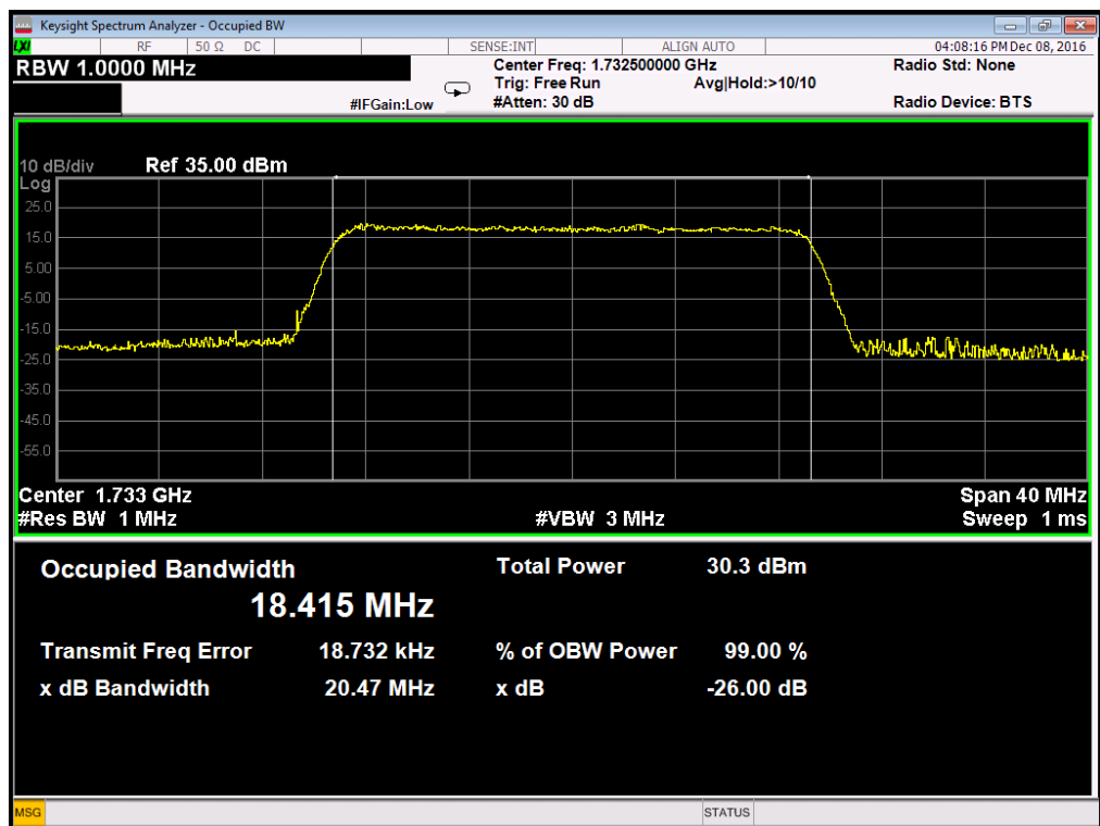
Occupied Bandwidth LTE Band 4/20MHz/QPSK
