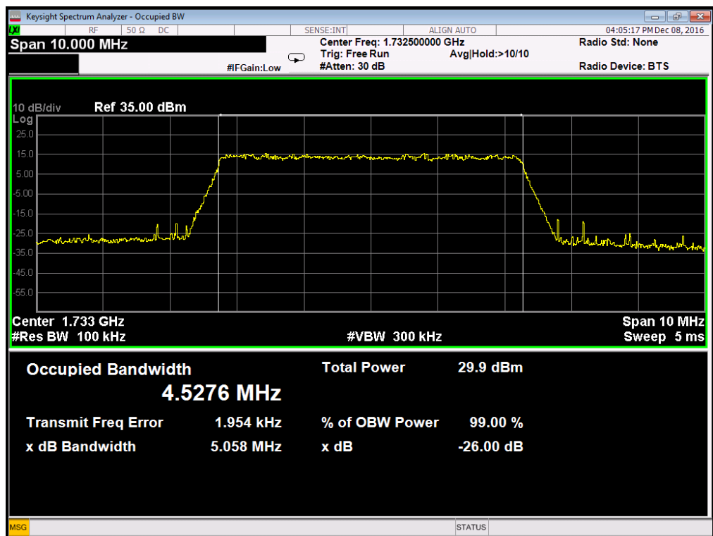
Occupied Bandwidth LTE Band 4/5MHz/QPSK
