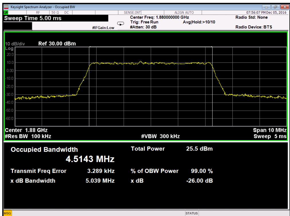
Occupied Bandwidth LTE Band 2/5MHz/16QAM
