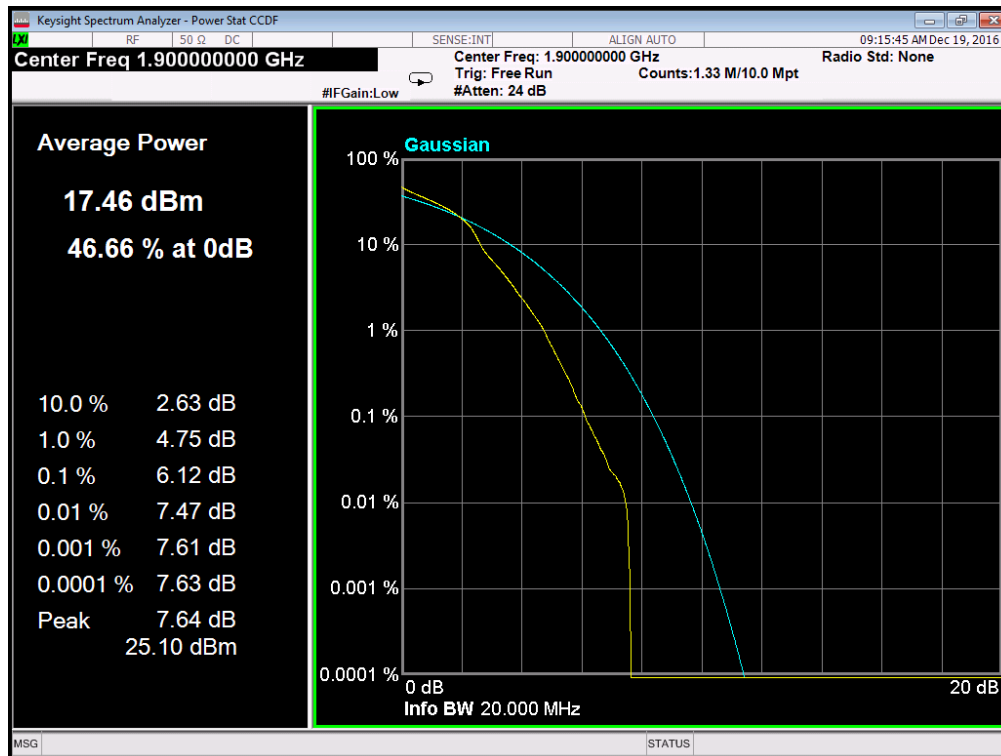
(Plot A5: Band 2/20MHz/16QAM in H Ch 1RB Size)
