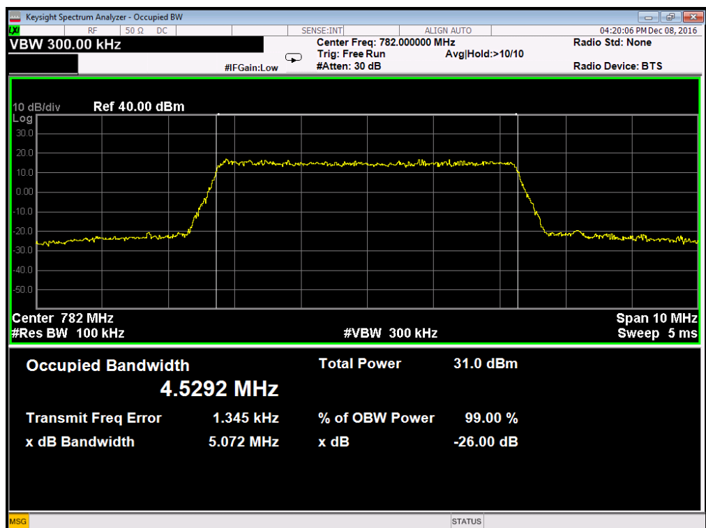
Occupied Bandwidth LTE Band 13/5MHz/16QAM
