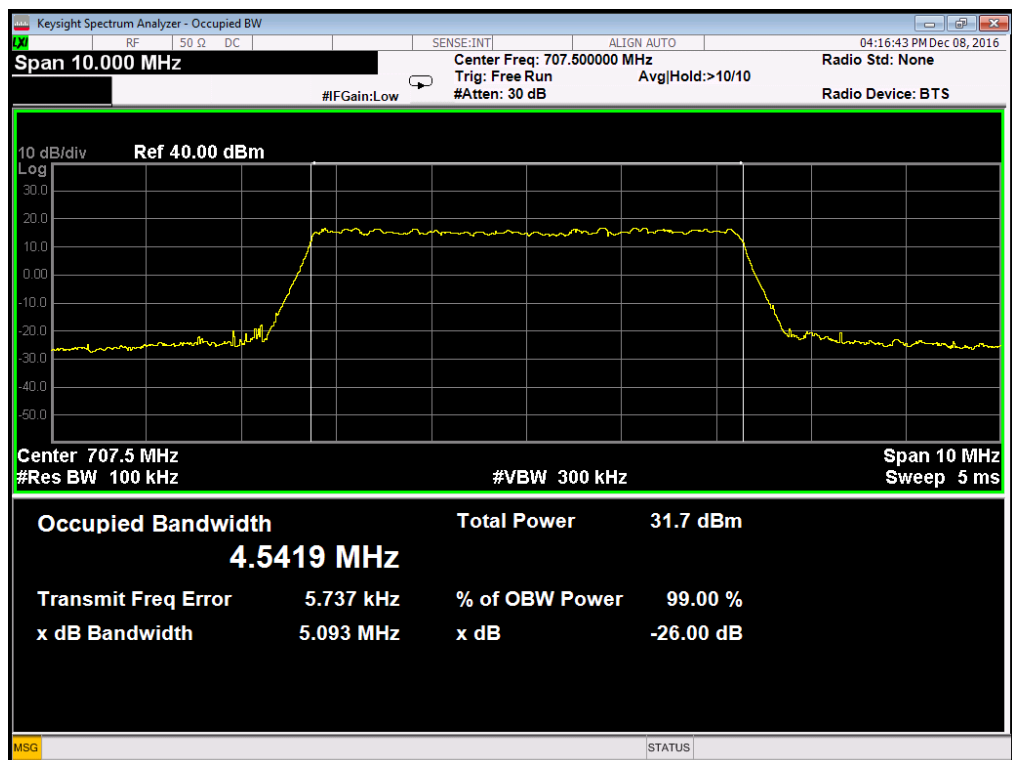
Occupied Bandwidth LTE Band 12/5MHz/QPSK
