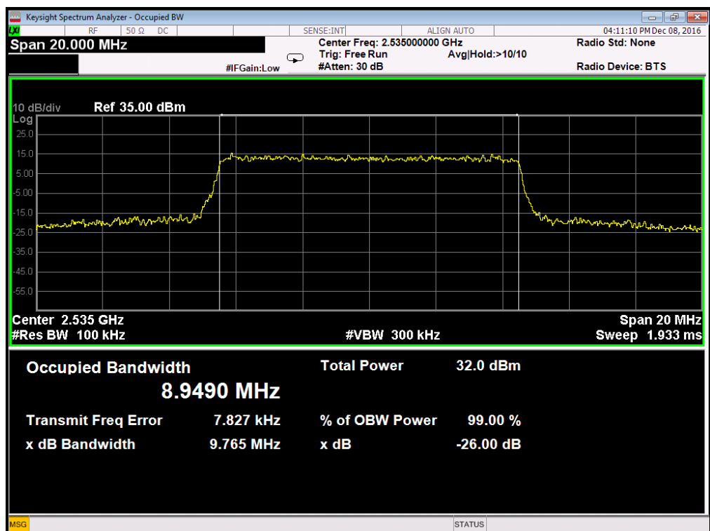
Occupied Bandwidth LTE Band 7/10MHz/16QAM
