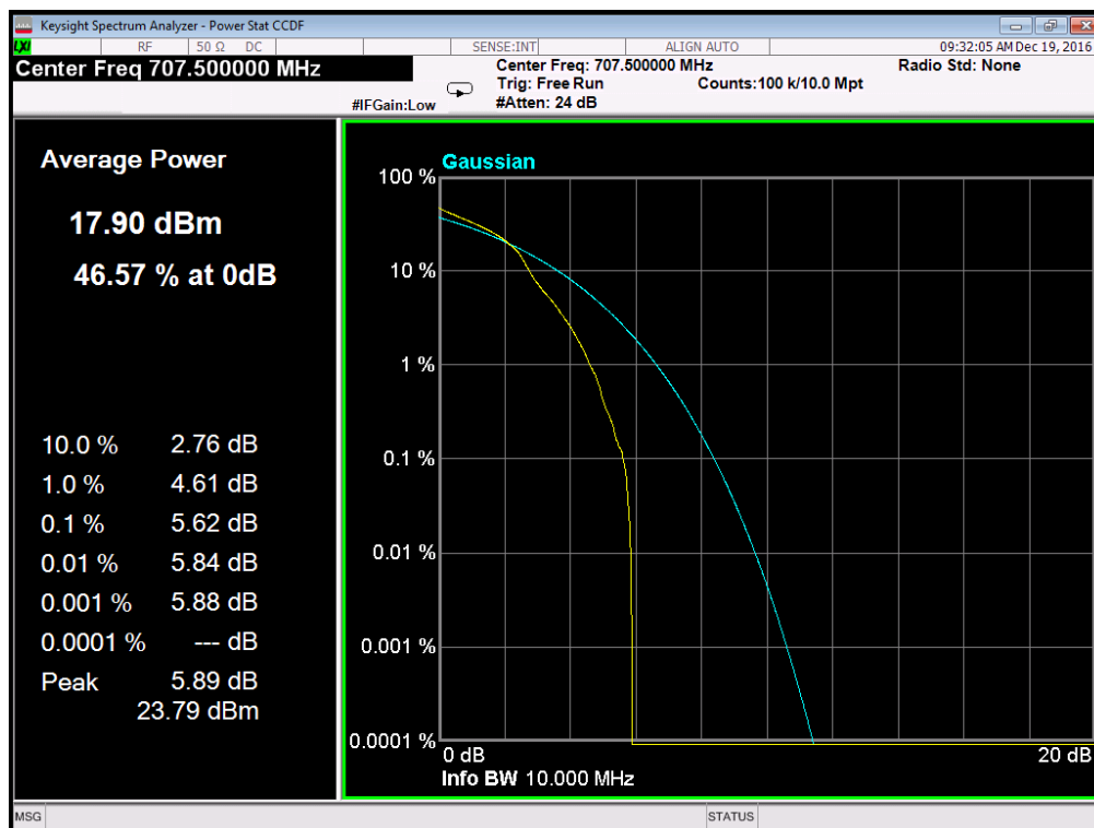
(Plot D3: Band 12/10MHz/16QAM in M Ch 1RB Size)
