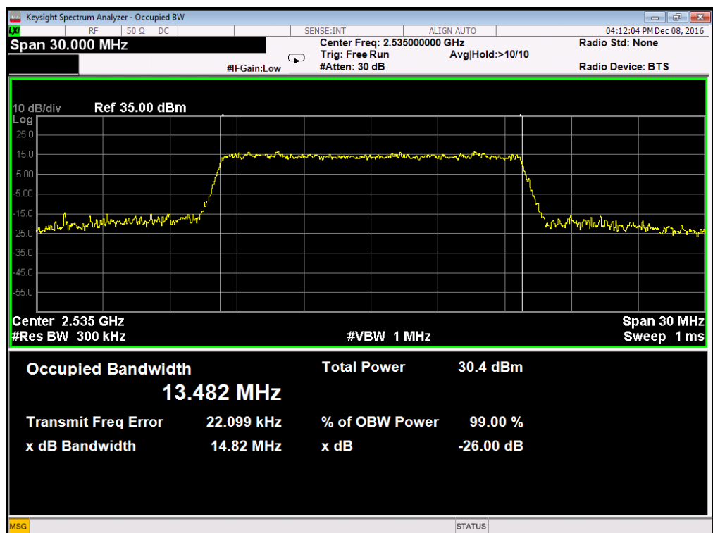
Occupied Bandwidth LTE Band 7/15MHz/16QAM
