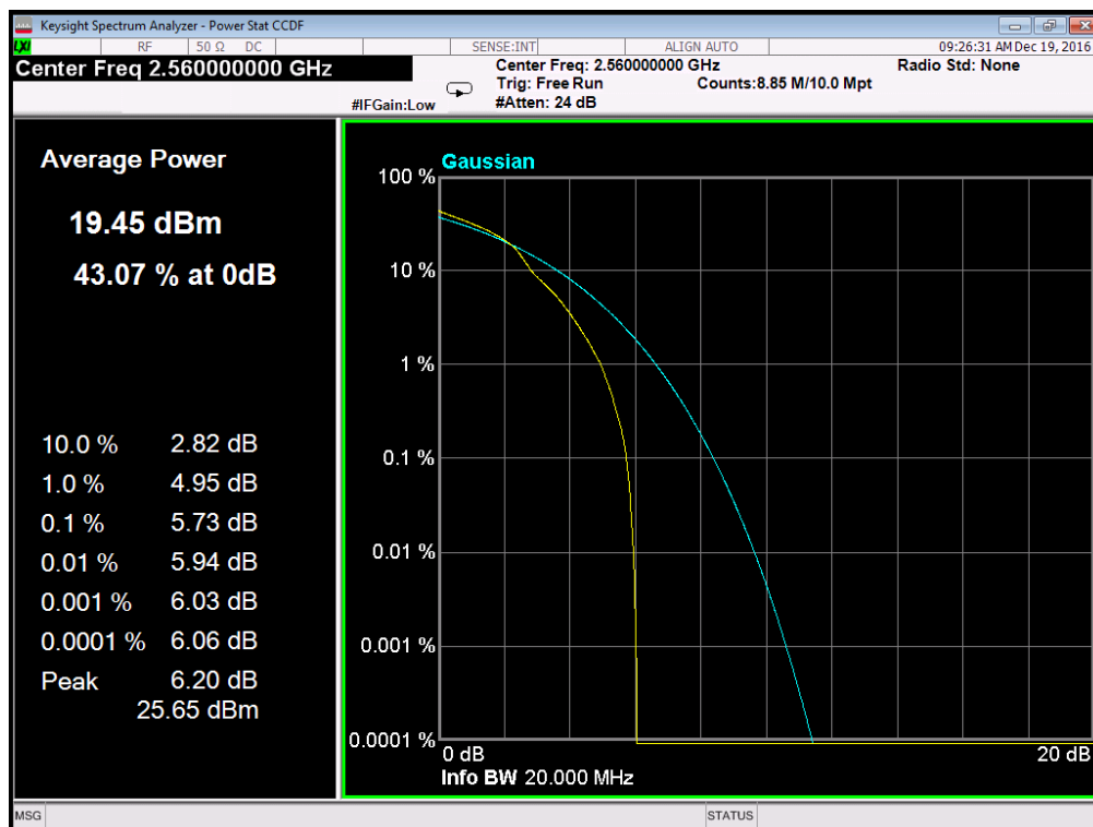
(Plot C5: Band 7/20MHz/16QAM in H Ch 1RB Size)
