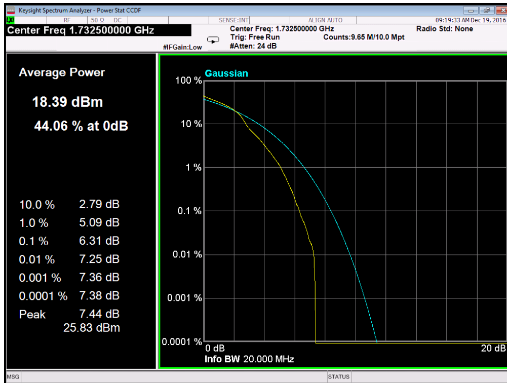
(Plot B3: Band 4/20MHz/16QAM in M Ch 1RB Size)
