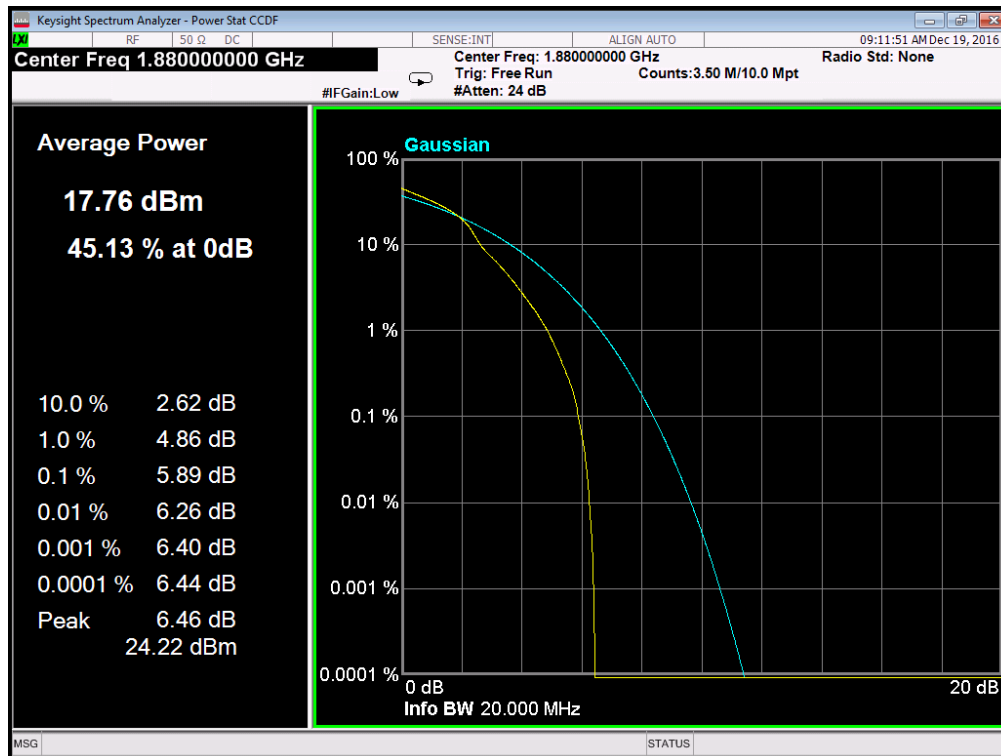
(Plot A3: Band 2/20MHz/16QAM in M Ch 1RB Size)
