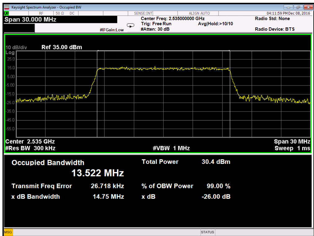
Occupied Bandwidth LTE Band 7/15MHz/QPSK
