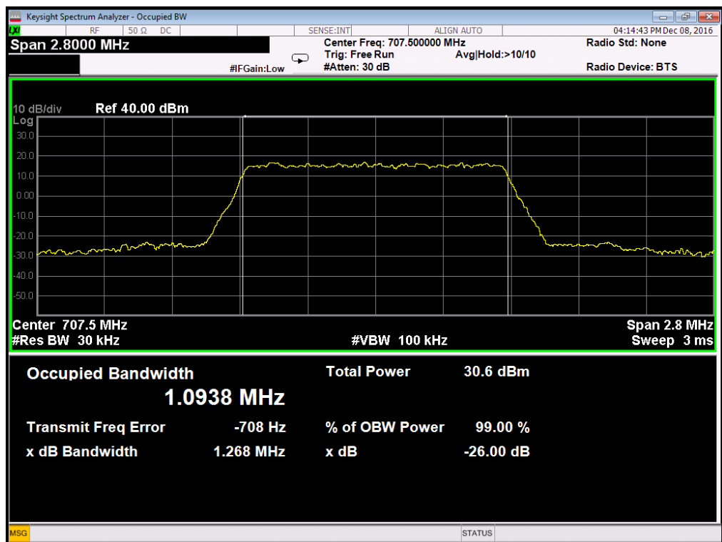
Occupied Bandwidth LTE Band 12/1.4MHz/QPSK
