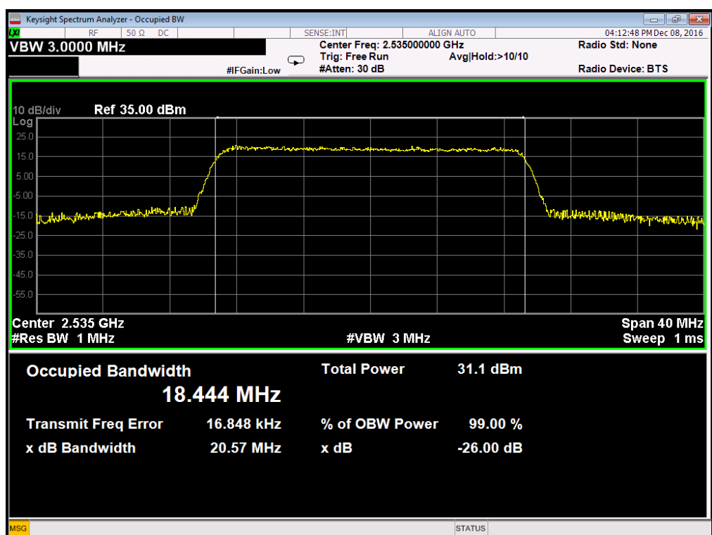
Occupied Bandwidth LTE Band 7/20MHz/16QAM
