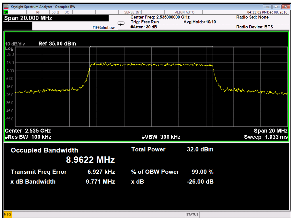
Occupied Bandwidth LTE Band 7/10MHz/QPSK
