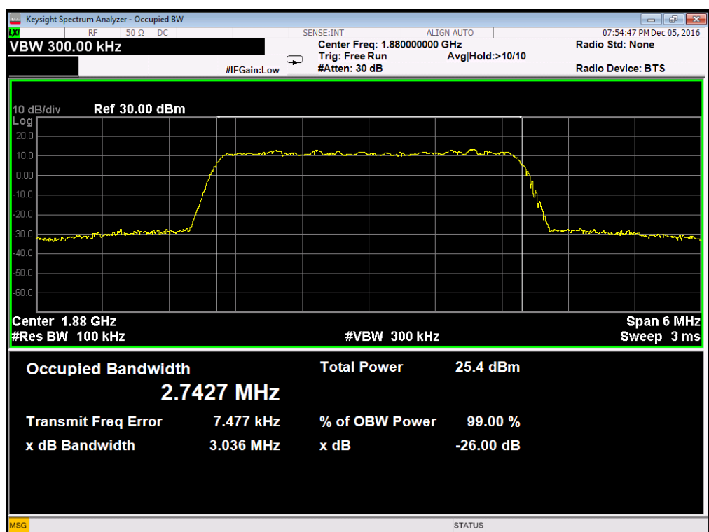
Occupied Bandwidth LTE Band 2/3MHz/16QAM
