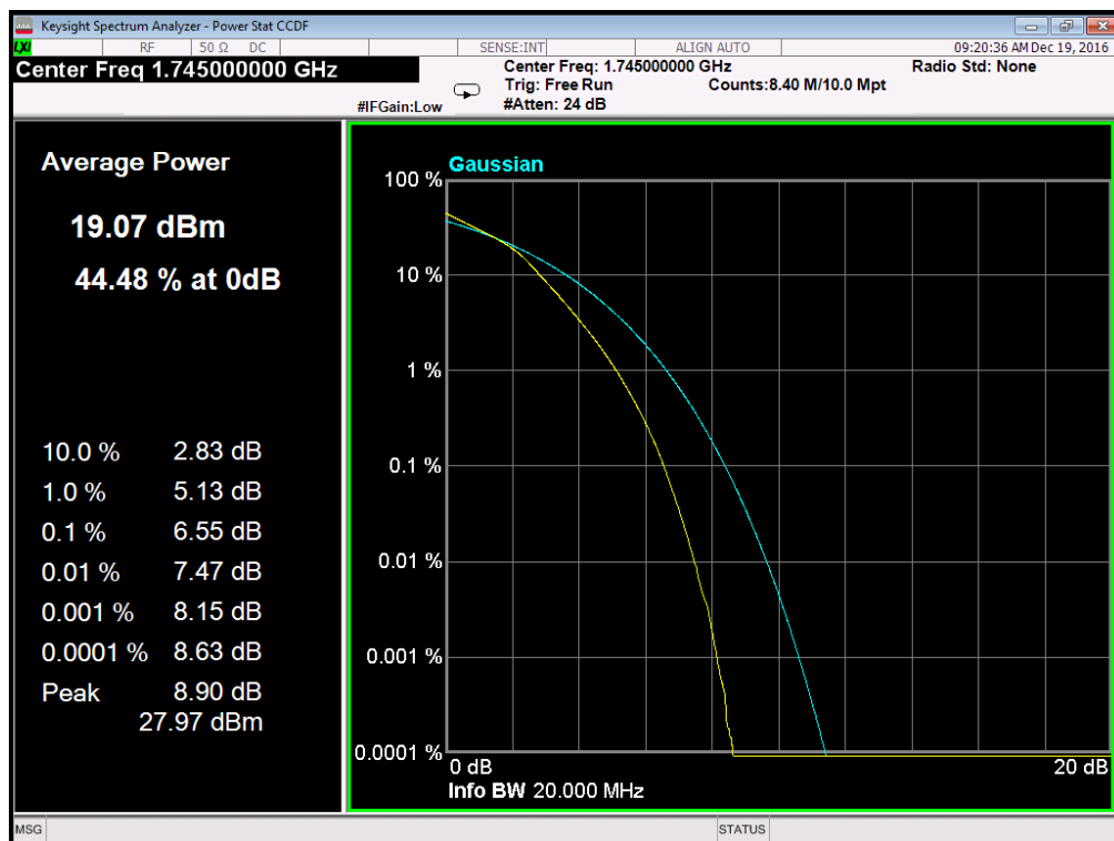
(Plot B6: Band 4/20MHz/16QAM in H Ch 100RB Size)
