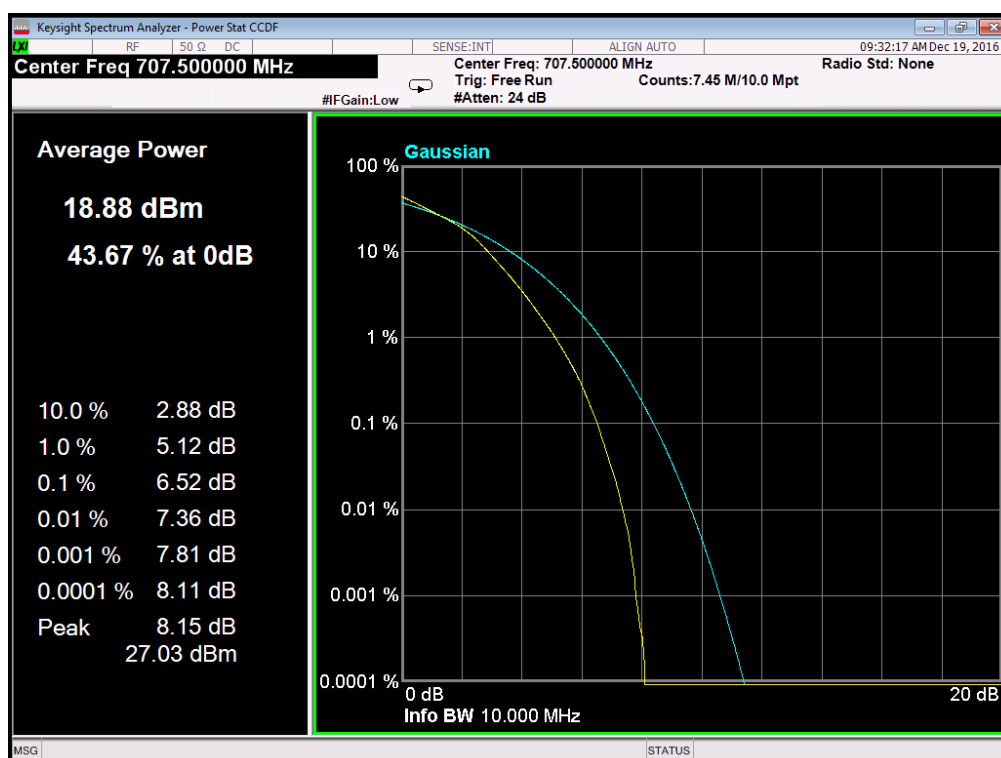
(Plot D4: Band 12/10MHz/16QAM in M Ch 50RB Size)
