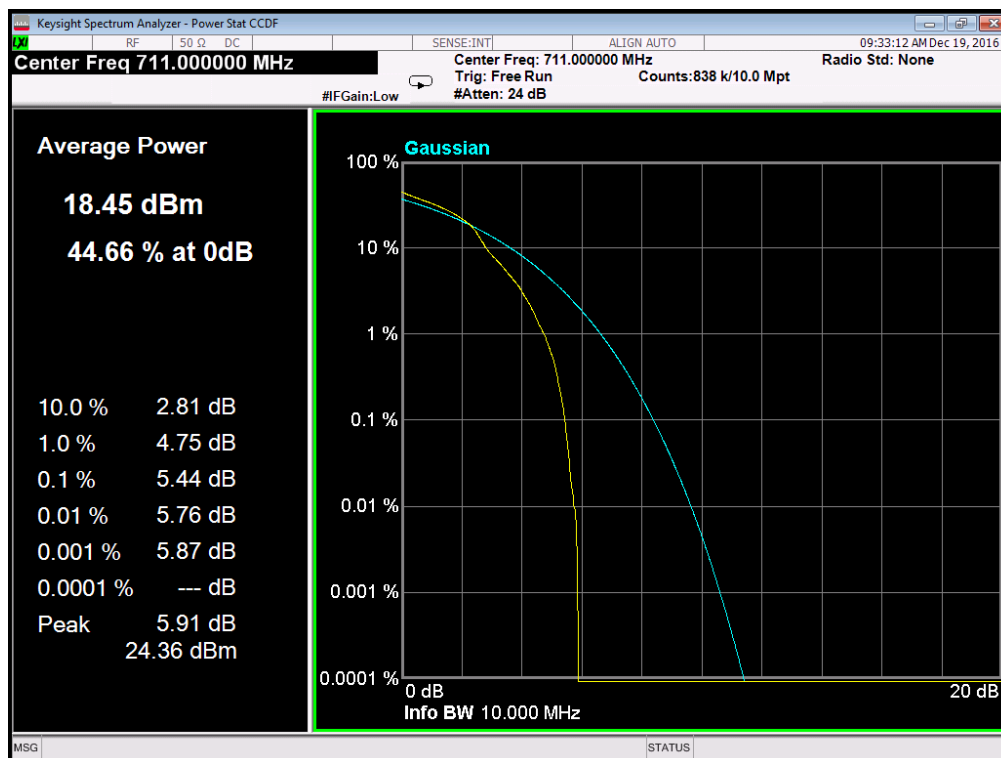
(Plot D5: Band 12/10MHz/16QAM in H Ch 1RB Size)
