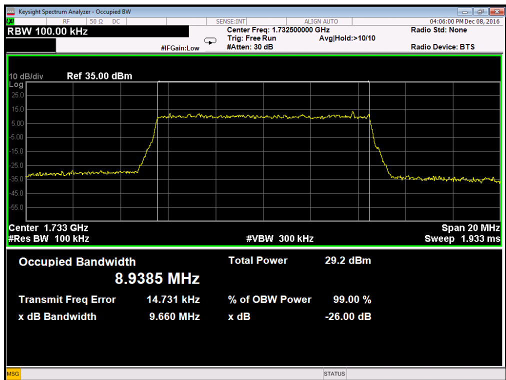
Occupied Bandwidth LTE Band 4/10MHz/QPSK
