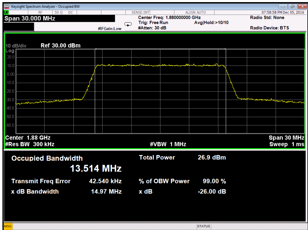
Occupied Bandwidth LTE Band 2/15MHz/QPSK
