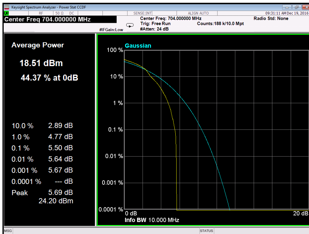
(Plot D1: Band 12/10MHz/16QAM in L Ch 1RB Size )
