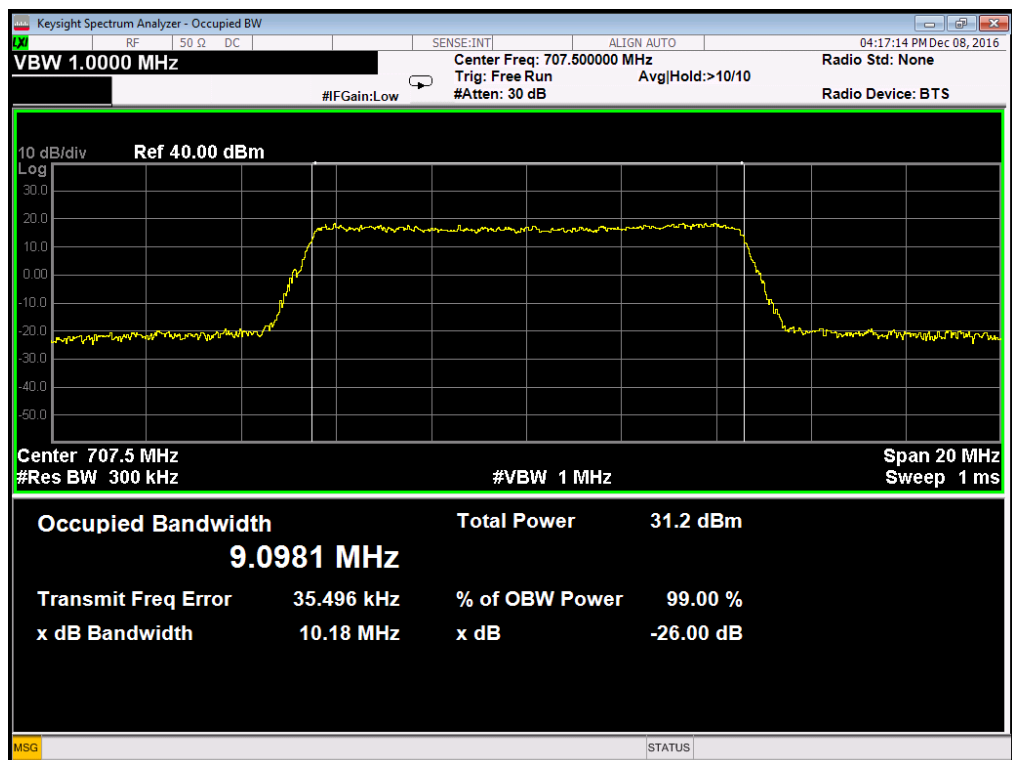
Occupied Bandwidth LTE Band 12/10MHz/QPSK
