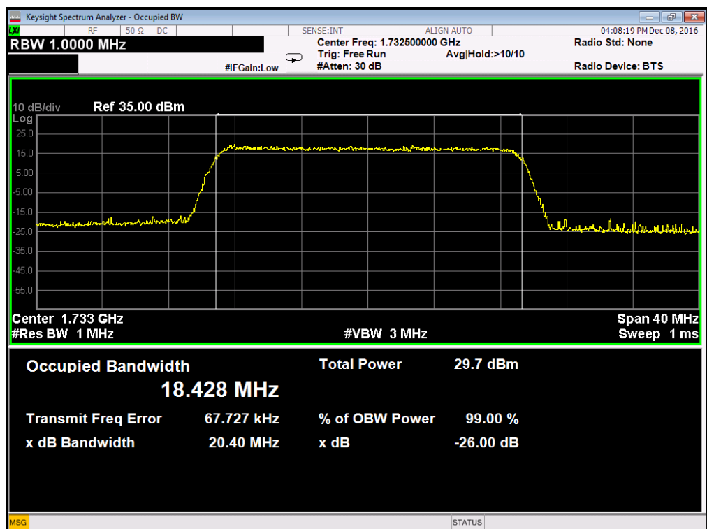
Occupied Bandwidth LTE Band 4/20MHz/16QAM
