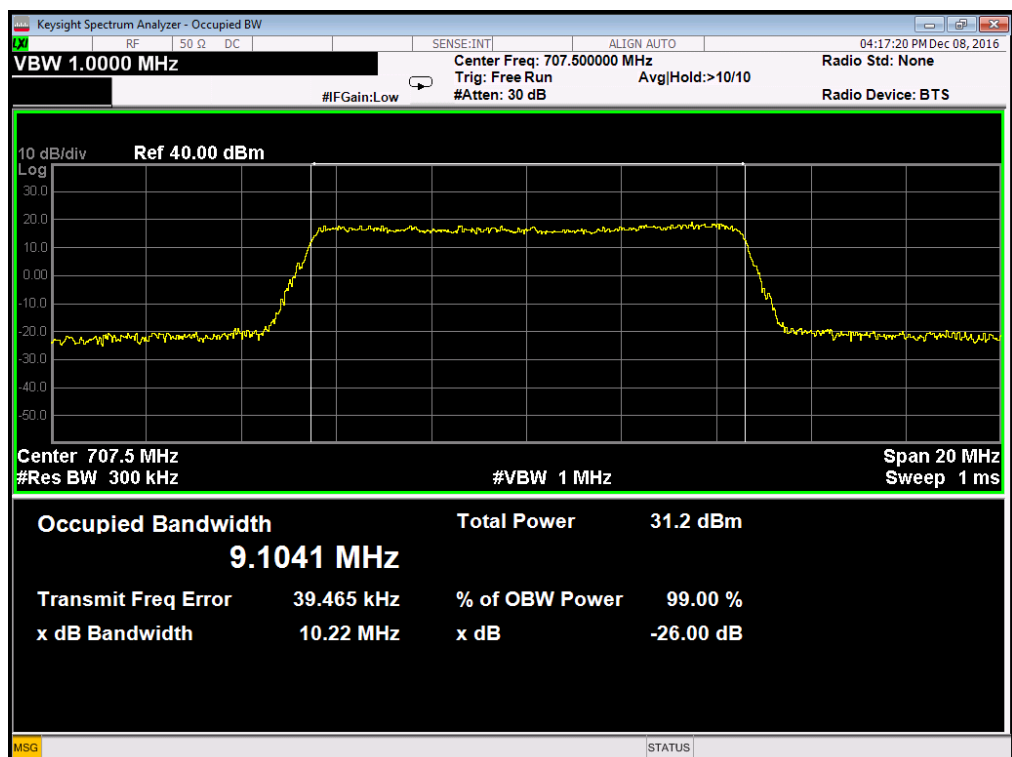
Occupied Bandwidth LTE Band 12/10MHz/16QAM
