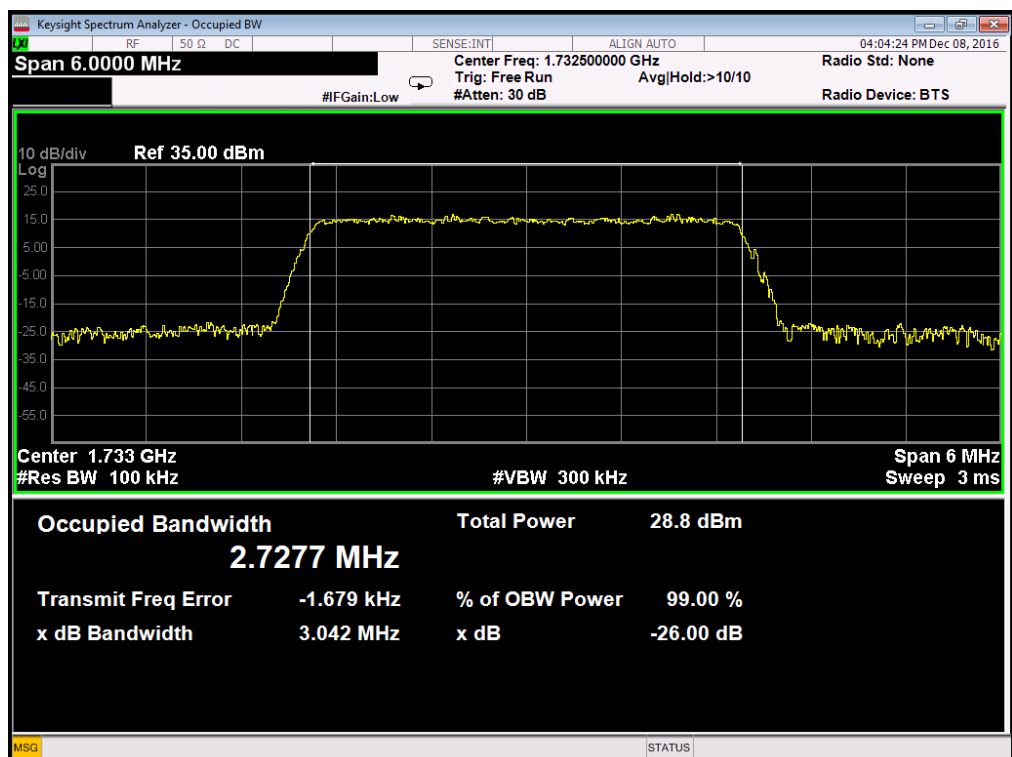
Occupied Bandwidth LTE Band 4/3MHz/16QAM
