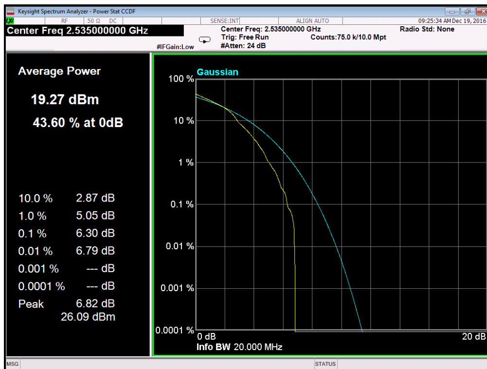
(Plot C3: Band 7/20MHz/16QAM in M Ch 1RB Size)
