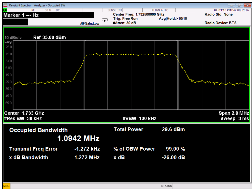
Occupied Bandwidth LTE Band 4/1.4MHz/QPSK
