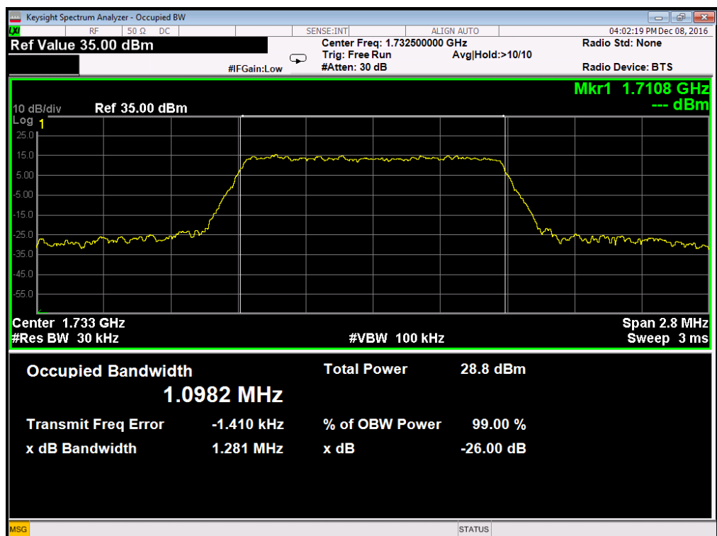
Occupied Bandwidth LTE Band 4/1.4MHz/16QAM
