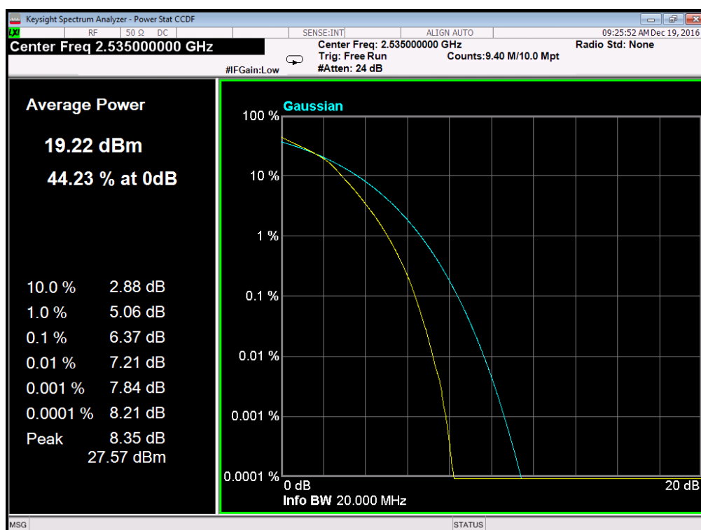
(Plot C4: Band 7/20MHz/16QAM in M Ch 100RB Size)
