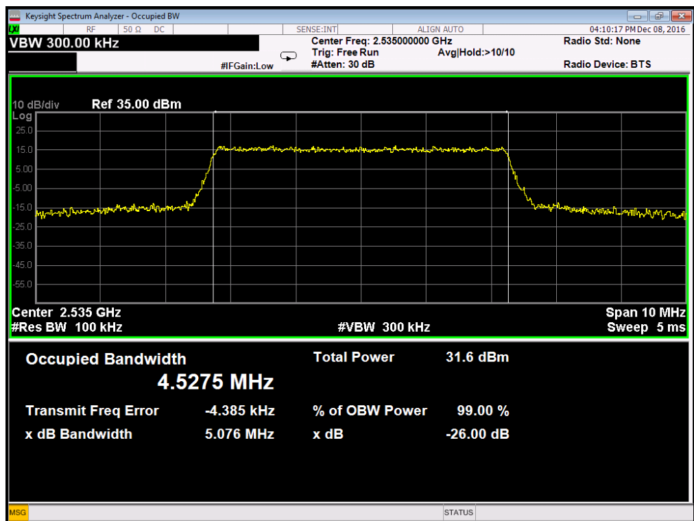
Occupied Bandwidth LTE Band 7/5MHz/QPSK
