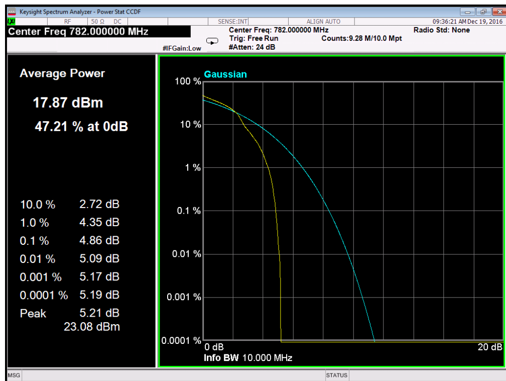
(Plot E1: Band 13/10MHz/16QAM in L/M/H Ch 1RB Size)
