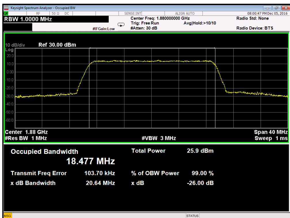
Occupied Bandwidth LTE Band 2/20MHz/16QAM
