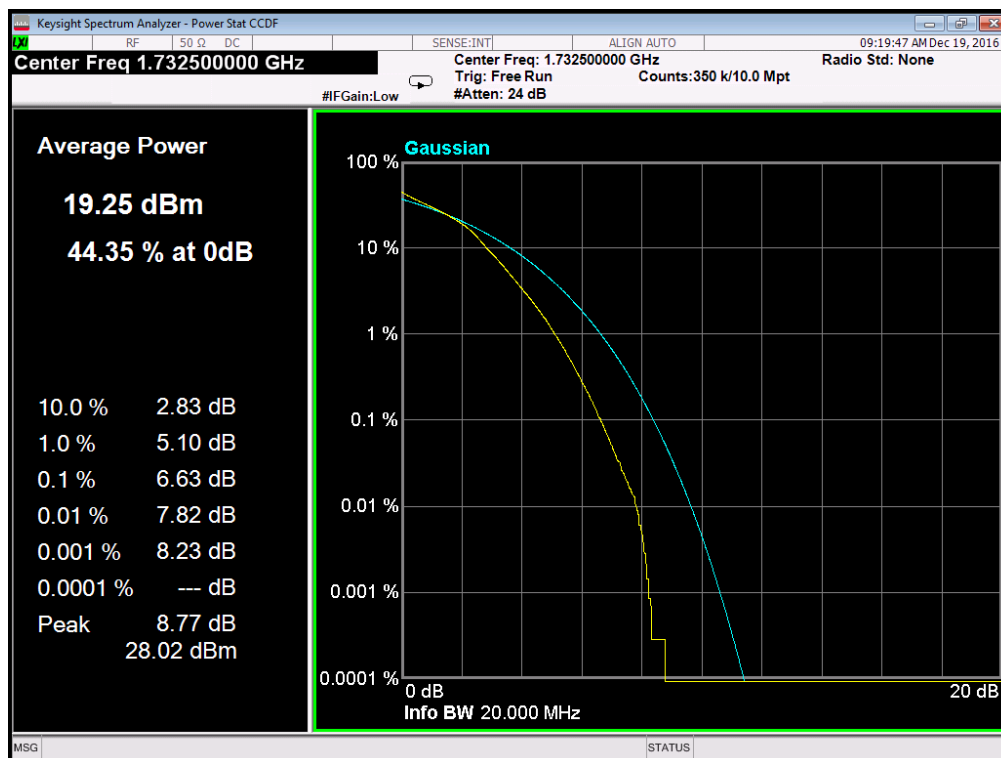
(Plot B4: Band 4/20MHz/16QAM in M Ch 100RB Size)
