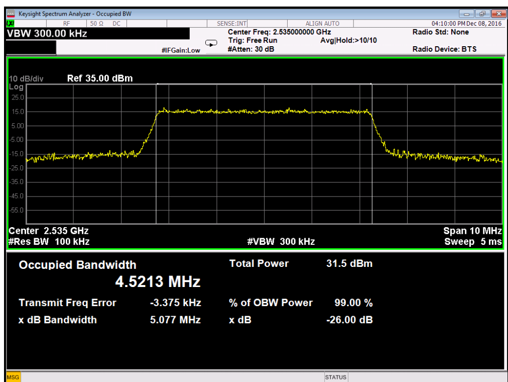
Occupied Bandwidth LTE Band 7/5MHz/16QAM
