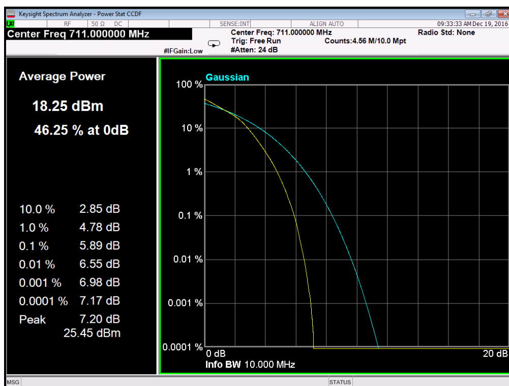
(Plot D6: Band 12/10MHz/16QAM in H Ch 50RB Size)
