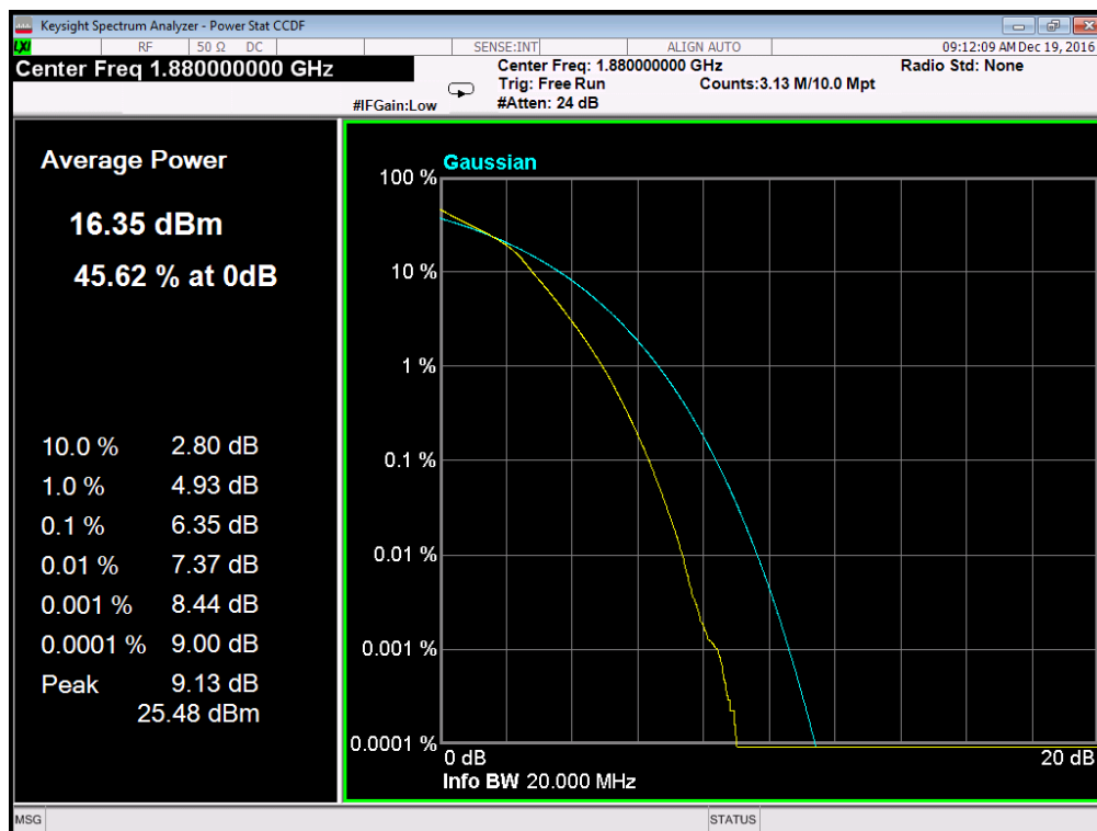
(Plot A4: Band 2/20MHz/16QAM in M Ch 100RB Size)
