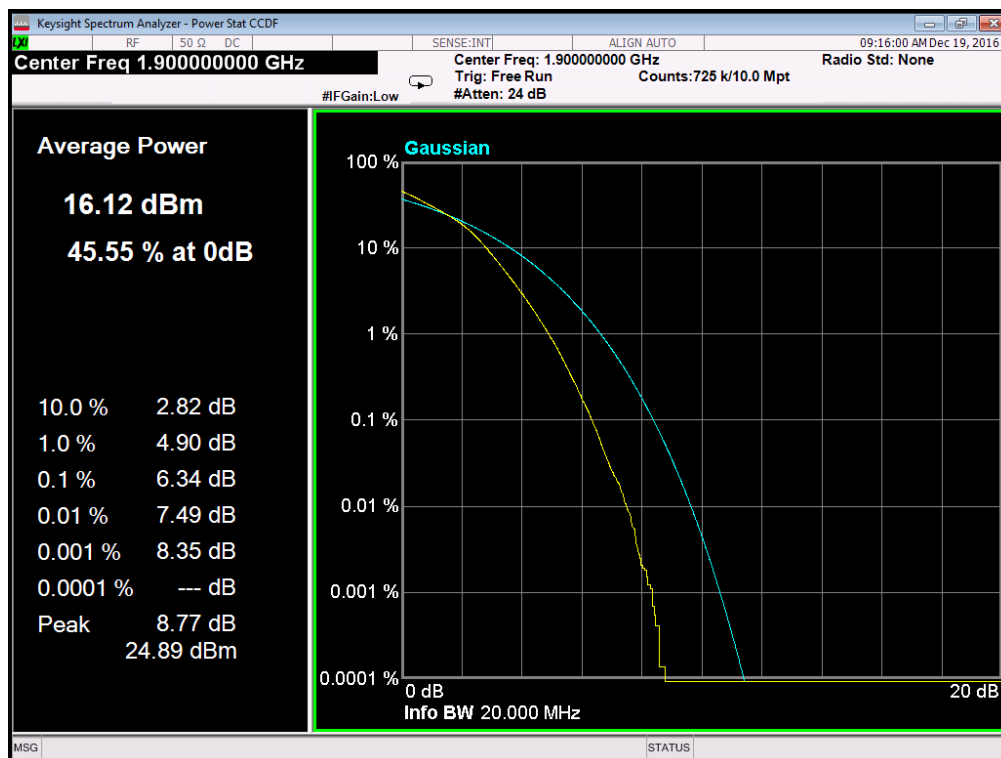
(Plot A6: Band 2/20MHz/16QAM in H Ch 100RB Size)
