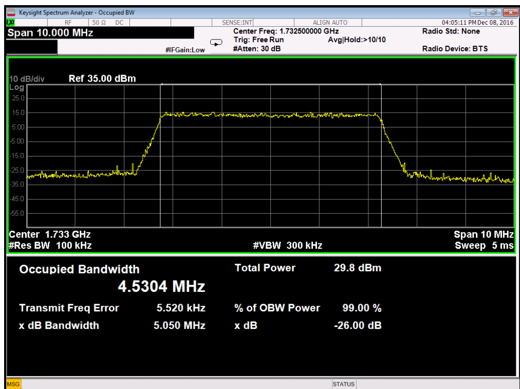
Occupied Bandwidth LTE Band 4/5MHz/16QAM
