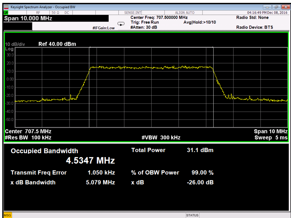
Occupied Bandwidth LTE Band 12/5MHz/16QAM
