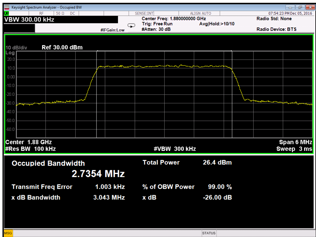
Occupied Bandwidth LTE Band 2/3MHz/QPSK
