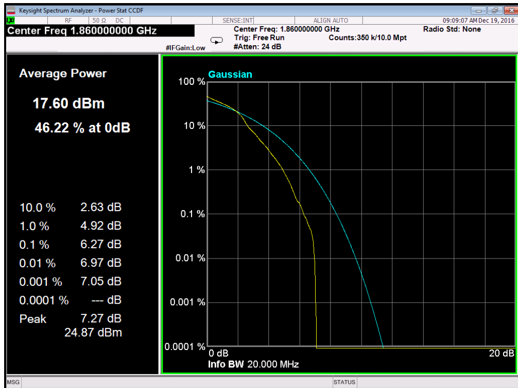
(Plot A1: Band 2/20MHz/16QAM in L Ch 1RB Size)
