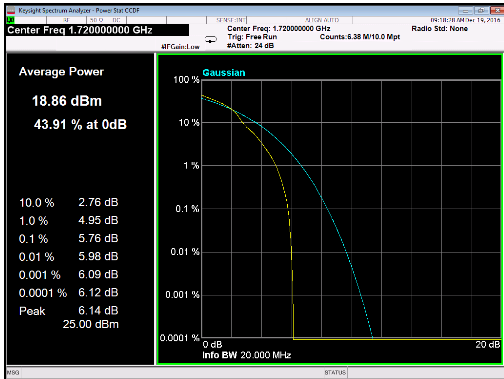
(Plot B1: Band 4/20MHz/16QAM in L Ch 1RB Size)
