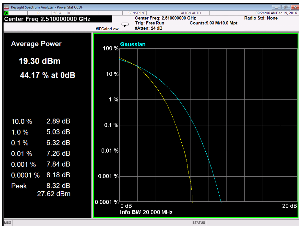
(Plot C2: Band 7/20MHz/16QAM in L Ch 100RB Size)
