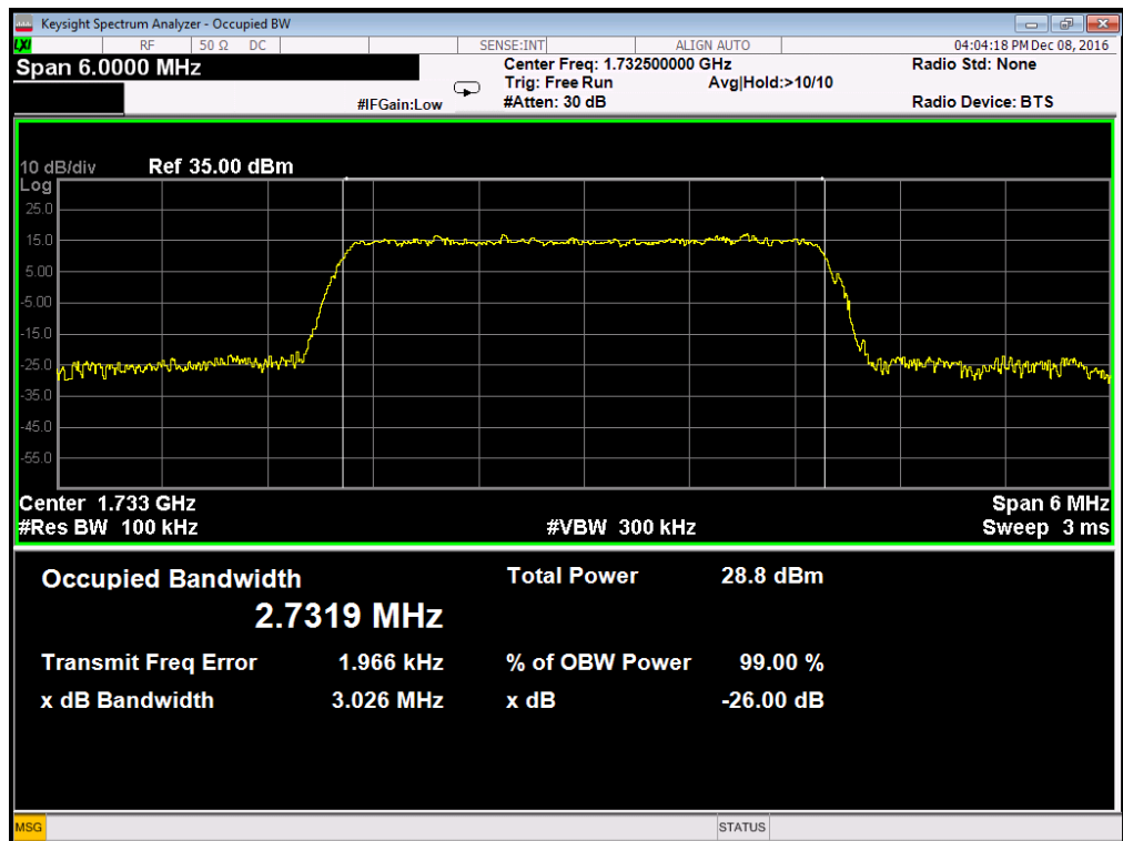
Occupied Bandwidth LTE Band 4/3MHz/QPSK
