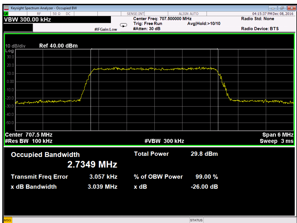
Occupied Bandwidth LTE Band 12/3MHz/16QAM
