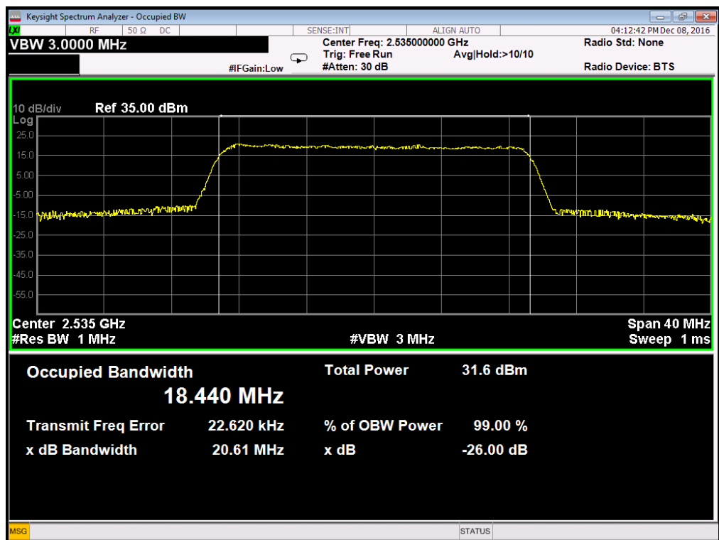
Occupied Bandwidth LTE Band 7/20MHz/QPSK
