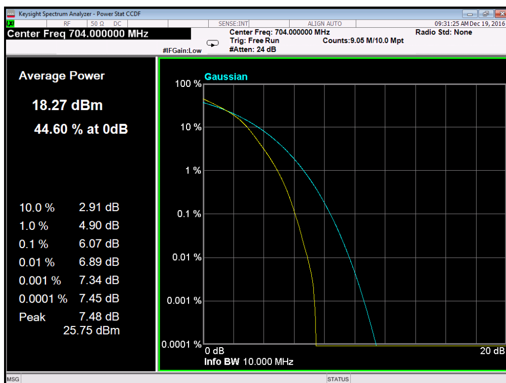
(Plot D2: Band 12/10MHz/16QAM in L Ch 50RB Size)
