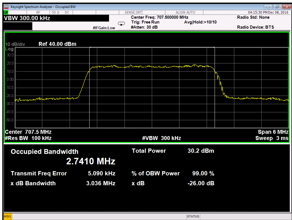
Occupied Bandwidth LTE Band 12/3MHz/QPSK
