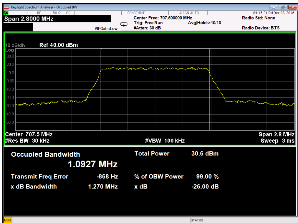
Occupied Bandwidth LTE Band 12/1.4MHz/16QAM
