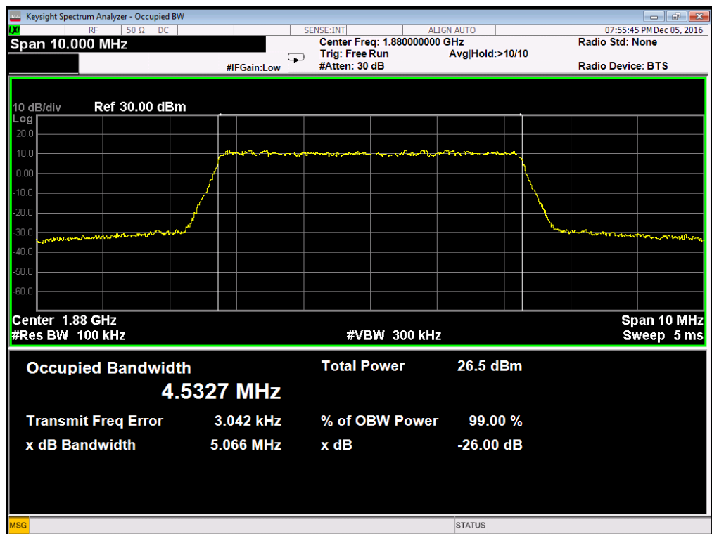
Occupied Bandwidth LTE Band 2/5MHz/QPSK
