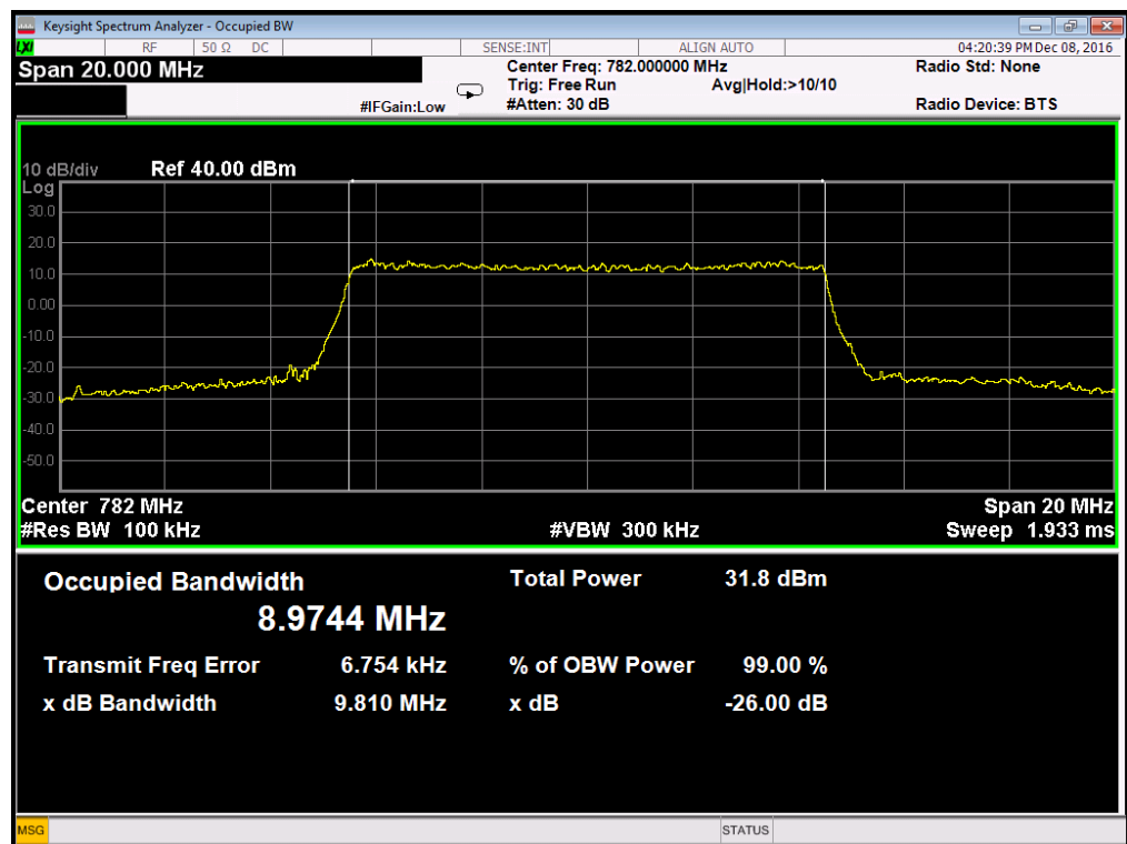
Occupied Bandwidth LTE Band 13/10MHz/QPSK
