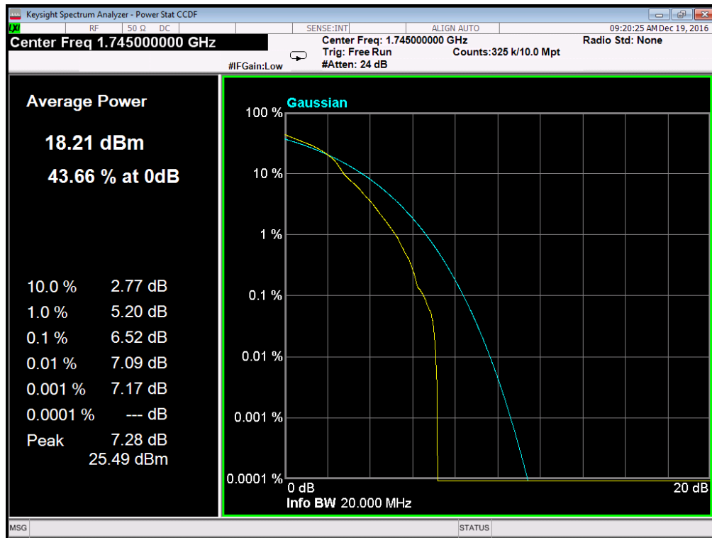
(Plot B5: Band 4/20MHz/16QAM in H Ch 1RB Size)
