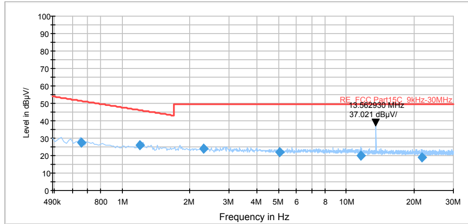
FCC RE 490K-30MHz QP
