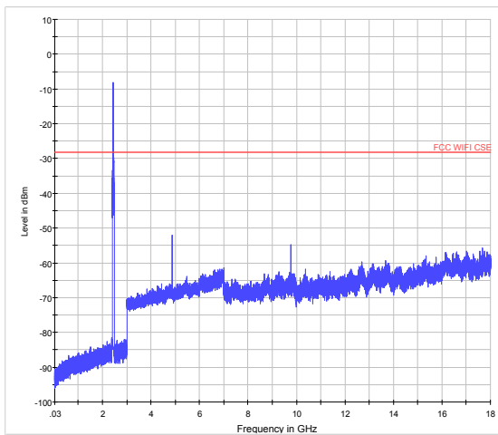
GFSK-CH39 30MHz to 18GHz
