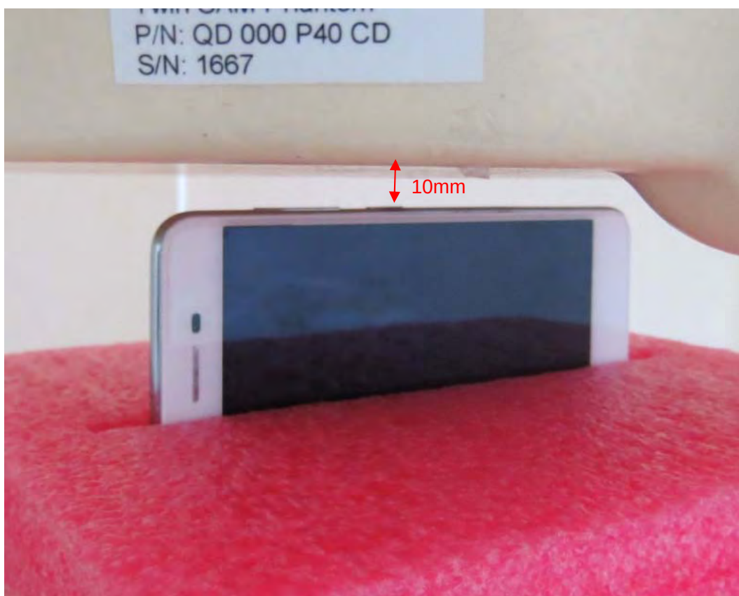
Picture 17: Right Side, the distance from handset to the bottom of the Phantom is 10mm
