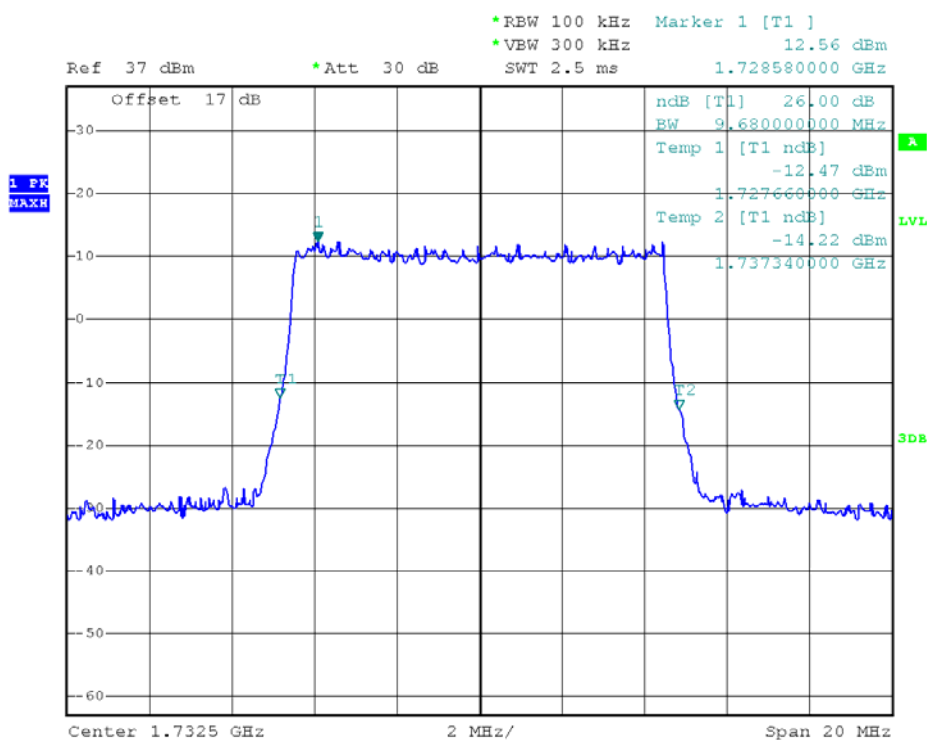
(Plot J4: 26dB Bandwidth LTE Band 4/10MHz/16QAM)
