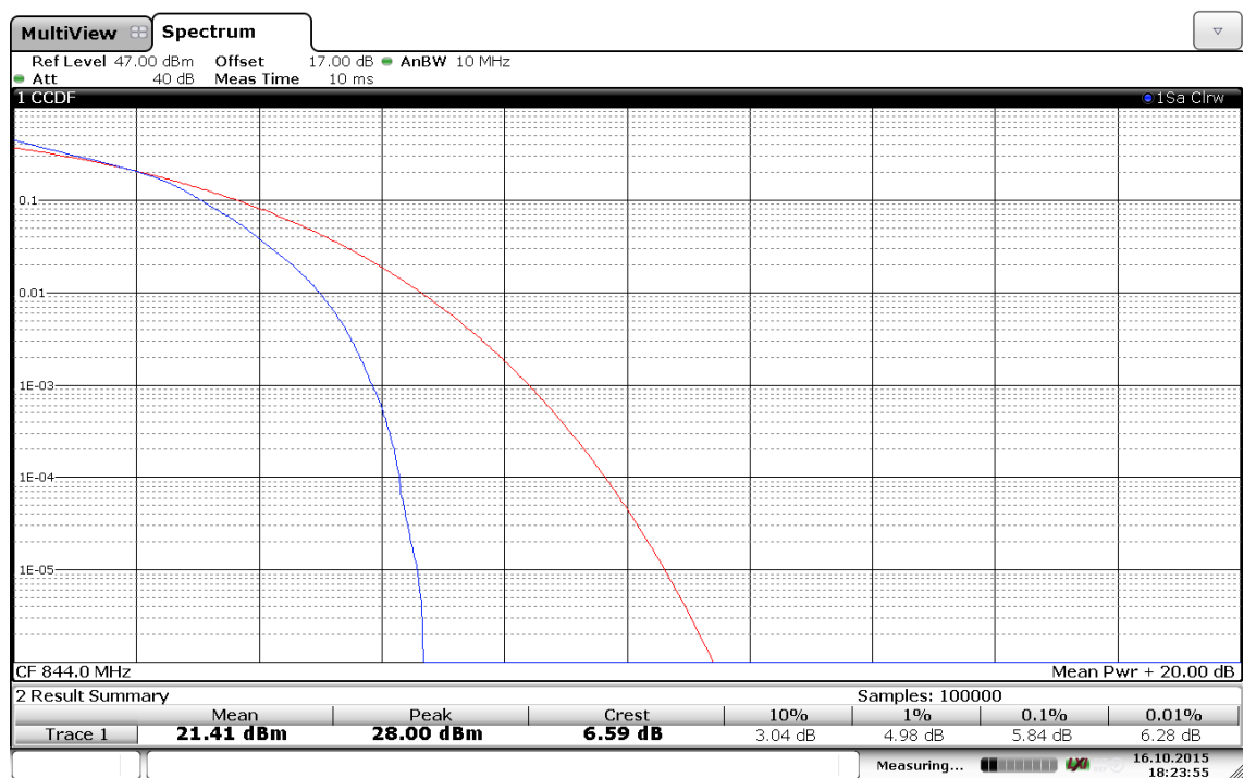
(Plot C5: Band 5/10MHz/16QAM in Ch.20600 1RB Size)
