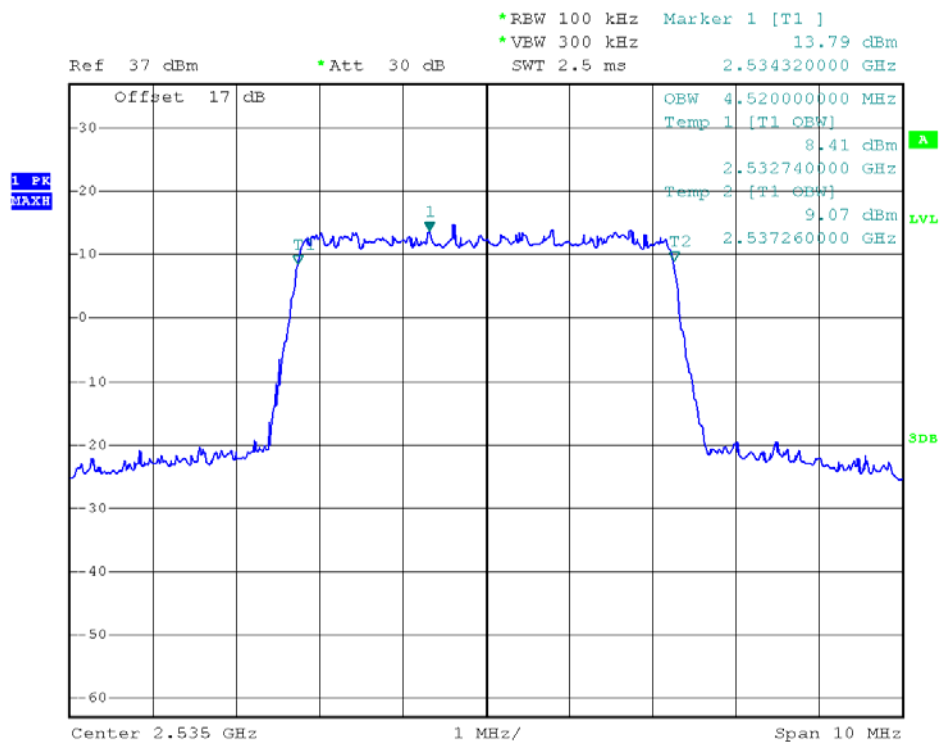
(Plot Q3: 99% Occupied Bandwidth LTE Band 7/5MHz/16QAM)
