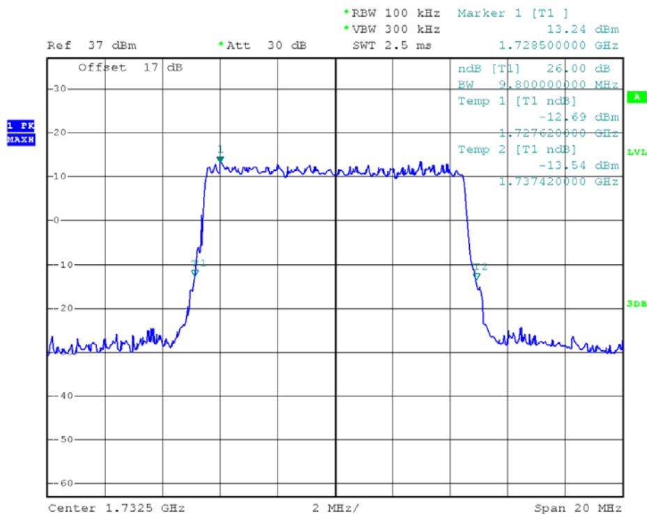
(Plot J2: 26dB Bandwidth LTE Band 4/10MHz/QPSK)
