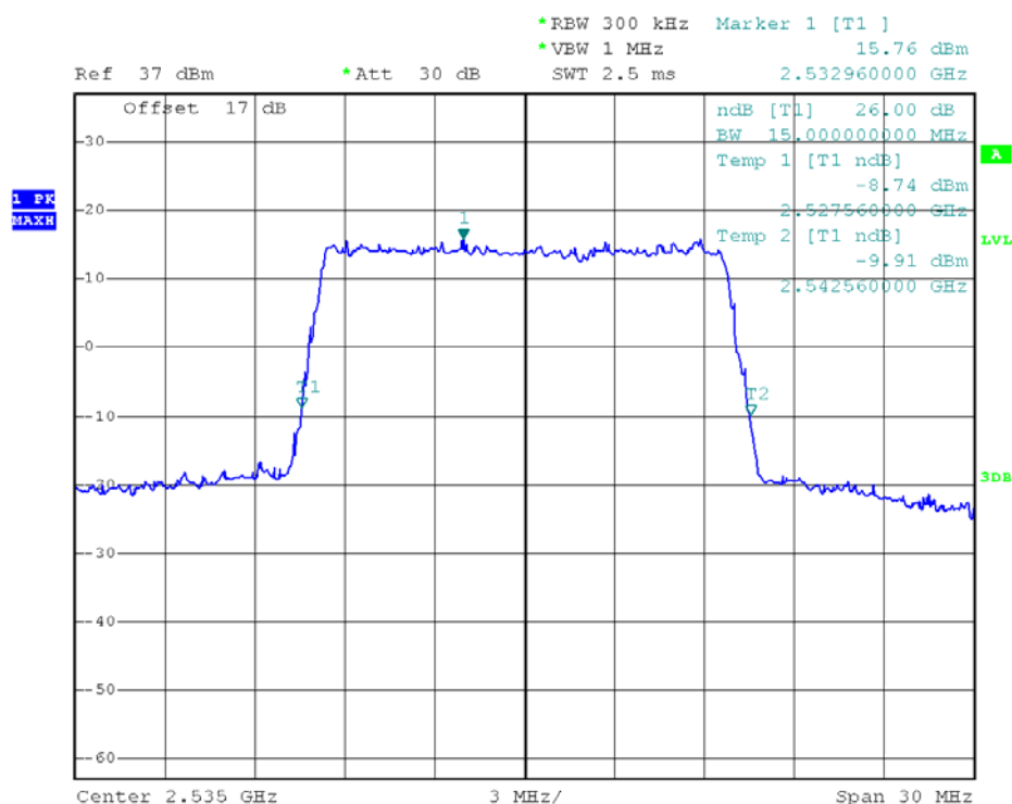
(Plot S2: 26dB Bandwidth LTE Band 7/15MHz/QPSK)
