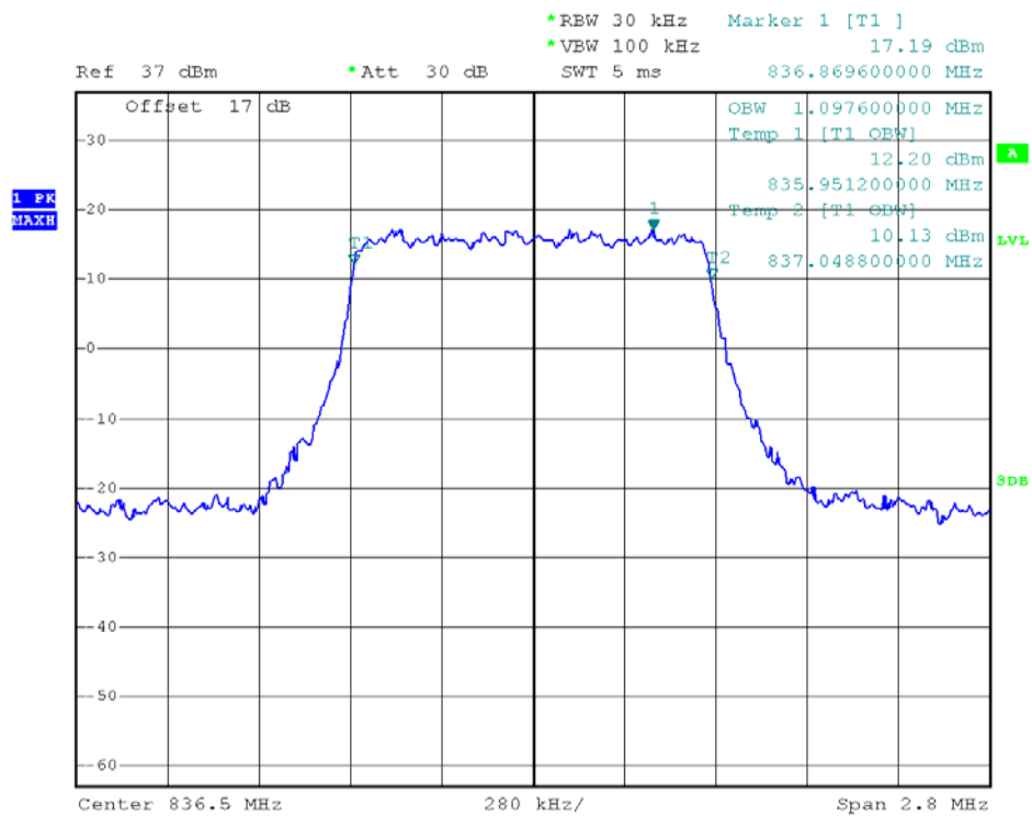
(Plot M1: 99% Occupied Bandwidth LTE Band 5/1.4MHz/QPSK)
