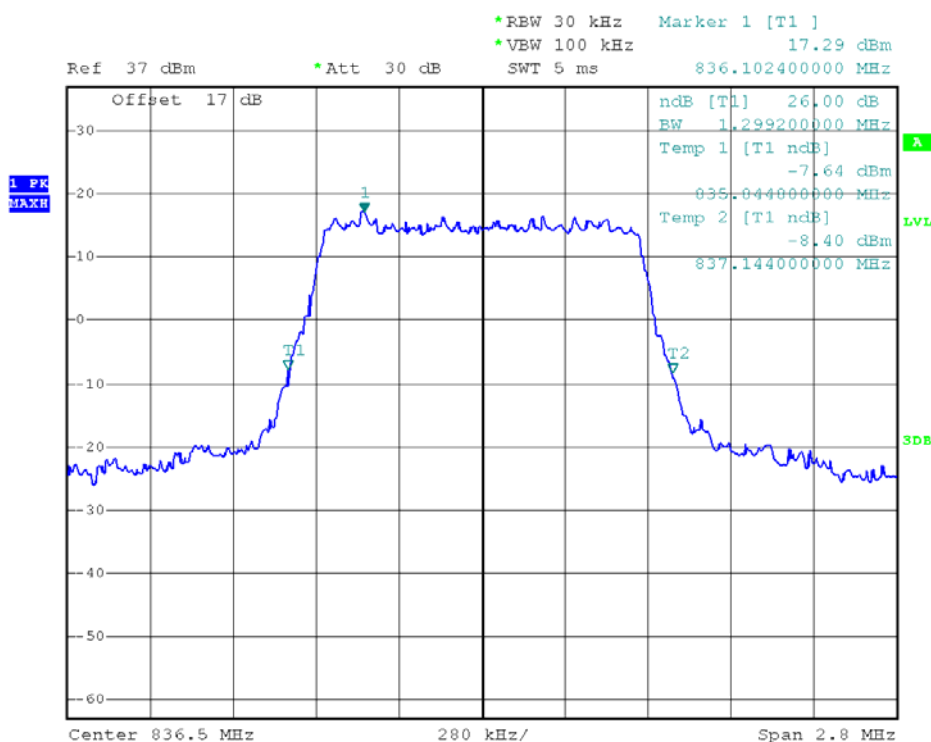
(Plot M4: 26dB Bandwidth LTE Band 5/1.4MHz/16QAM)
