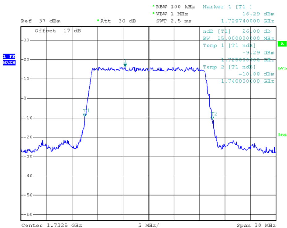
(Plot K2: 26dB Bandwidth LTE Band 4/15MHz/QPSK)
