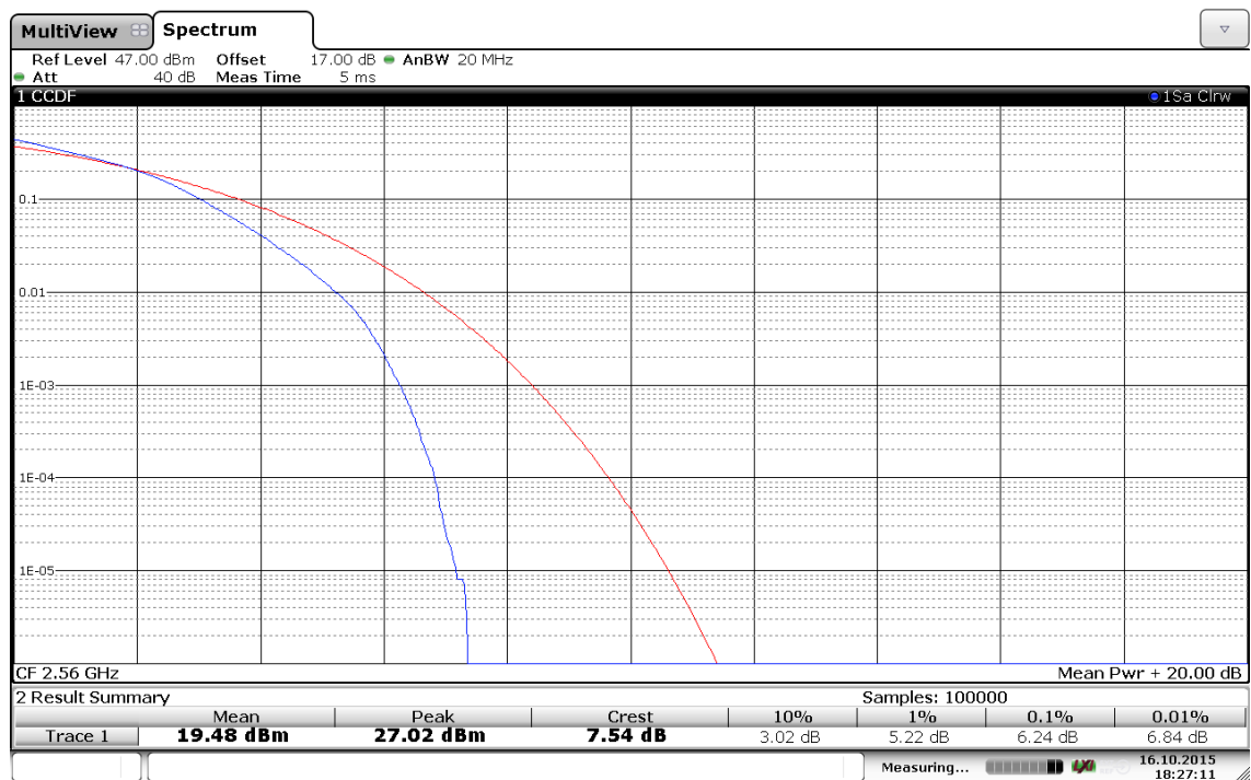
(Plot D5: Band 7/20MHz/16QAM in Ch.21350 1RB Size)
