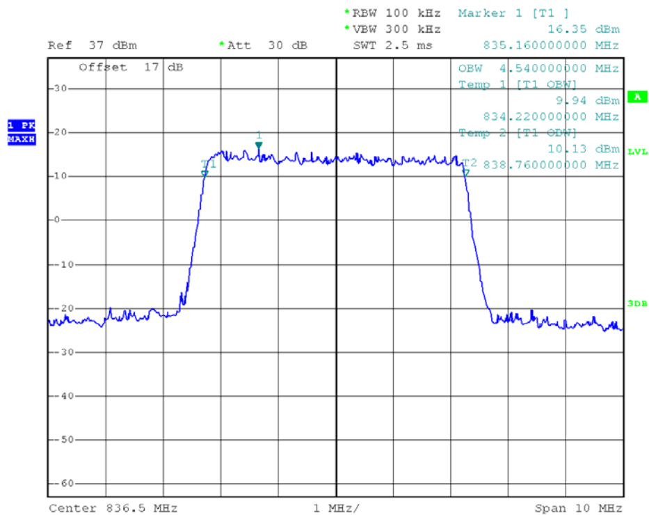
(Plot O3: 99% Occupied Bandwidth LTE Band 5/5MHz/16QAM)
