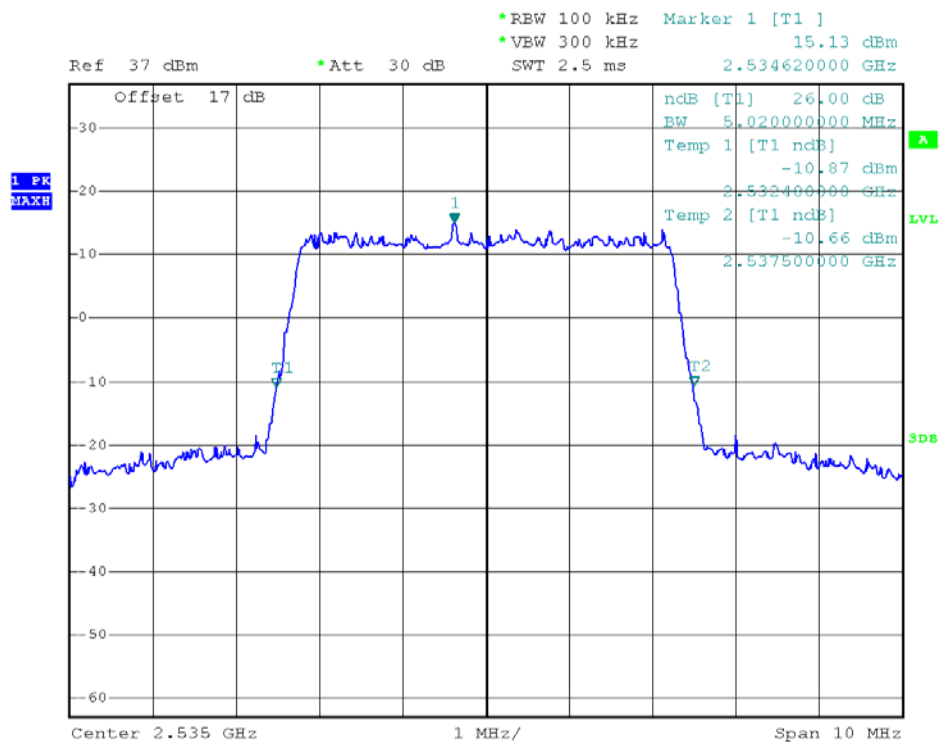
(Plot Q4: 26dB Bandwidth LTE Band 7/5MHz/16QAM)
