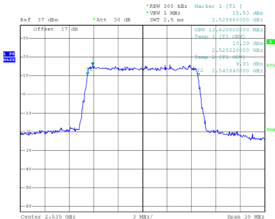
(Plot S1: 99% Occupied Bandwidth LTE Band 7/15MHz/QPSK)
