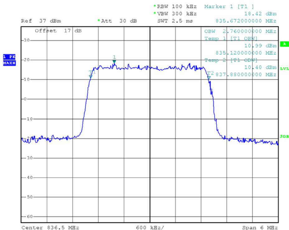
(Plot N3: 99% Occupied Bandwidth LTE Band 5/3MHz/16QAM)
