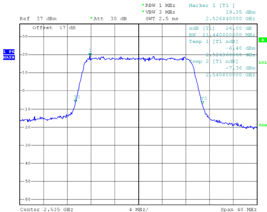
(Plot T2: 26dB Bandwidth LTE Band 7/20MHz/QPSK)
