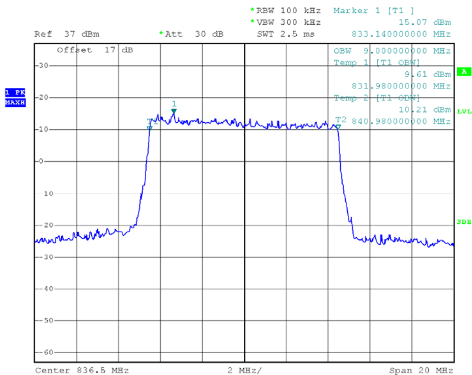
(Plot P1: 99% Occupied Bandwidth LTE Band 5/10MHz/QPSK)
