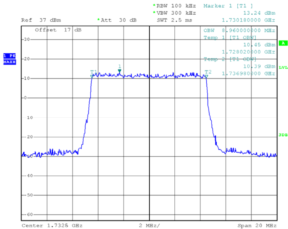
(Plot J1: 99% Occupied Bandwidth LTE Band 4/10MHz/QPSK)
