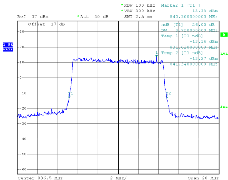
(Plot P4: 26dB Bandwidth LTE Band 5/10MHz/16QAM)
