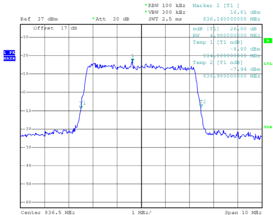
(Plot O4: 26dB Bandwidth LTE Band 5/5MHz/16QAM)
