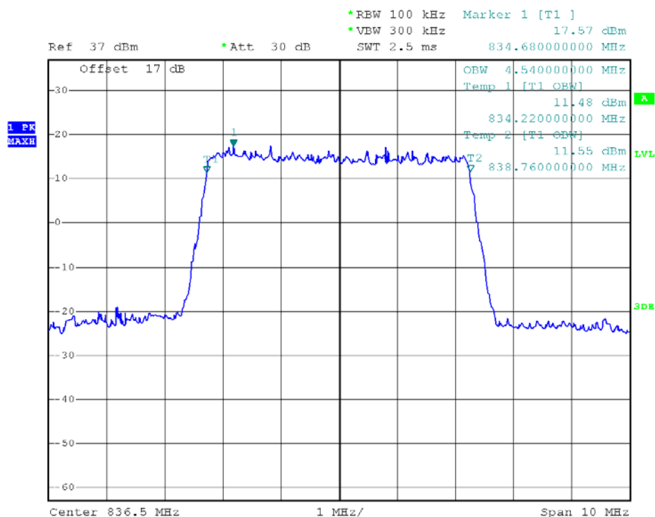
(Plot O1: 99% Occupied Bandwidth LTE Band 5/5MHz/QPSK)
