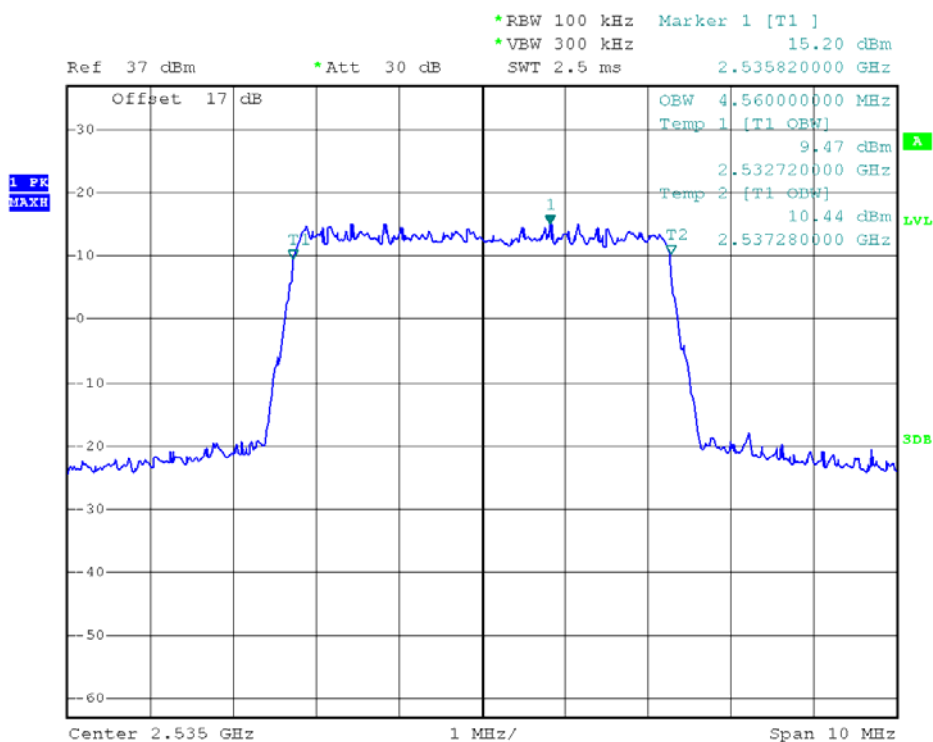
(Plot Q1: 99% Occupied Bandwidth LTE Band 7/5MHz/QPSK)
