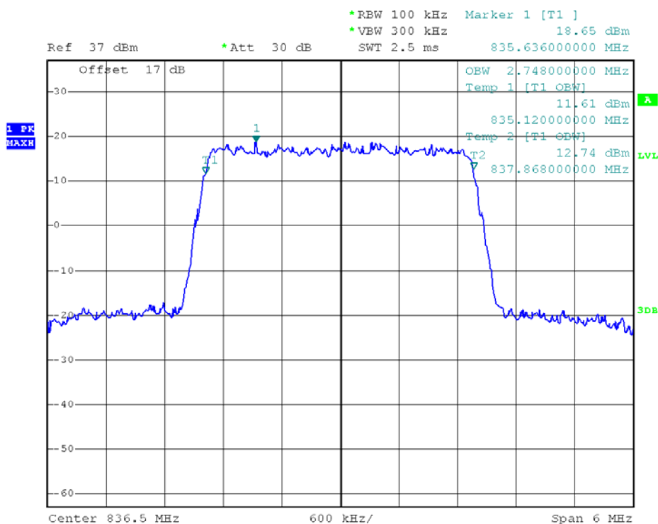
(Plot N1: 99% Occupied Bandwidth LTE Band 5/3MHz/QPSK)
