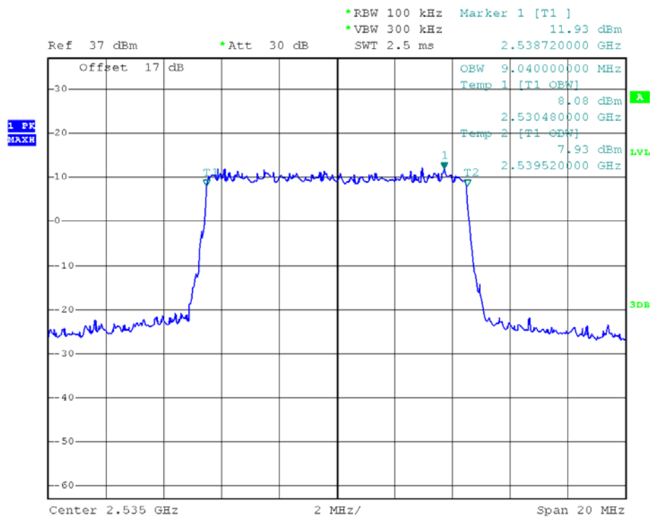
(Plot R1: 99% Occupied Bandwidth LTE Band 7/10MHz/QPSK)
