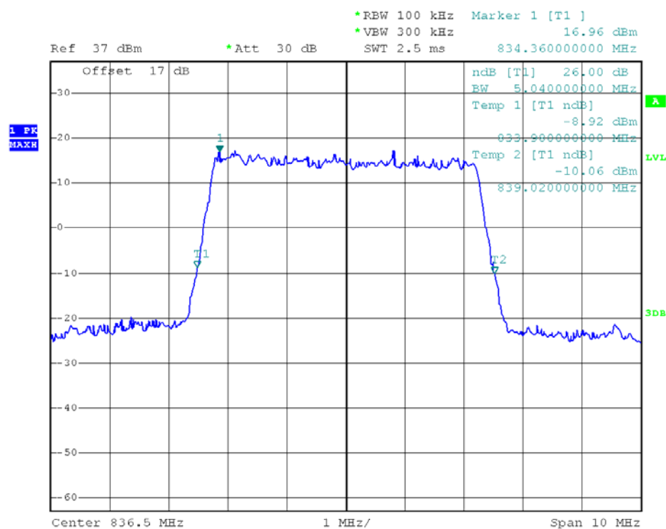
(Plot O2: 26dB Bandwidth LTE Band 5/5MHz/QPSK)
