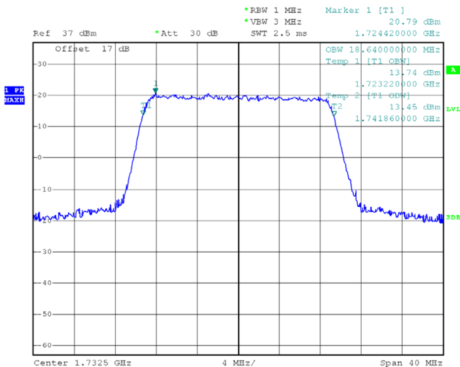
(Plot L1: 99% Occupied Bandwidth LTE Band 4/20MHz/QPSK)
