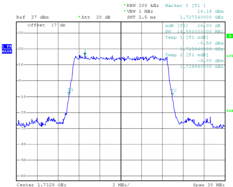
(Plot K4: 26dB Bandwidth LTE Band 4/15MHz/16QAM)
