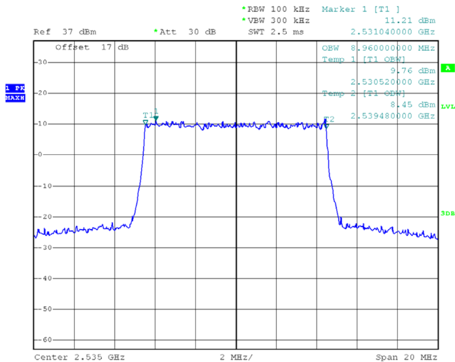
(Plot R3: 99% Occupied Bandwidth LTE Band 7/10MHz/16QAM)
