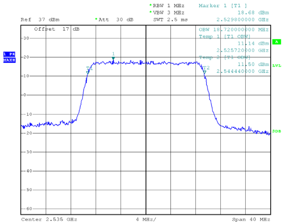
(Plot T3: 99% Occupied Bandwidth LTE Band 7/20MHz/16QAM)
