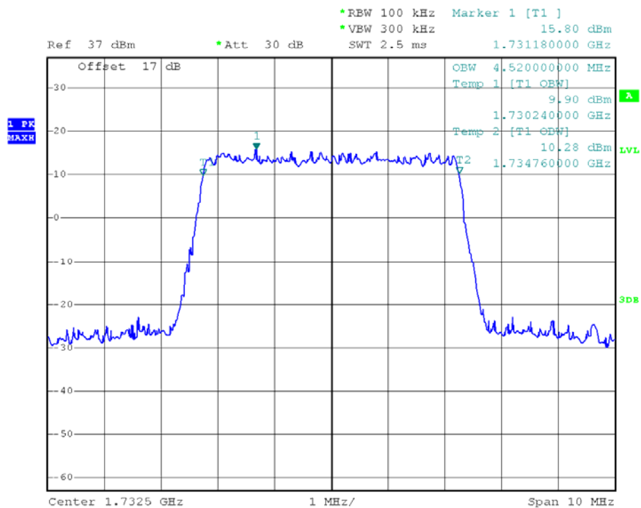
(Plot I3: 99% Occupied Bandwidth LTE Band 4/5MHz/16QAM)
