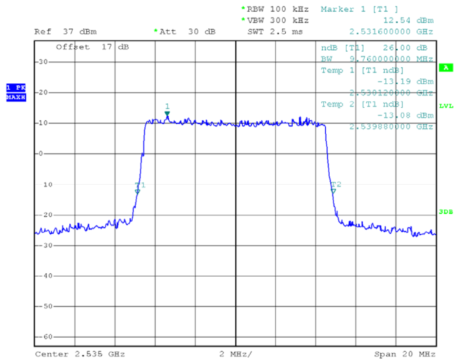
(Plot R2: 26dB Bandwidth LTE Band 7/10MHz/QPSK)
