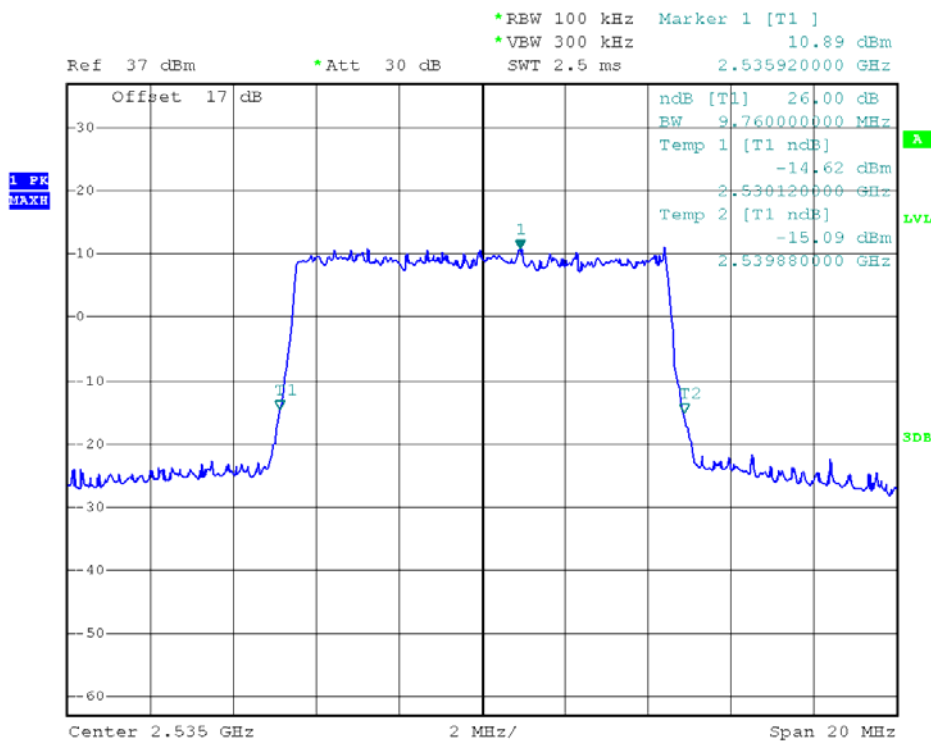
(Plot R4: 26dB Bandwidth LTE Band 7/10MHz/16QAM)
