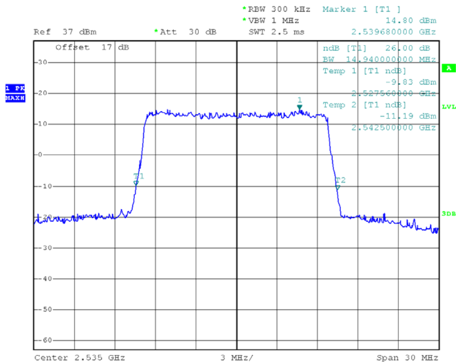
(Plot S4: 26dB Bandwidth LTE Band 7/15MHz/16QAM)
