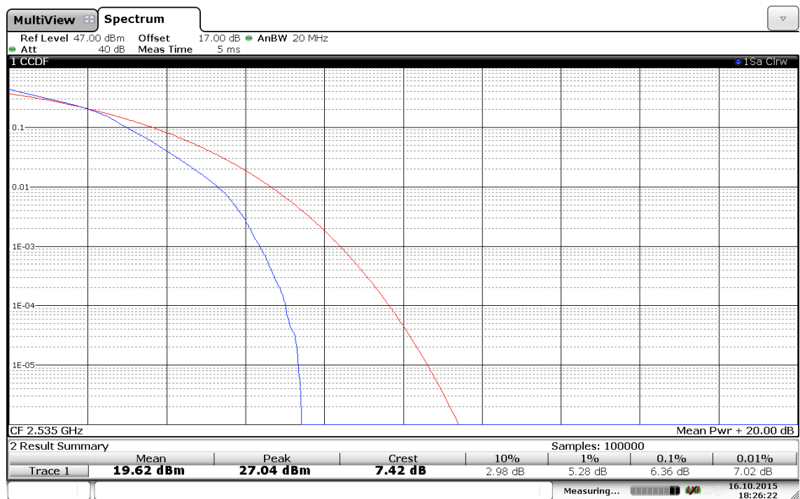
(Plot D3: Band 7/20MHz/16QAM in Ch.21100 1RB Size)
