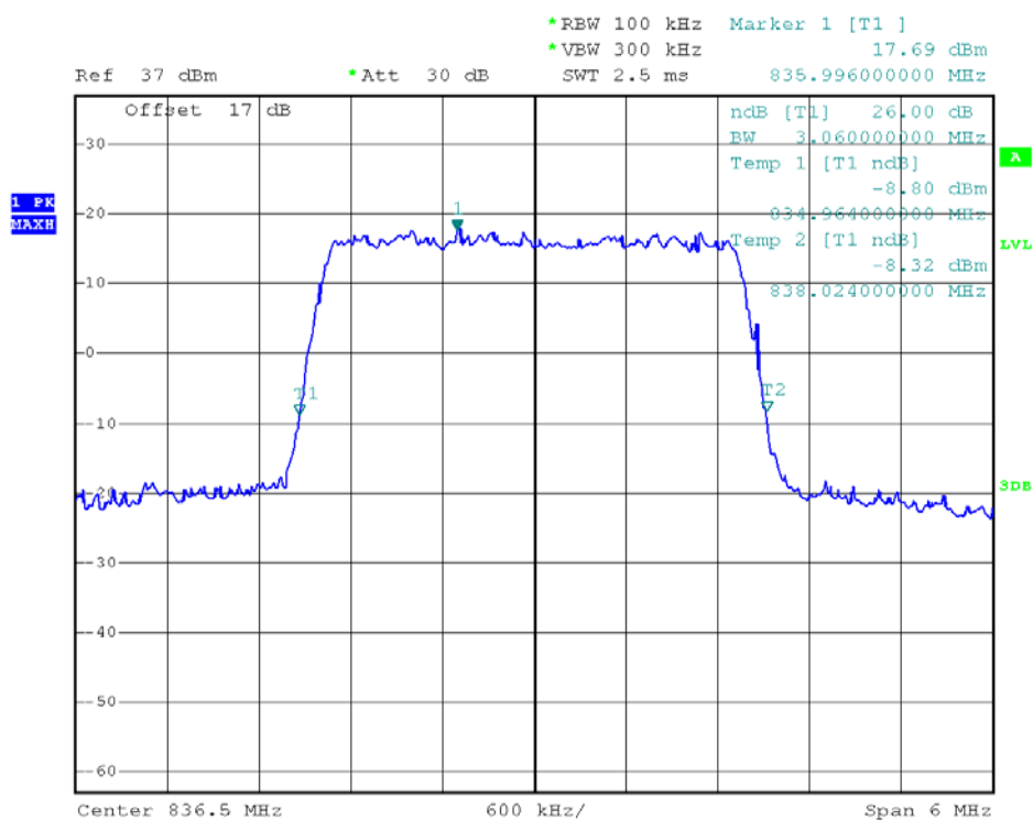
(Plot N4: 26dB Bandwidth LTE Band 5/3MHz/16QAM)
