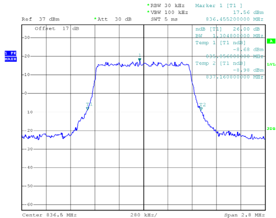
(Plot M2: 26dB Bandwidth LTE Band 5/1.4MHz/QPSK)
