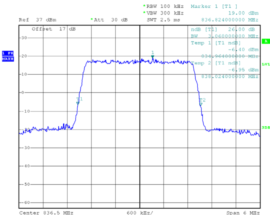
(Plot N2: 26dB Bandwidth LTE Band 5/3MHz/QPSK)
