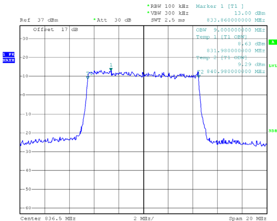
(Plot P3: 99% Occupied Bandwidth LTE Band 5/10MHz/16QAM)
