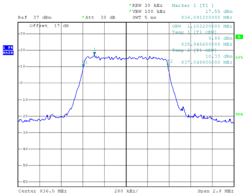
(Plot M3: 99% Occupied Bandwidth LTE Band 5/1.4MHz/16QAM)
