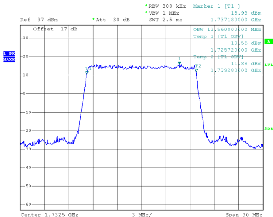
(Plot K3: 99% Occupied Bandwidth LTE Band 4/15MHz/16QAM)
