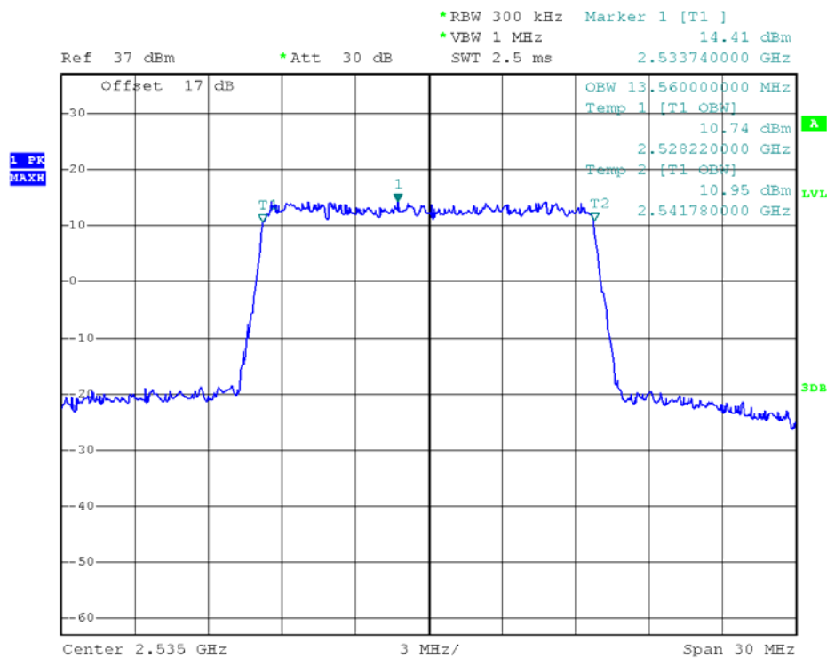
(Plot S3: 99% Occupied Bandwidth LTE Band 7/15MHz/16QAM)
