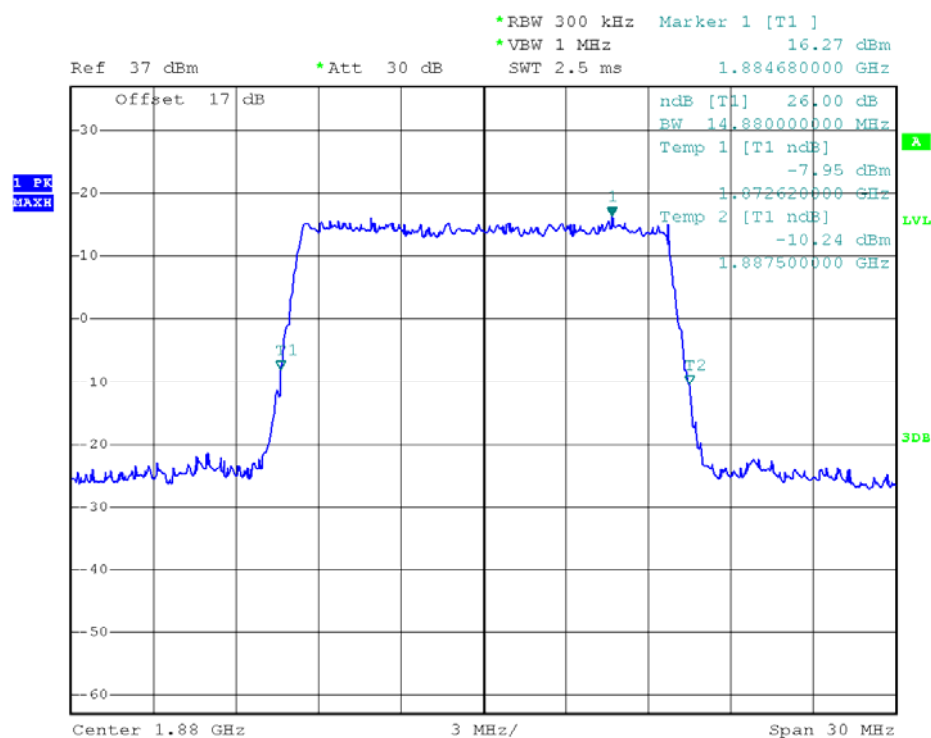
(Plot E4: 26dB Bandwidth LTE Band 2/15MHz/16QAM)
