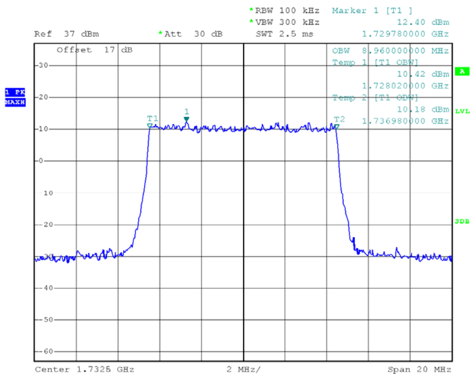
(Plot J3: 99% Occupied Bandwidth LTE Band 4/10MHz/16QAM)
