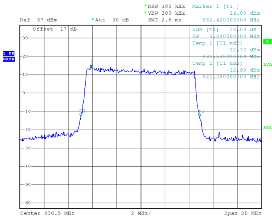
(Plot P2: 26dB Bandwidth LTE Band 5/10MHz/QPSK)
