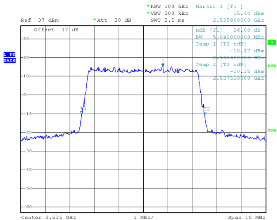
(Plot Q2: 26dB Bandwidth LTE Band 7/5MHz/QPSK)
