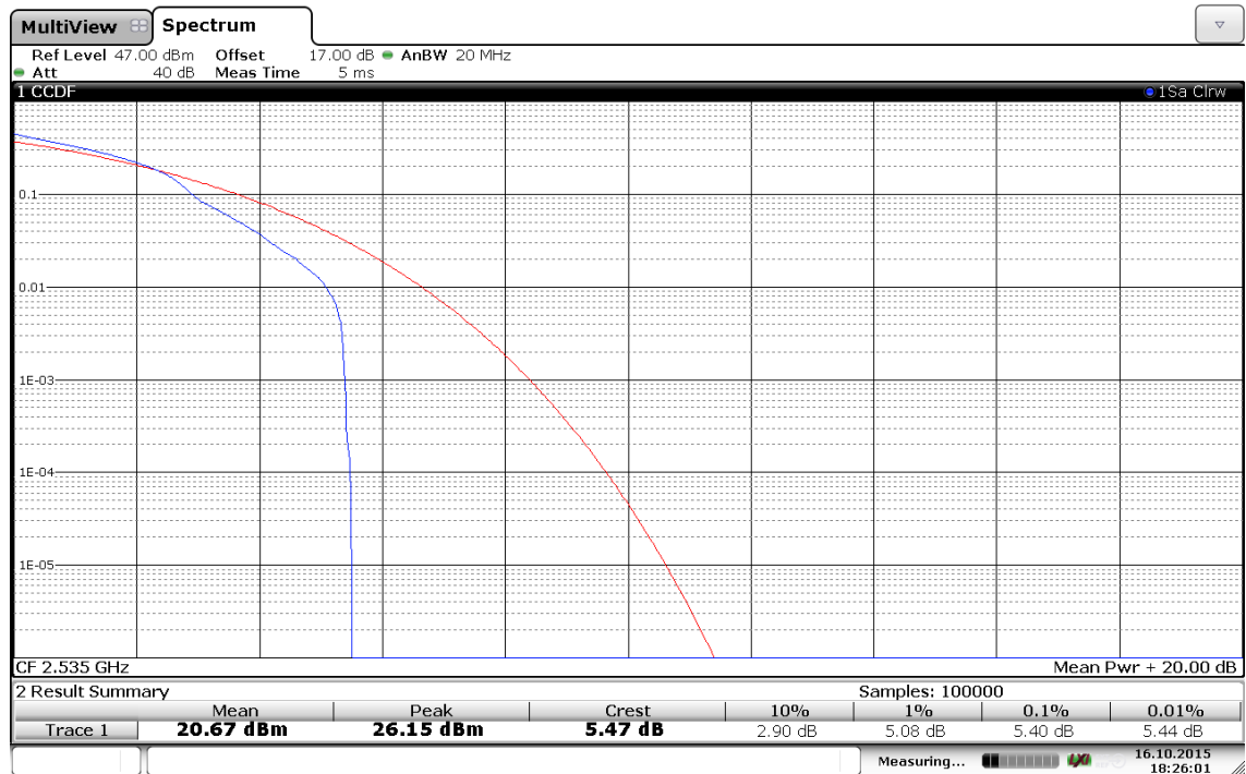
(Plot D3: Band 7/20MHz/16QAM in Ch.21100 1RB Size)
