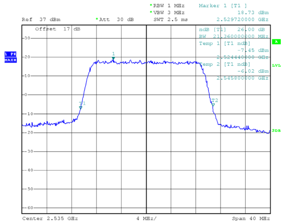
(Plot T4: 26dB Bandwidth LTE Band 7/20MHz/16QAM)
