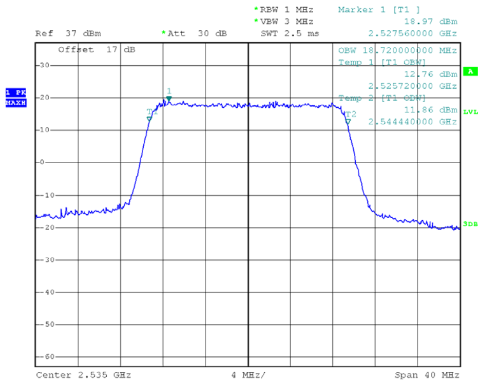
(Plot T1: 99% Occupied Bandwidth LTE Band 7/20MHz/QPSK)
