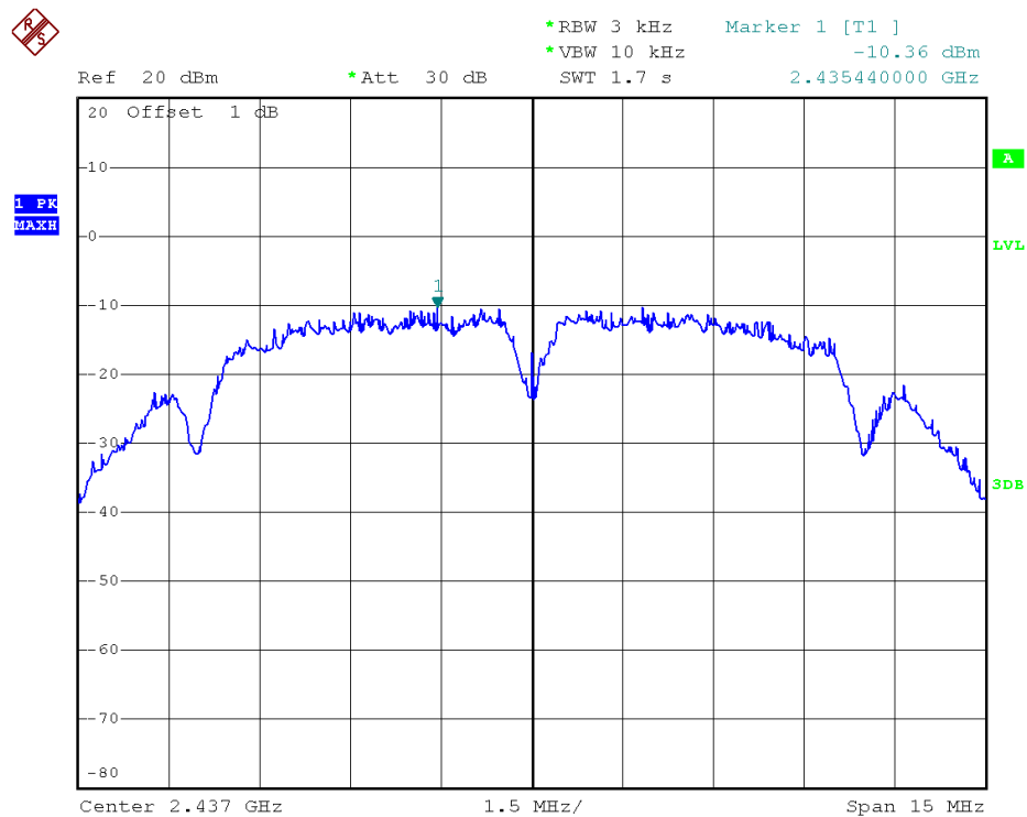
802.11b - Channel 6
