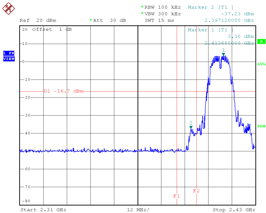
802.11b - Low Band Edge Plot on Channel 1
