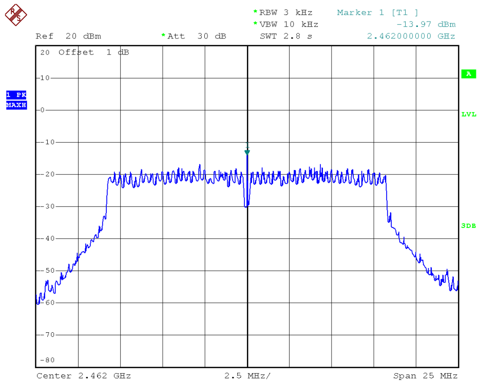
802.11g - Channel 11
