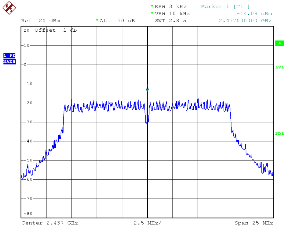
802.11g - Channel 6
