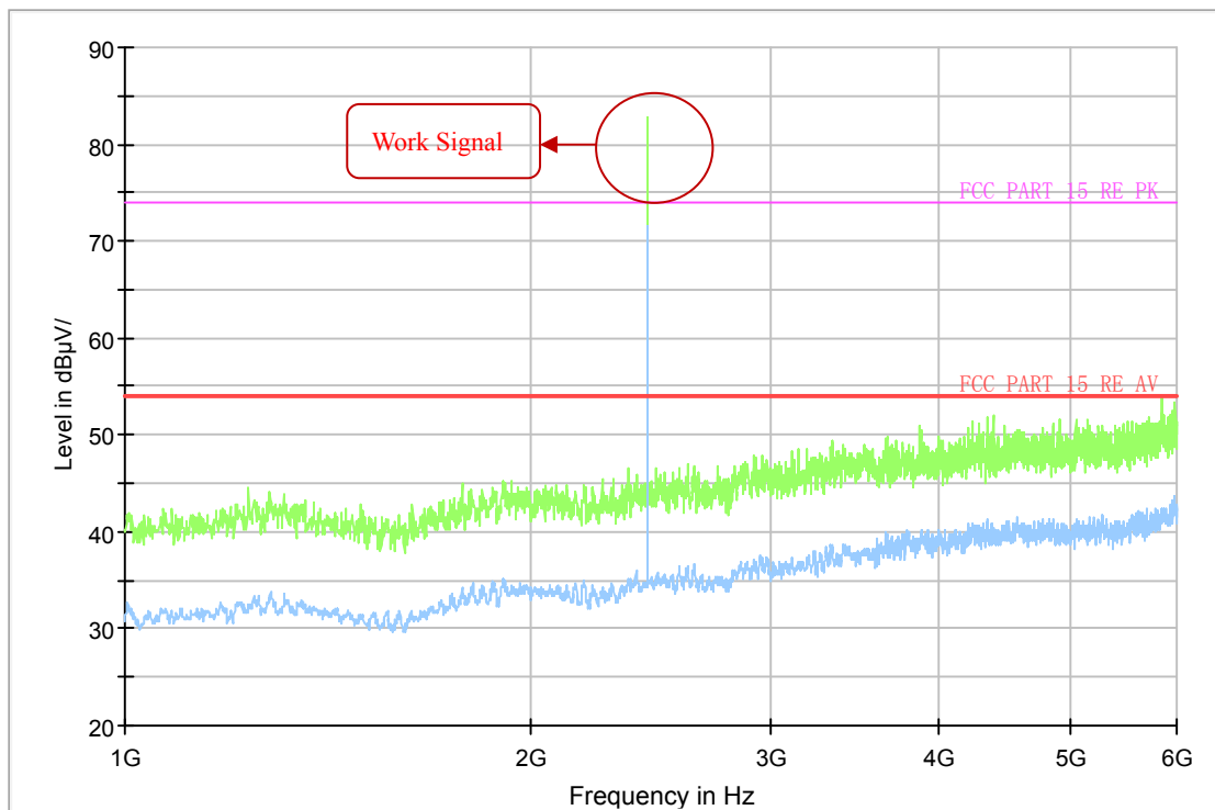
Fig.6 Radiated Emission of channel 39 in 1GHz-6GHz
