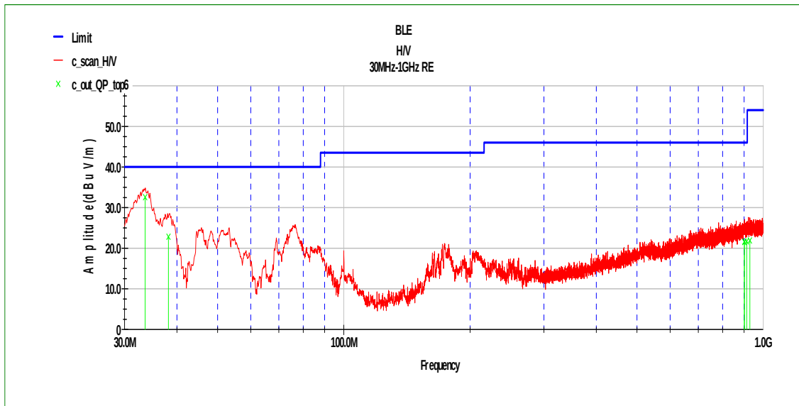
Fig.5 Radiated Emission of channel 39 in 30MHz-1GHz
