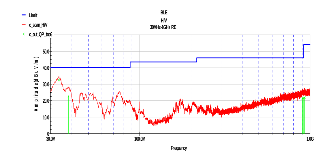
Fig.1 Radiated Emission of channel 0 in 30MHz-1GHz
