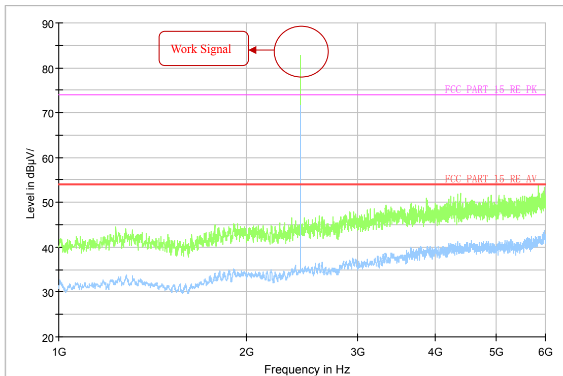
Fig.4 Radiated Emission of channel 19 in 1GHz-6GHz
