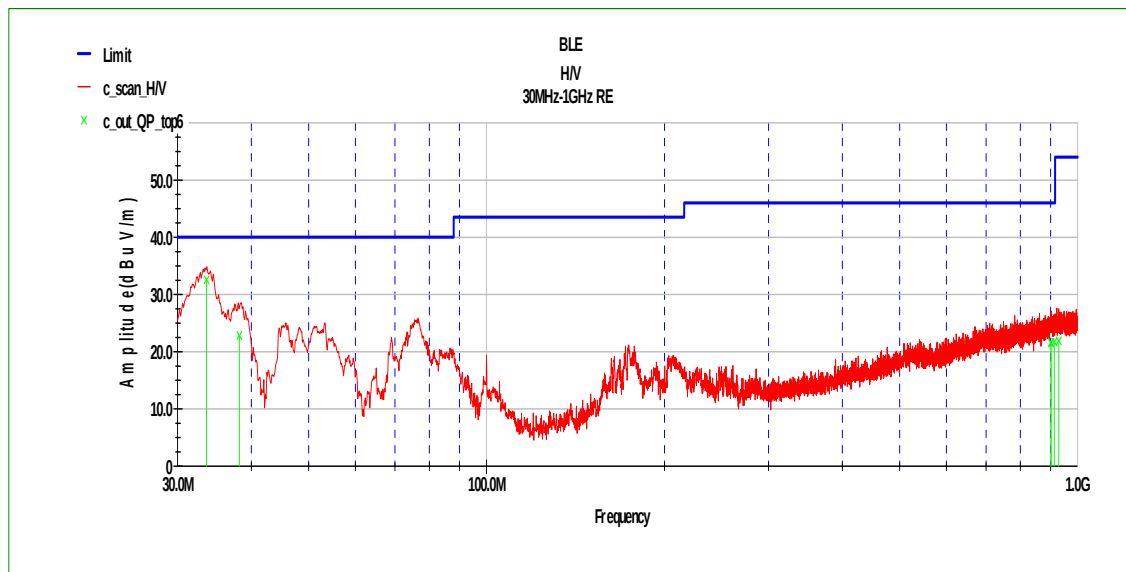
Fig.3 Radiated Emission of channel 19 in 30MHz-1GHz
