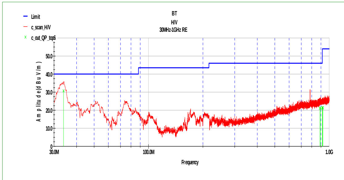
Fig.5 Radiated Emission of channel 78 in 30MHz-1GHz
