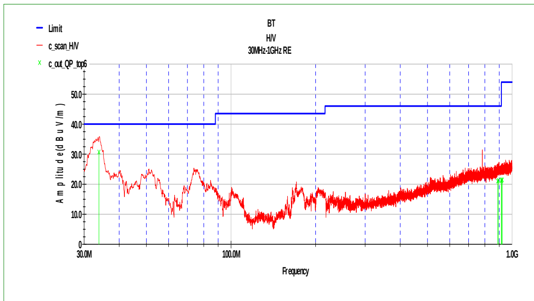
Fig.3 Radiated Emission of channel 39 in 30MHz-1GHz
