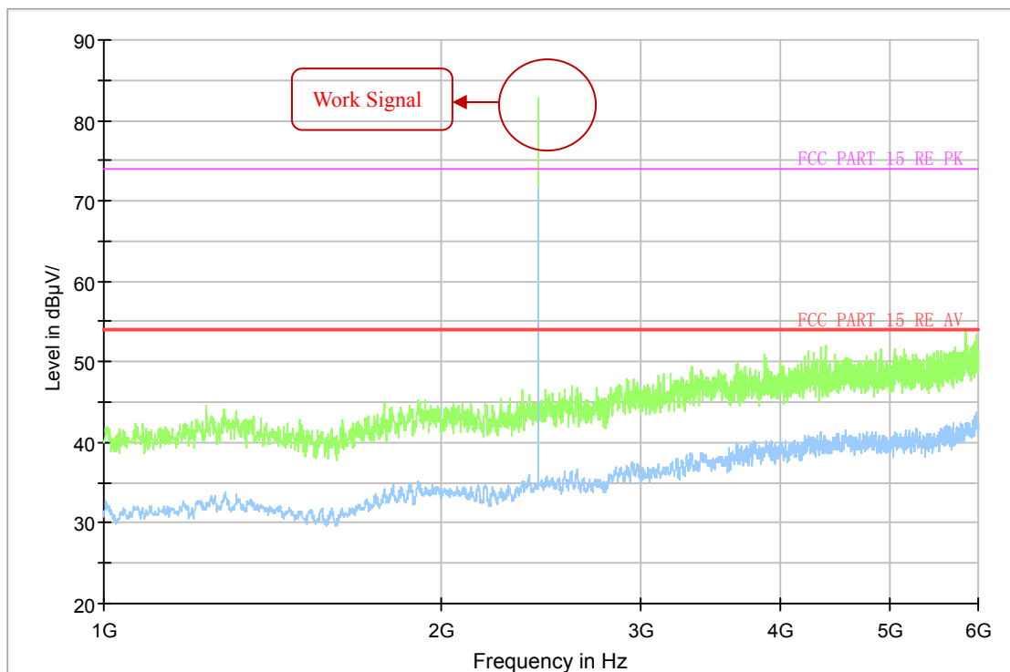
Fig.6 Radiated Emission of channel 78 in 1GHz-6GHz
