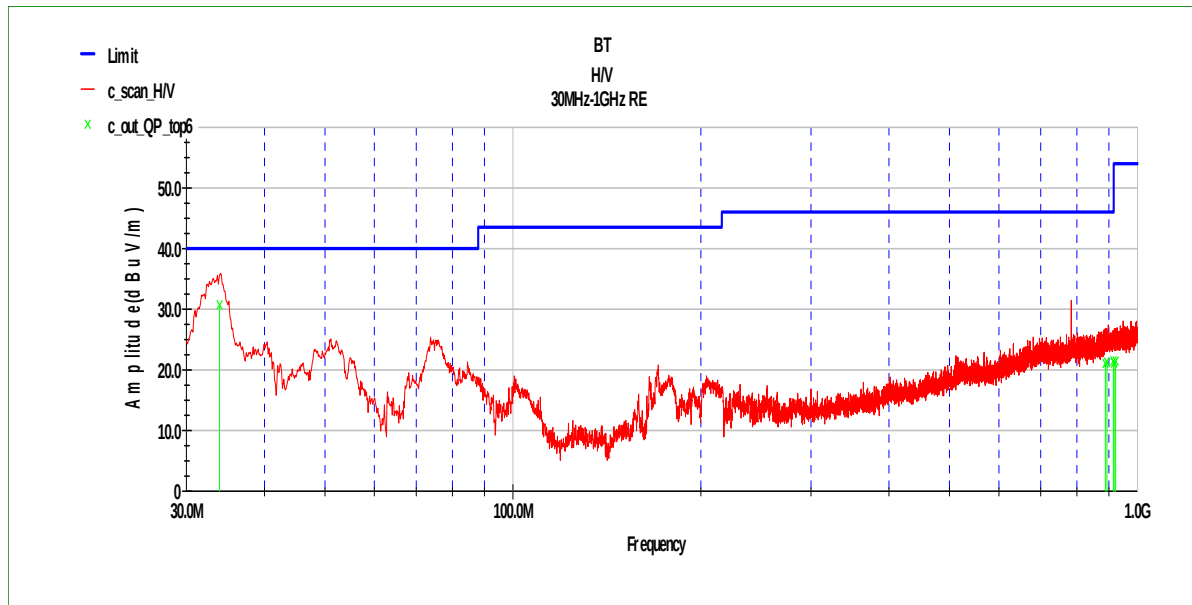
Fig.1 Radiated Emission of channel 0 in 30MHz-1GHz
