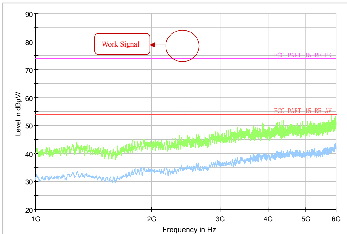
Fig.2 Radiated Emission of channel 0 in 1GHz-6GHz
