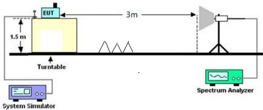
Radiated Emissions Frequency: above 1GHz
