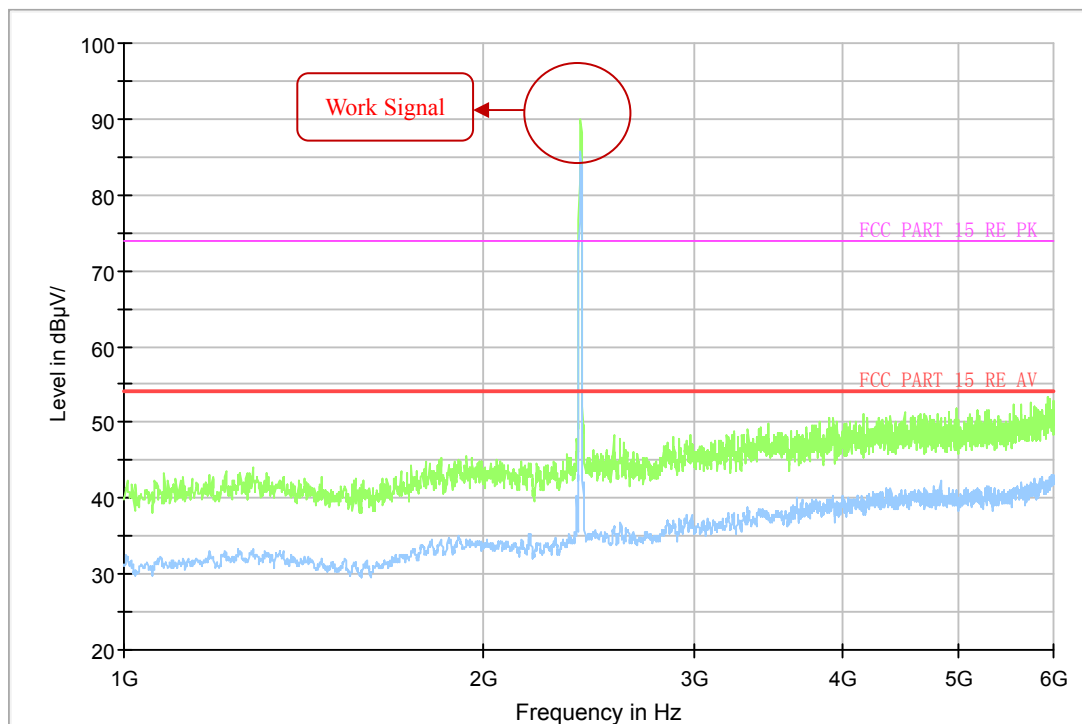
Fig.12 Radiated Emission of channel 1 in 1GHz-6GHz
