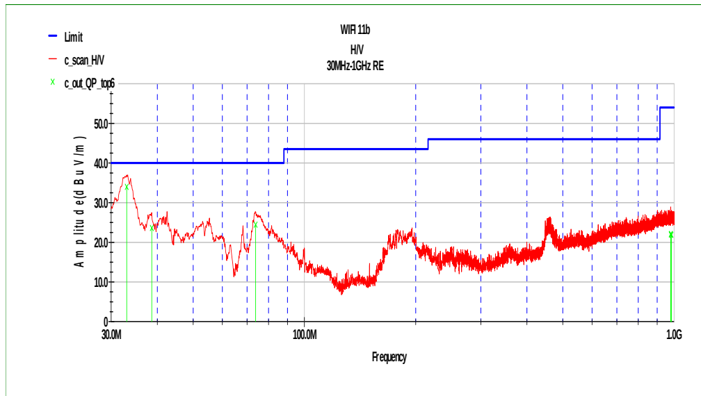
Fig.3 Radiated Emission of channel 6 in 30MHz-1GHz
