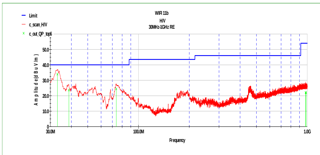
Fig.1 Radiated Emission of channel 1 in 30MHz-1GHz
