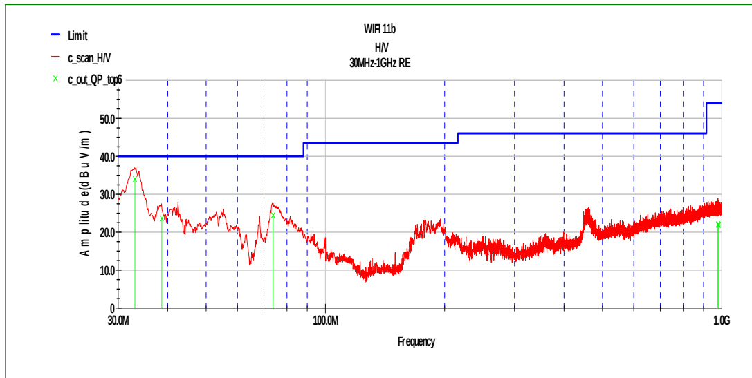
Fig.5 Radiated Emission of channel 11 in 30MHz-1GHz
