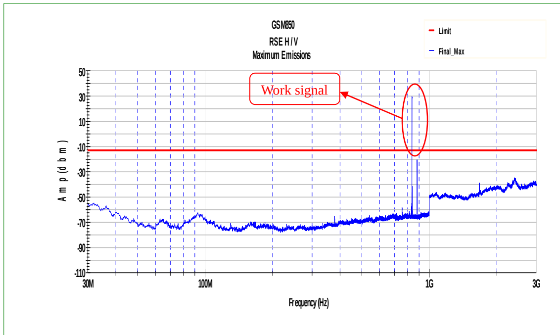
Fig.1 GSM850 on Channel 189 30MHz~3GHz
