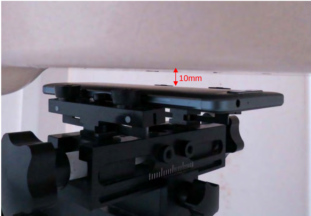
Picture 20: Back Side, the distance from handset to the bottom of the Phantom is 10mm
