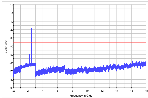
GFSK-CH39 30MHz to 18GHz
