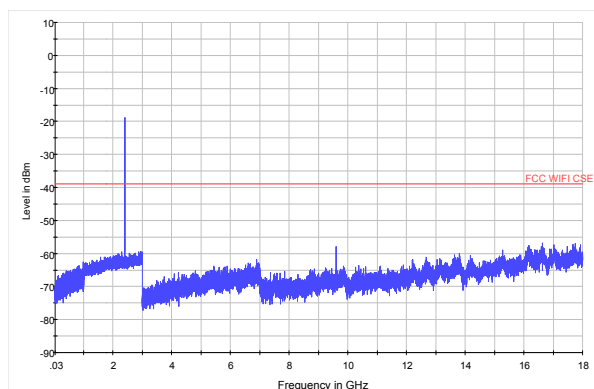
EDR-CH39 30MHz to 18GHz
