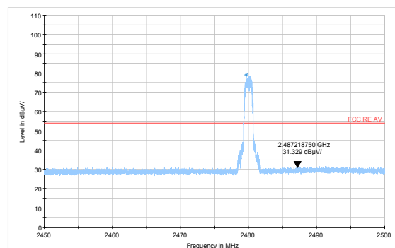
3DH5-Channel 78: Average
