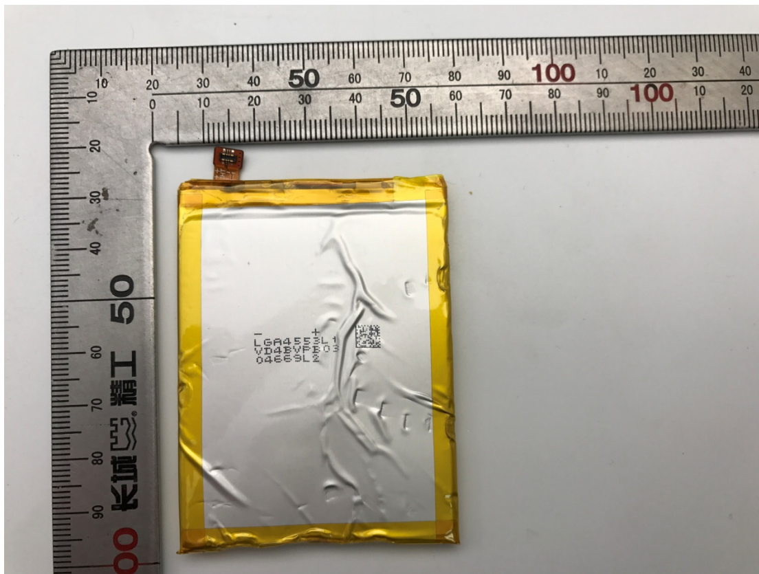
The battery view (Li3928T44P8h475371)
