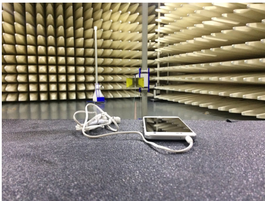
Pic5.Spurious RadiatedEmissions Test setup (1GHz~25GHz)
