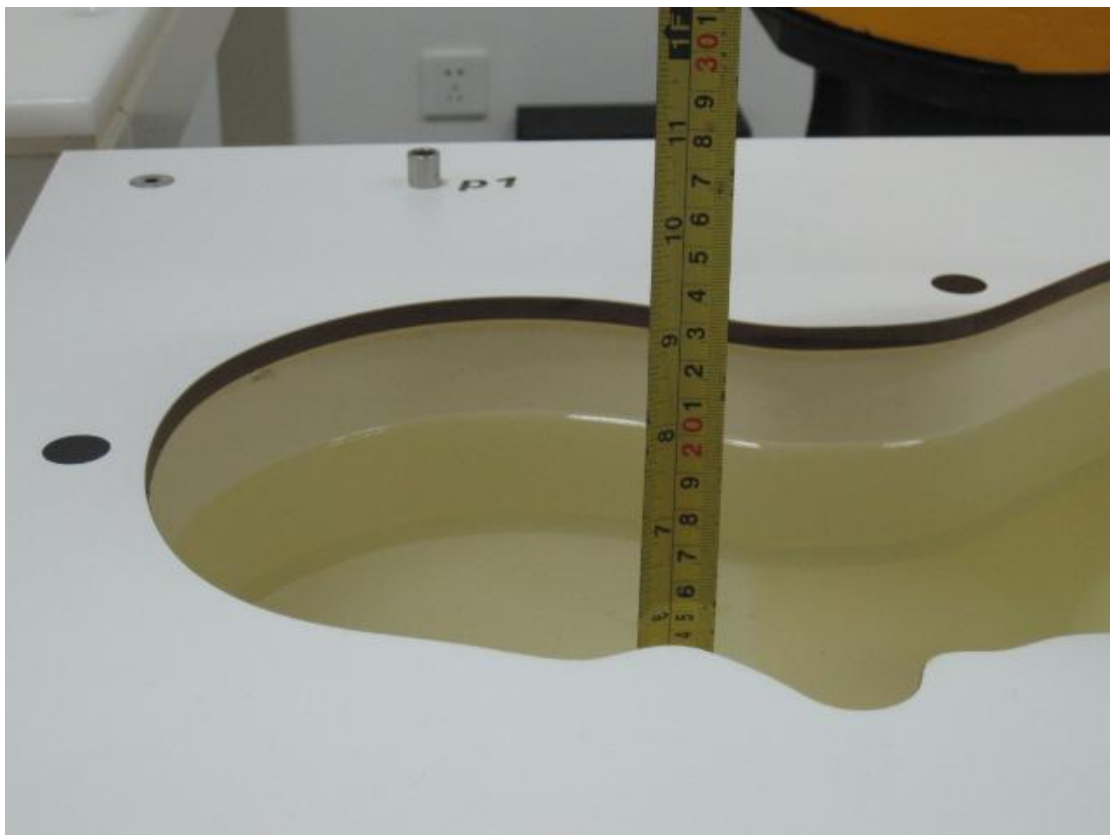
Picture D 12: Liquid depth in the head Phantom (750MHz) (15.4cm deep)
