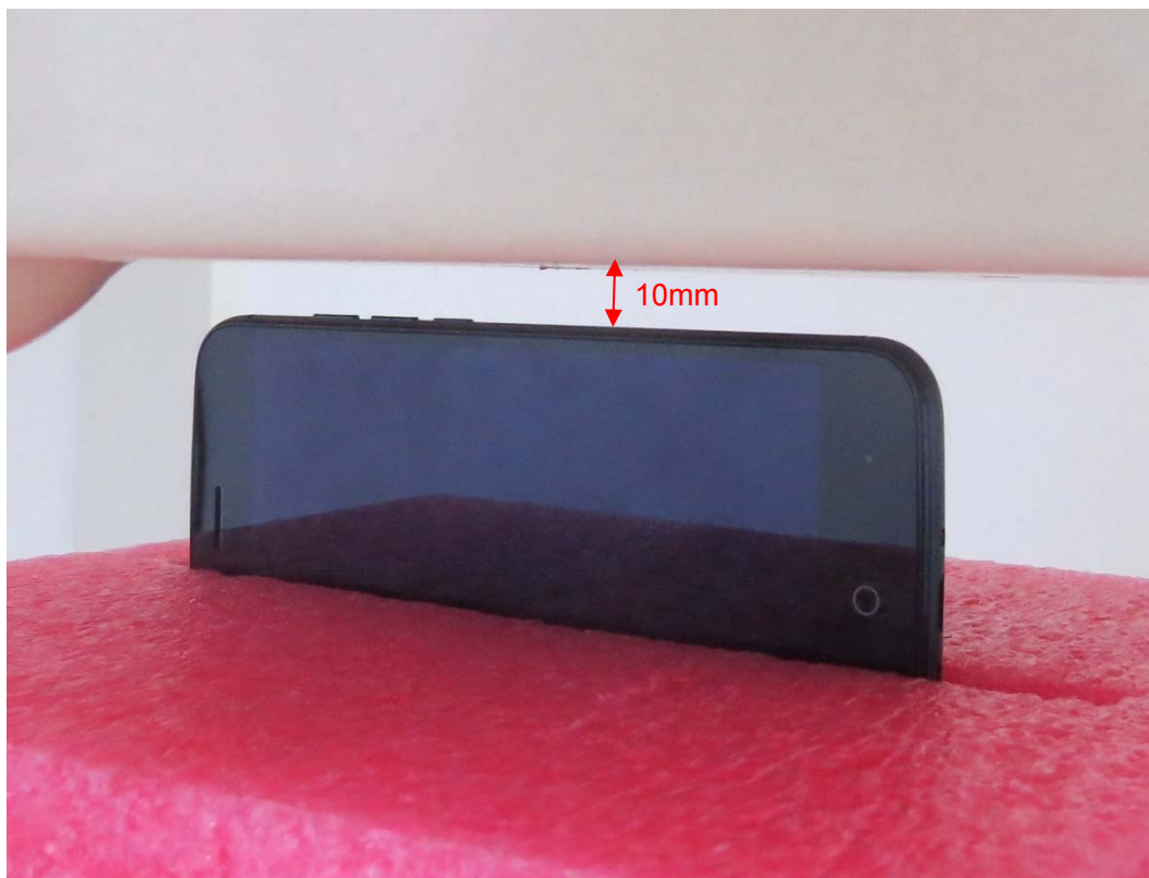
Picture 13: Right Side, the distance from handset to the bottom of the Phantom is 10mm
