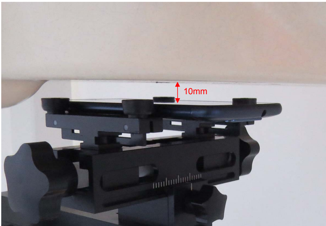
Picture 11: Front Side, the distance from handset to the bottom of the Phantom is 10mm
