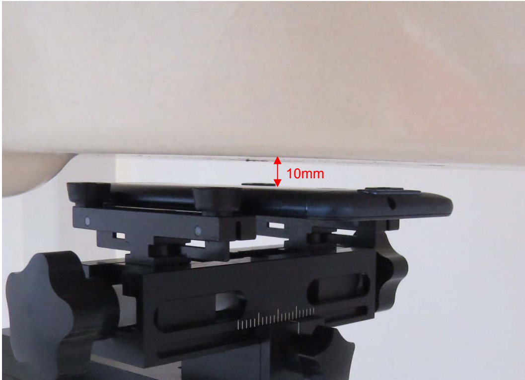
Picture 10: Back Side, the distance from handset to the bottom of the Phantom is 10mm
