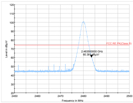
DH5-Channel 78: Peak
