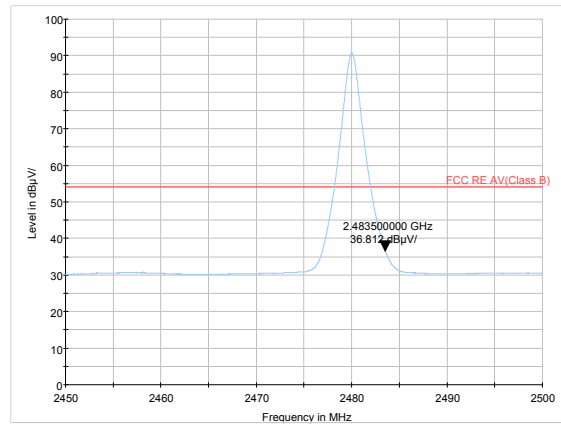
DH5-Channel 78: Average
