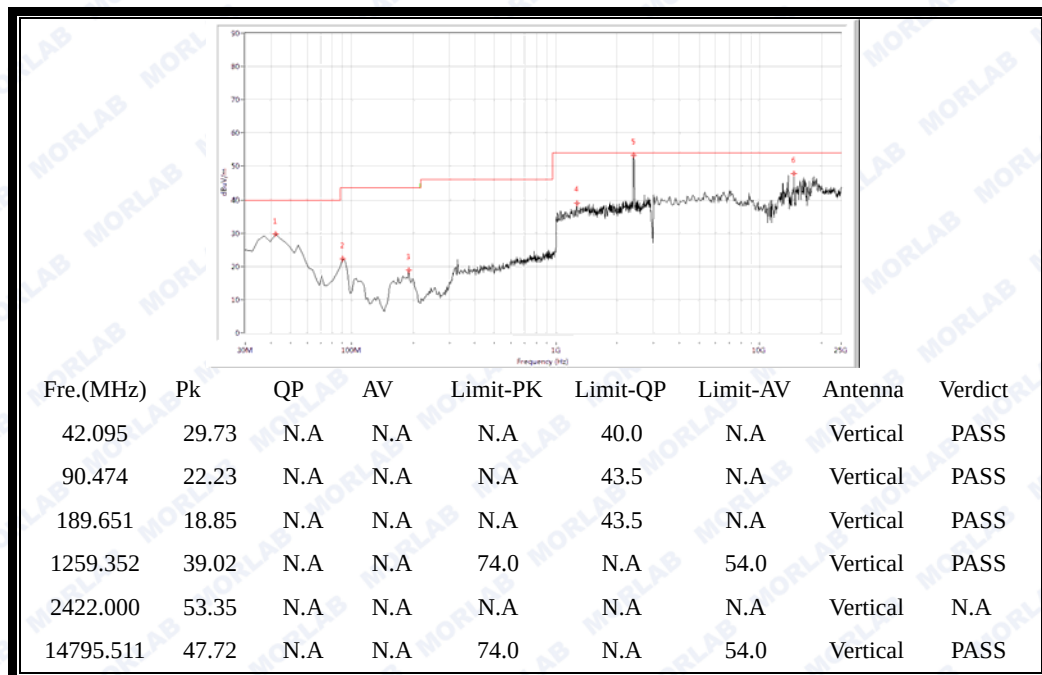
(Plot A.3: Antenna Vertical, 30MHz to 25GHz)
