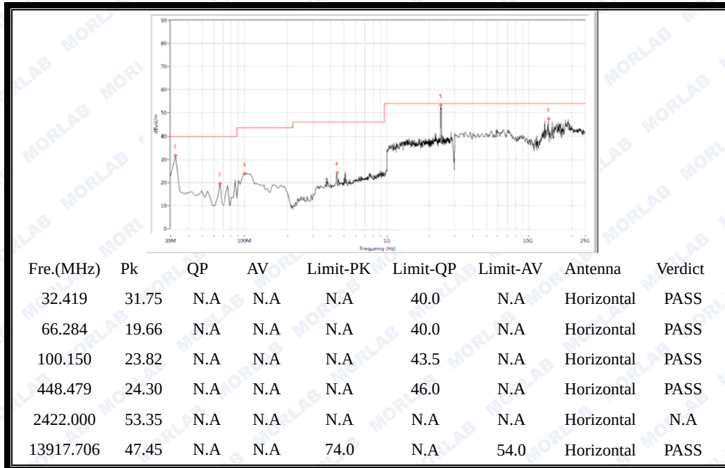
(Plot A.2: Antenna Horizontal, 30MHz to 25GHz)
