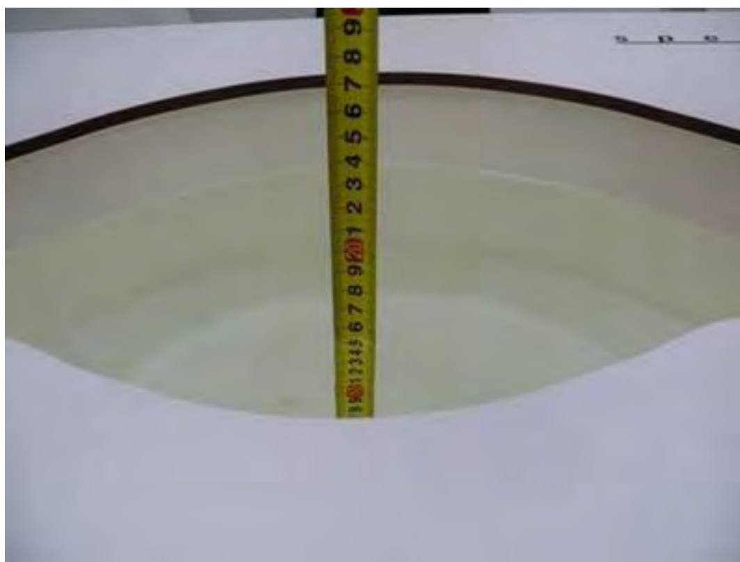
Picture 10: Liquid depth in the flat Phantom (2450 MHz, 15.3cm depth)
