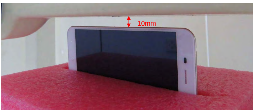
Picture 20: Left Side, the distance from handset to the bottom of the Phantom is 10mm
