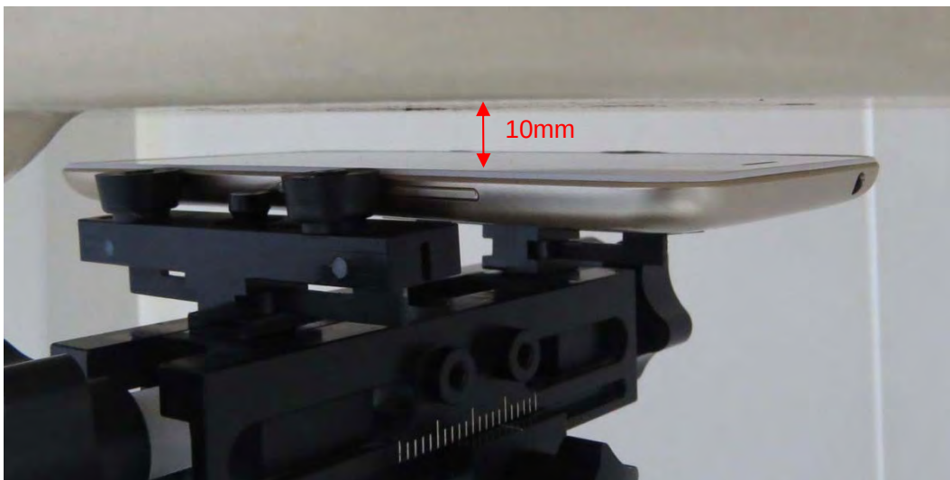
Picture 19: Front Side, the distance from handset to the bottom of the Phantom is 10mm
