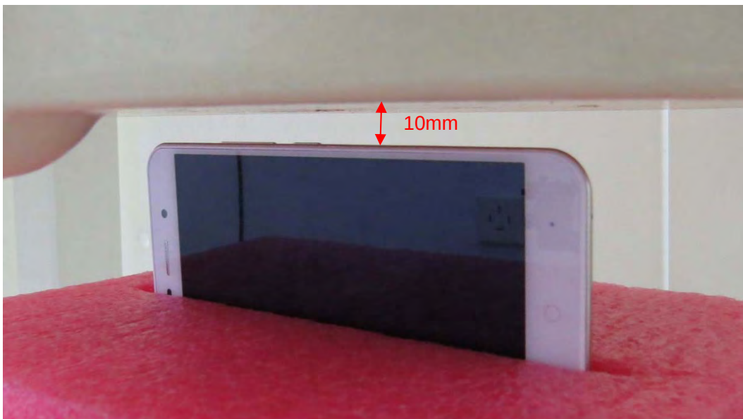
Picture 21: Right Side, the distance from handset to the bottom of the Phantom is 10mm
