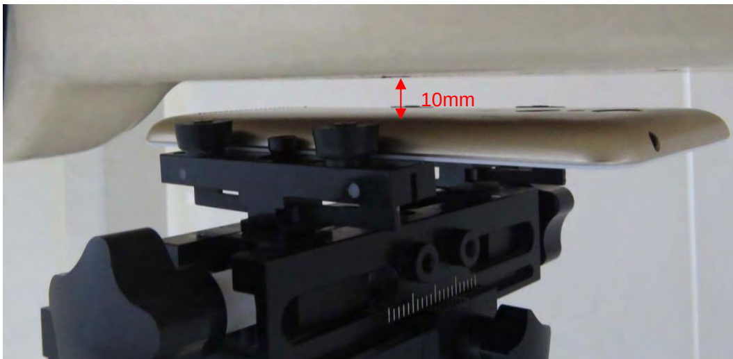
Picture 18: Back Side, the distance from handset to the bottom of the Phantom is 10mm
