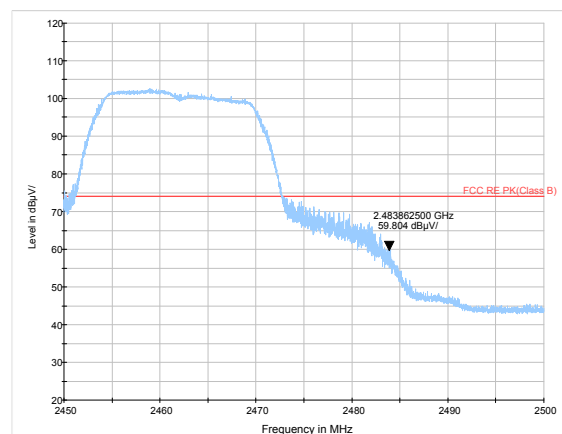
802.11g-Channel 11: Peak
