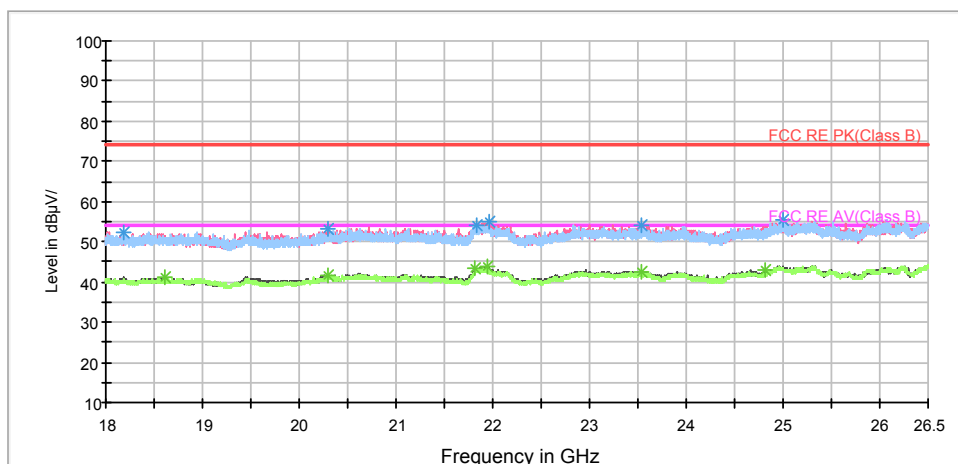
BELL_RE 18-26.5GHz PK+AV
