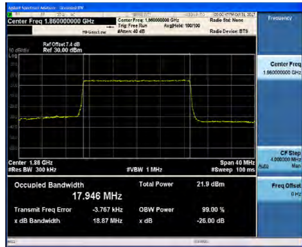
LTE Band 2 20MHz 16QAM CH-Middle
