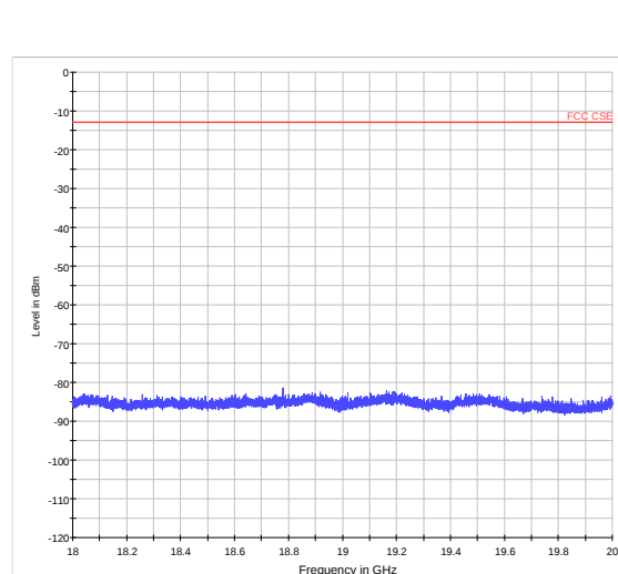
LTE Band 2 5MHz CH-Middle 18GHz~20GHz
